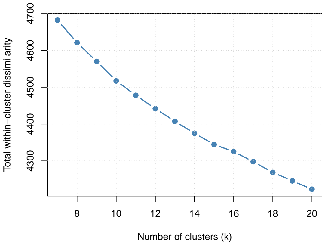
Elbow Method
