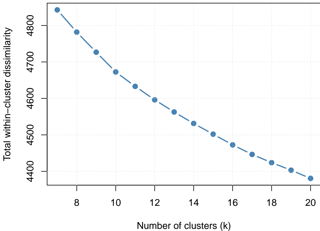
Elbow Method
