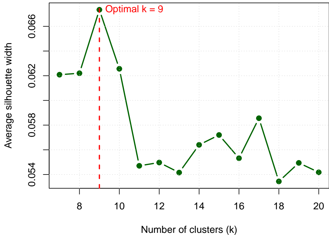
Silhouette Method
