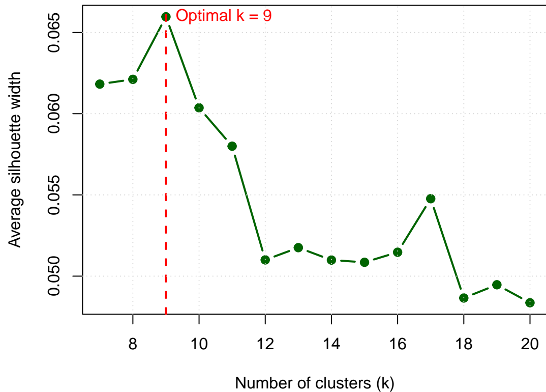
Silhouette Method
