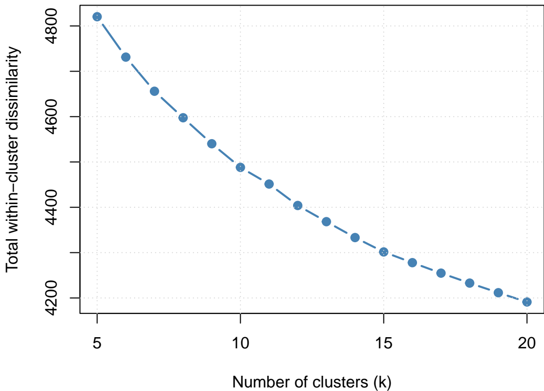
Elbow Method
