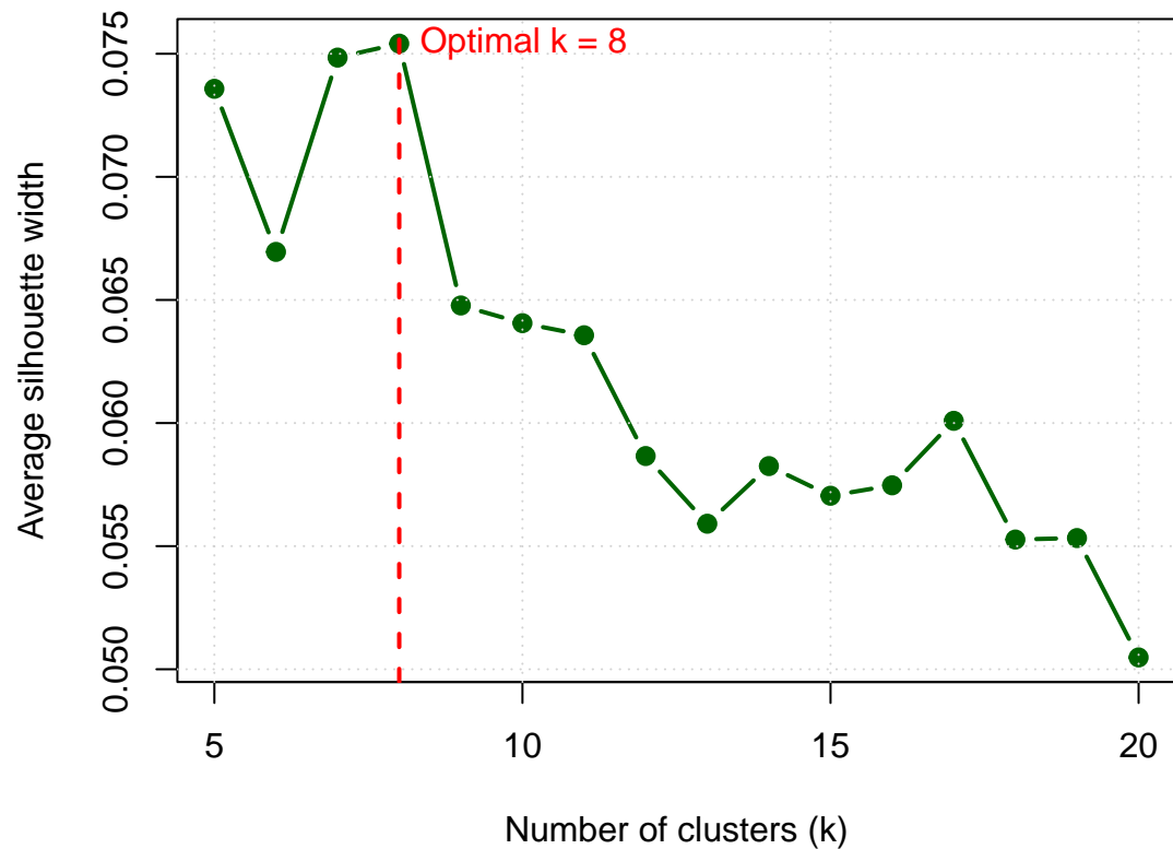
Silhouette Method
