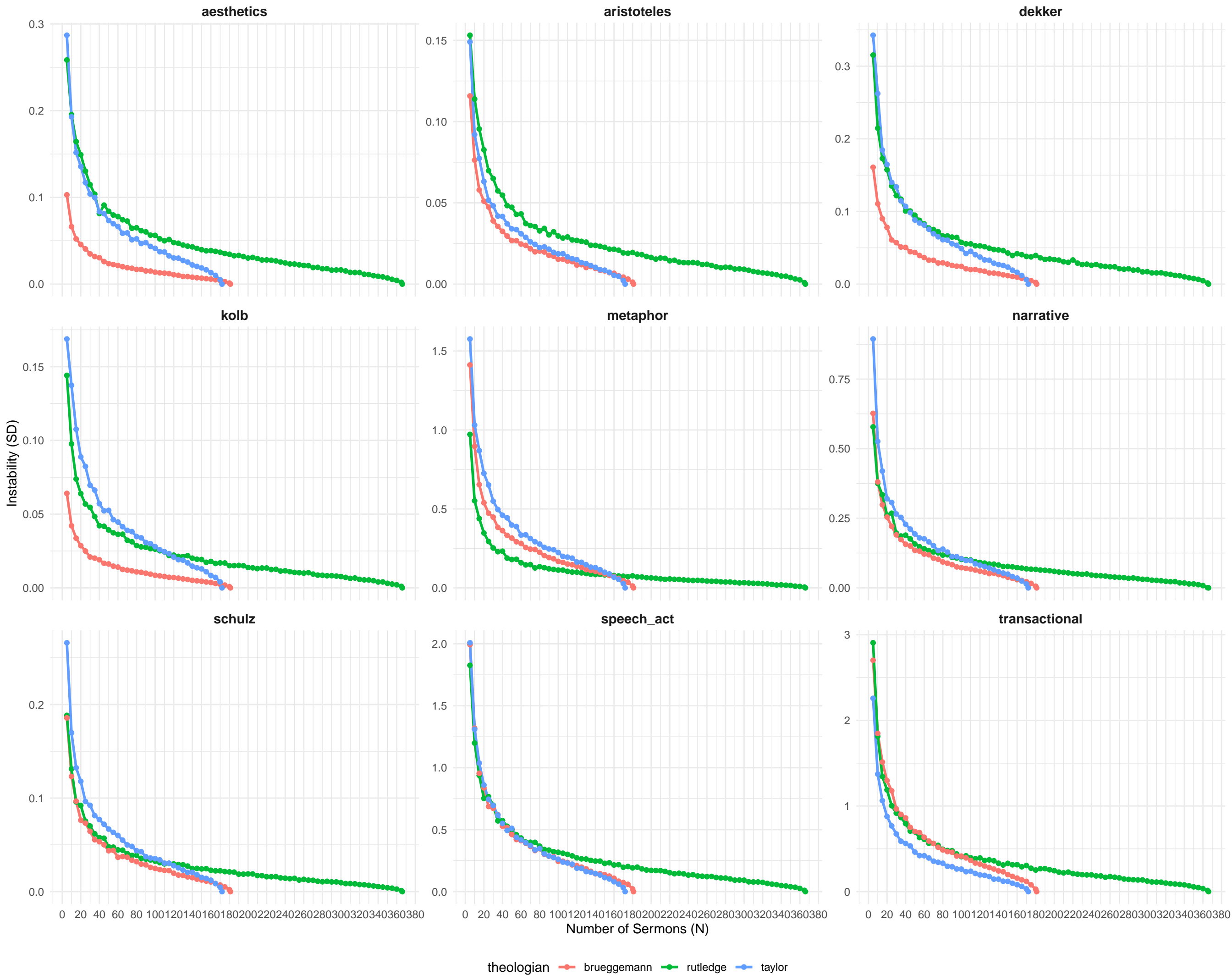
Instability of Variance Estimate (Zoomed: N \geq 5 ) Standard Deviation of the Estimator (Lower is better)
