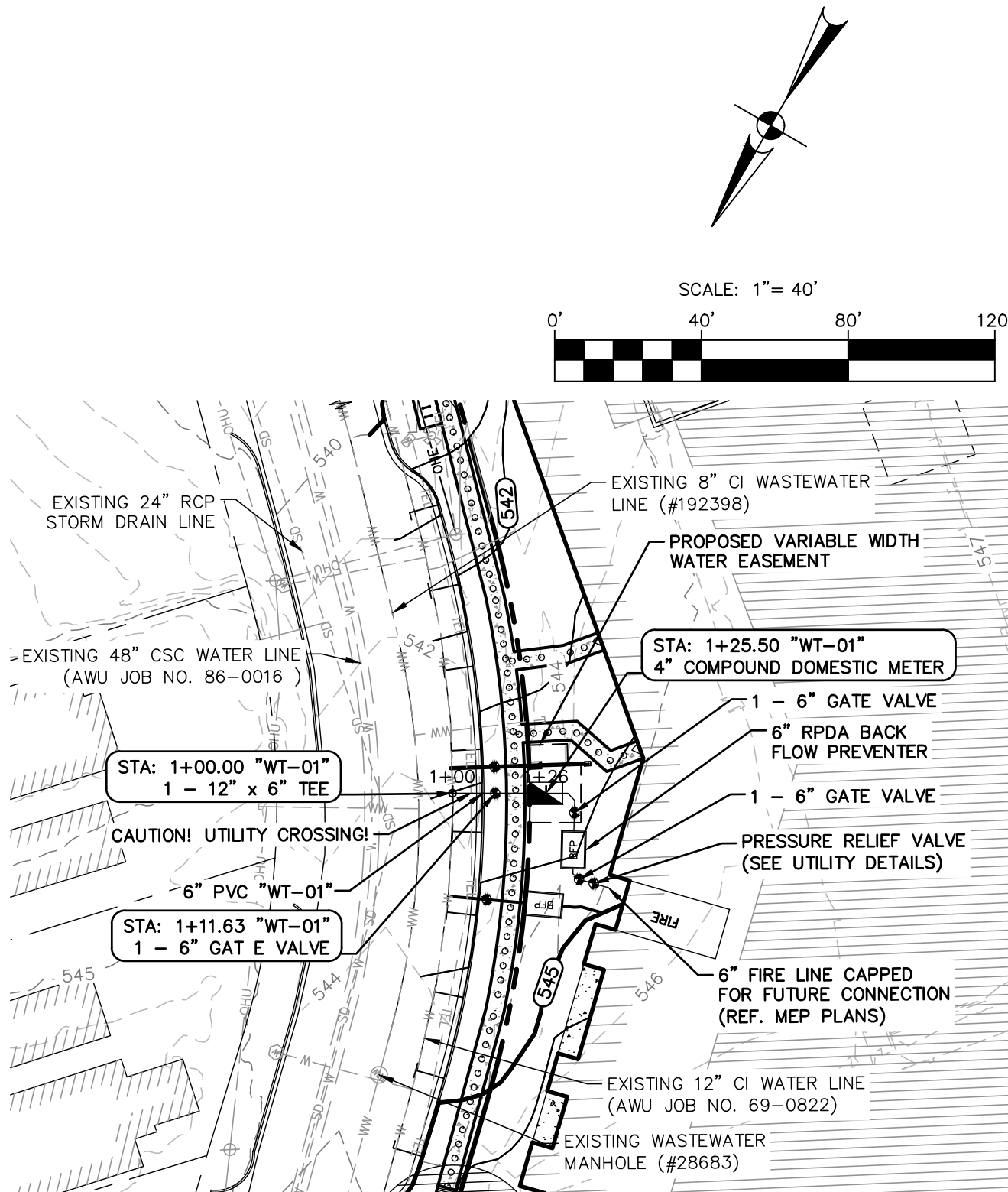
6" PVC DOMESTIC WATER - "WT-01"
