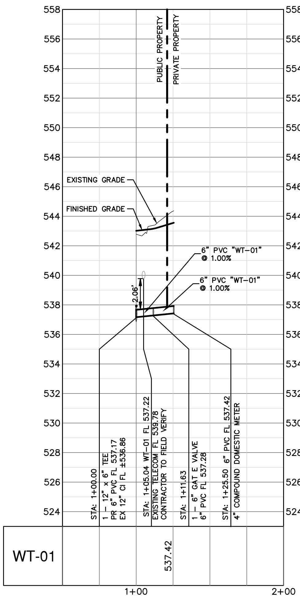
6" PVC DOMESTIC WATER - "WT-01"
