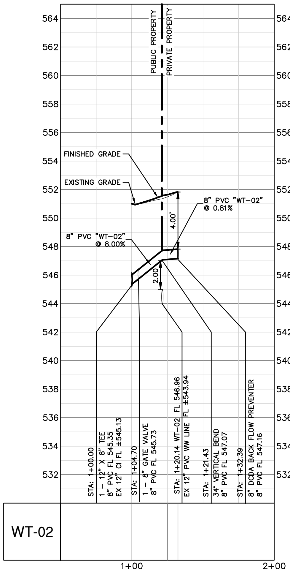
8" PVC FIRE - "WT-02"
