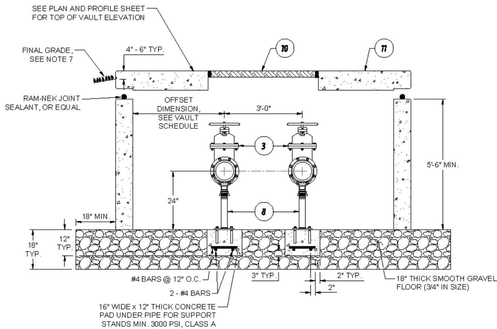
SECTION B-B VIEW
