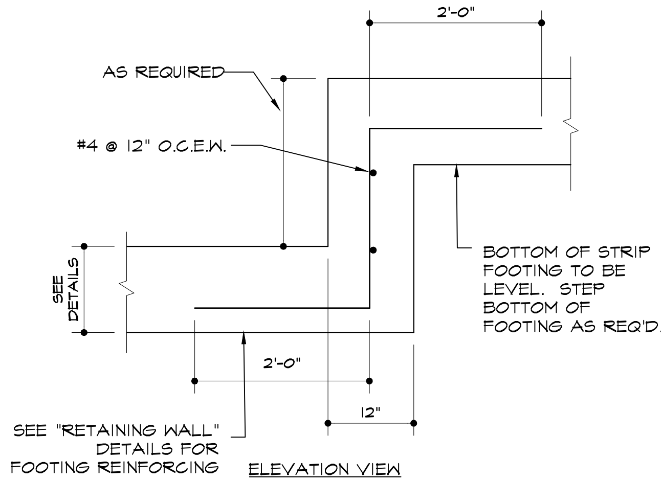
TYPICAL STEP IN FOOTING
