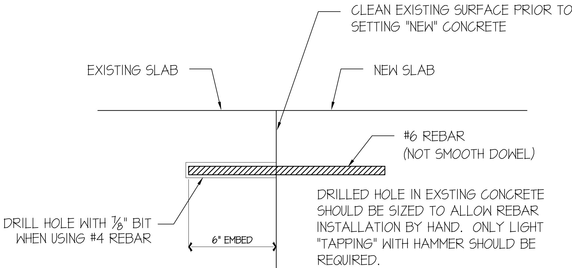
DOWEL DETAIL
