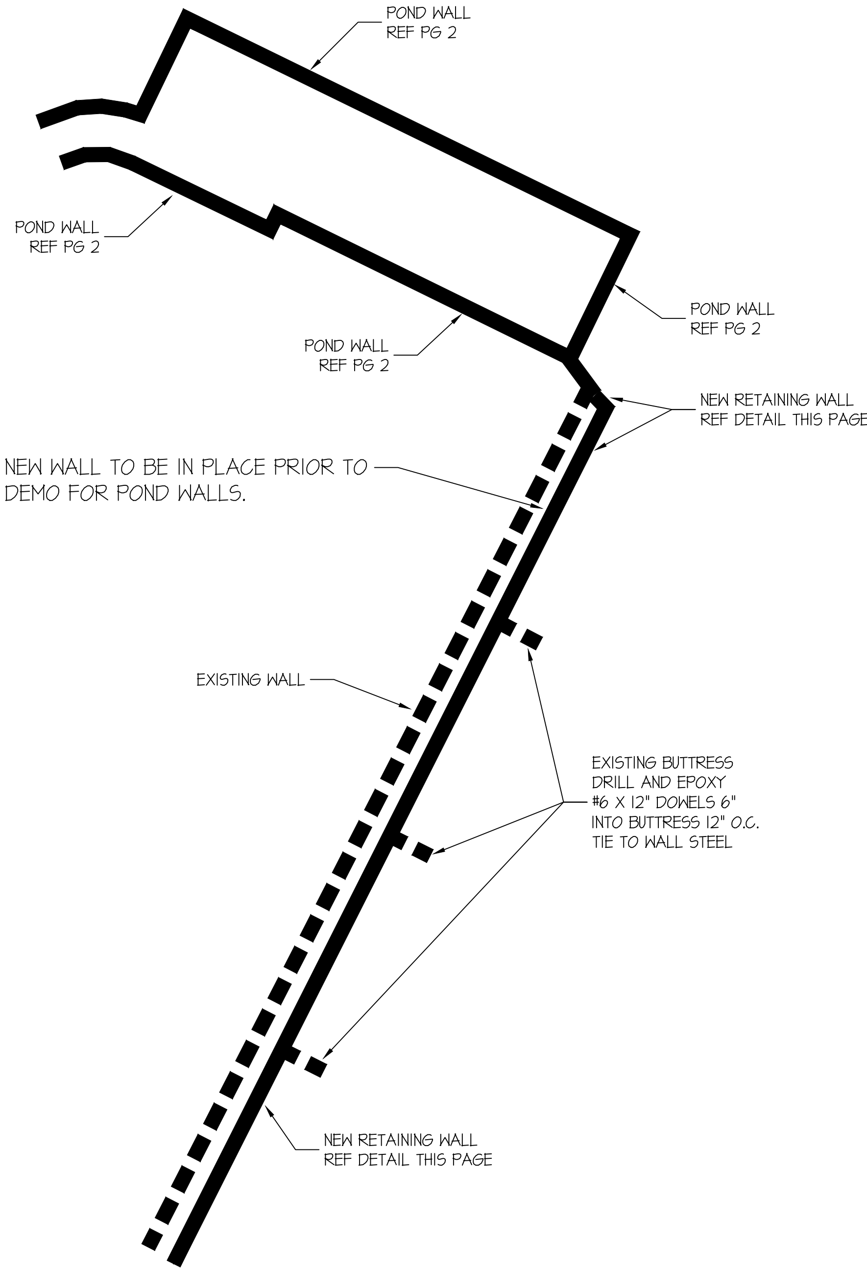
PLAN VIEW
