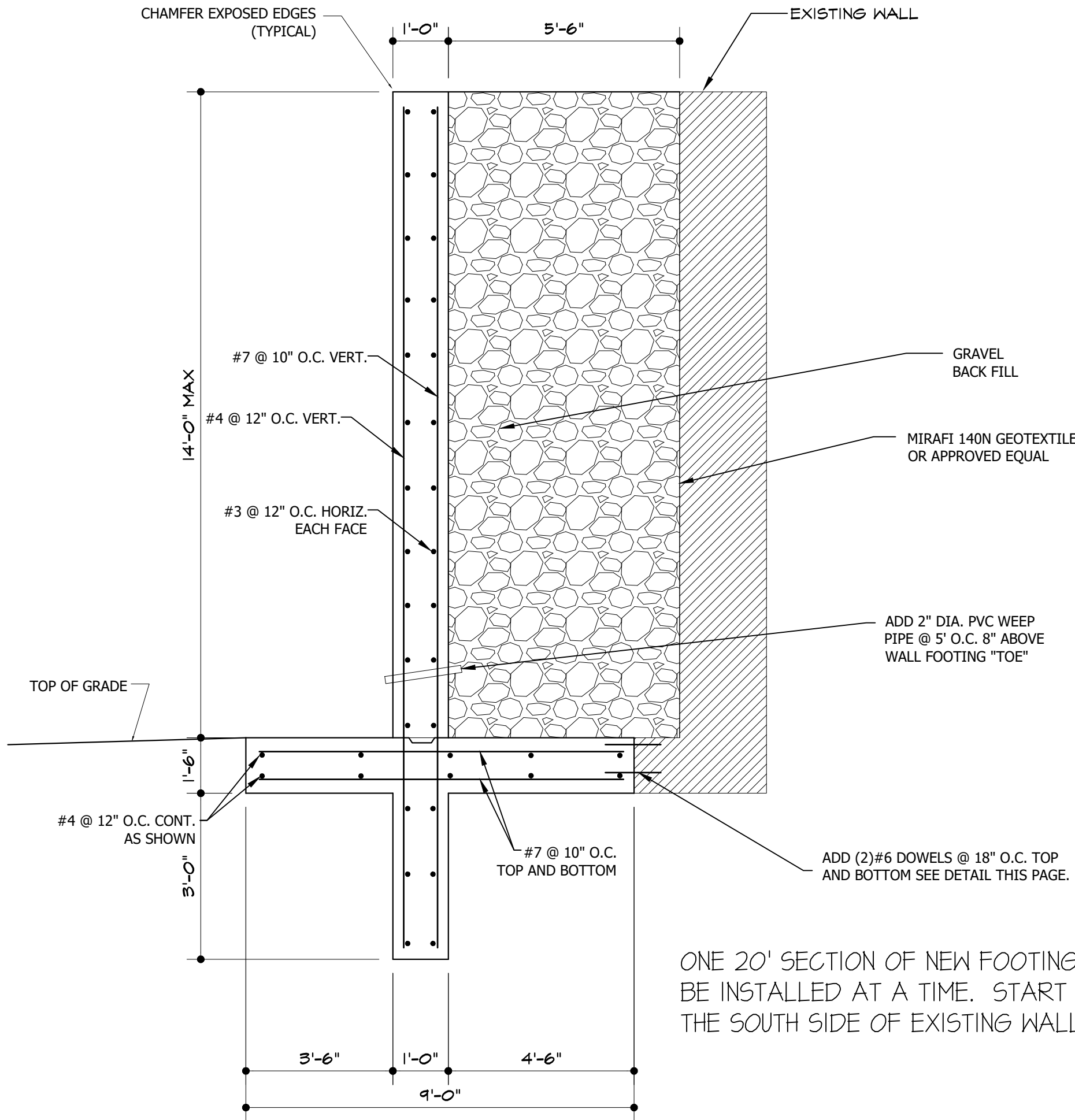
14'-0" MAX. RETAINING WALL
