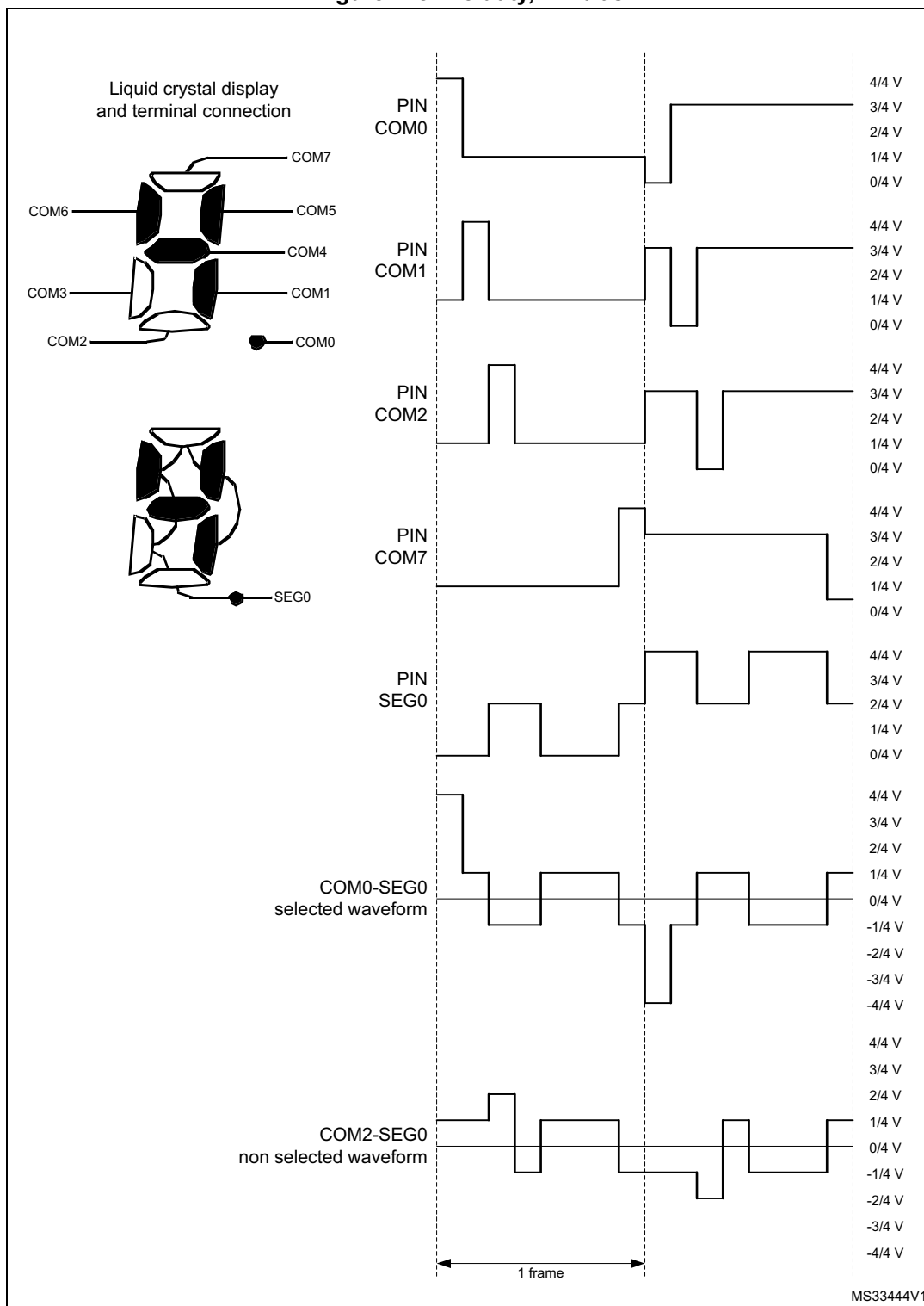
Figure 178. 1/8 duty, 1/4 bias
