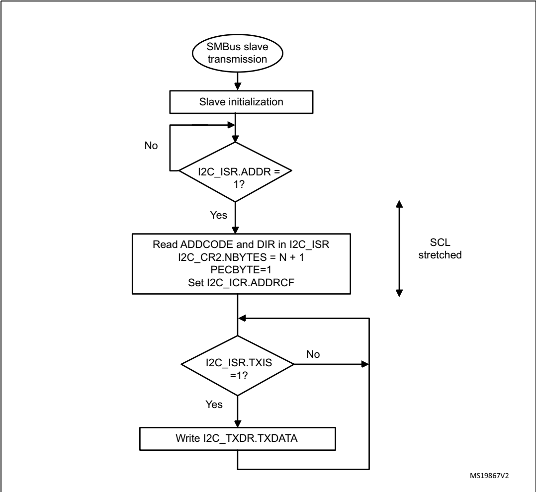
Figure 415. Transfer bus diagram for SMBus slave transmitter (SBC = 1)
