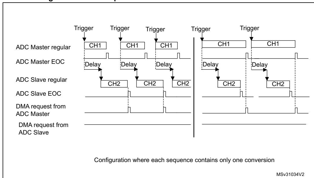
Figure 133. DMA requests in interleaved mode when MDMA = 10
