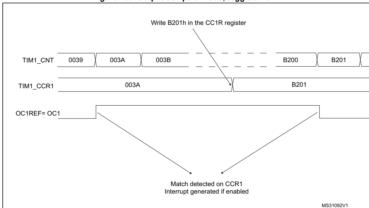
Figure 258. Output compare mode, toggle on OC1
