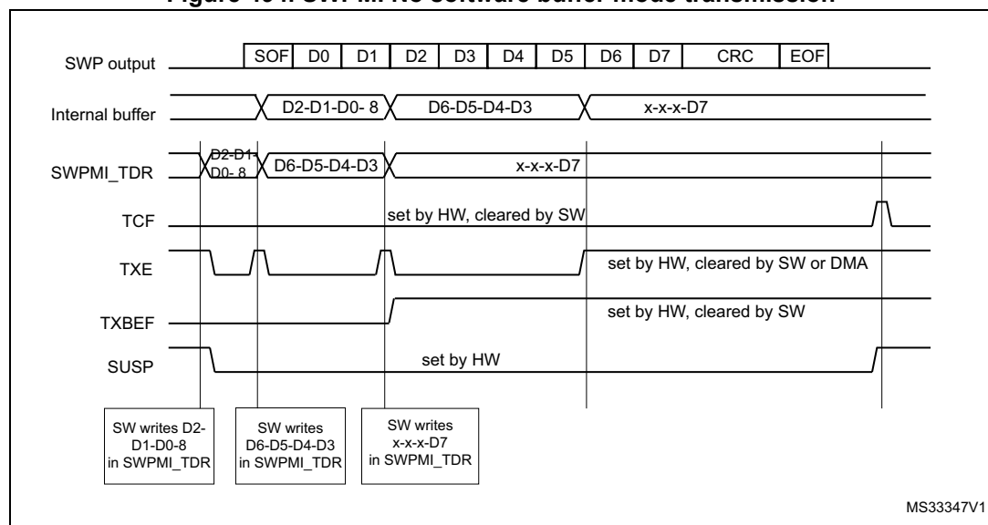
Figure 494. SWPMI No software buffer mode transmission
