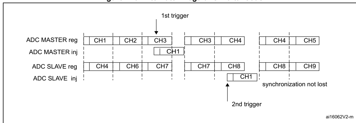
Figure 126. Alternate + regular simultaneous
