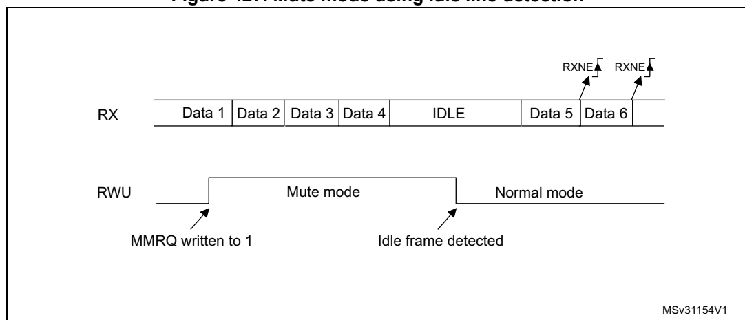
Figure 427. Mute mode using Idle line detection
