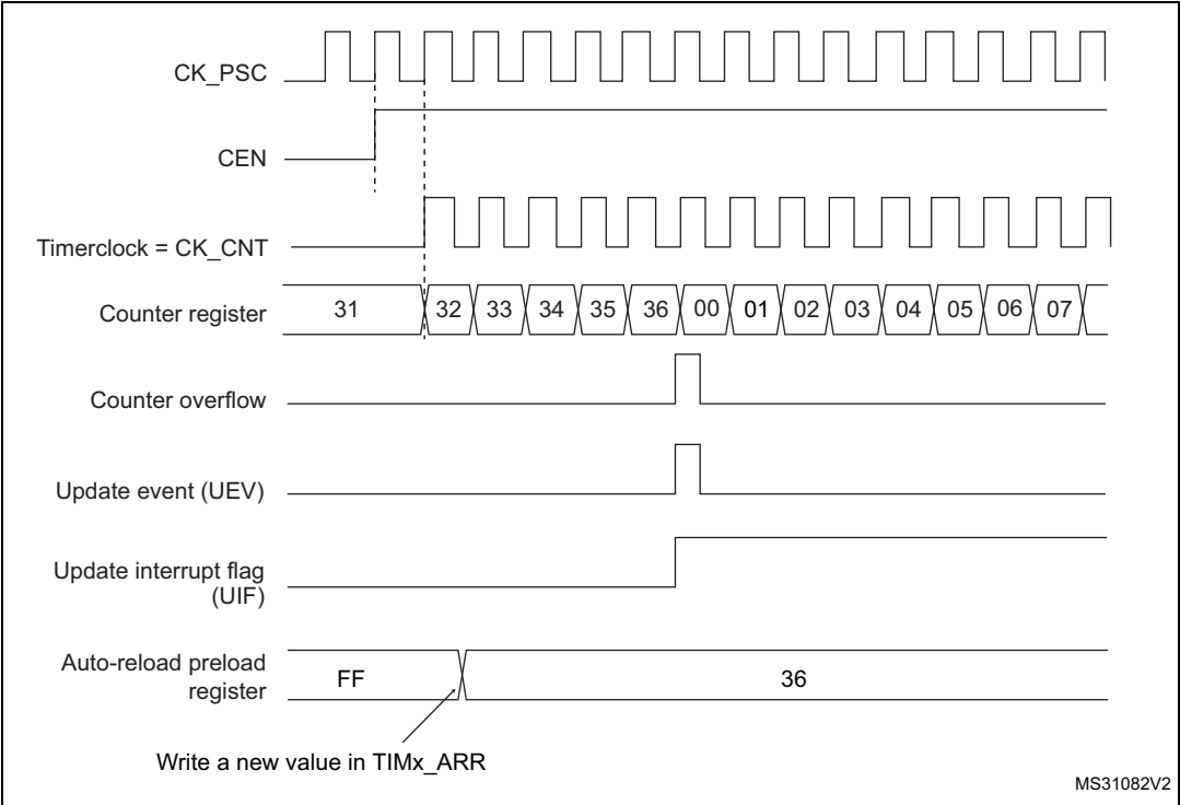
Figure 342. Counter timing diagram, update event when ARPE=0 (TIMx_ARR not preloaded)
