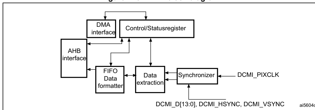
Figure 146. DCMI block diagram
