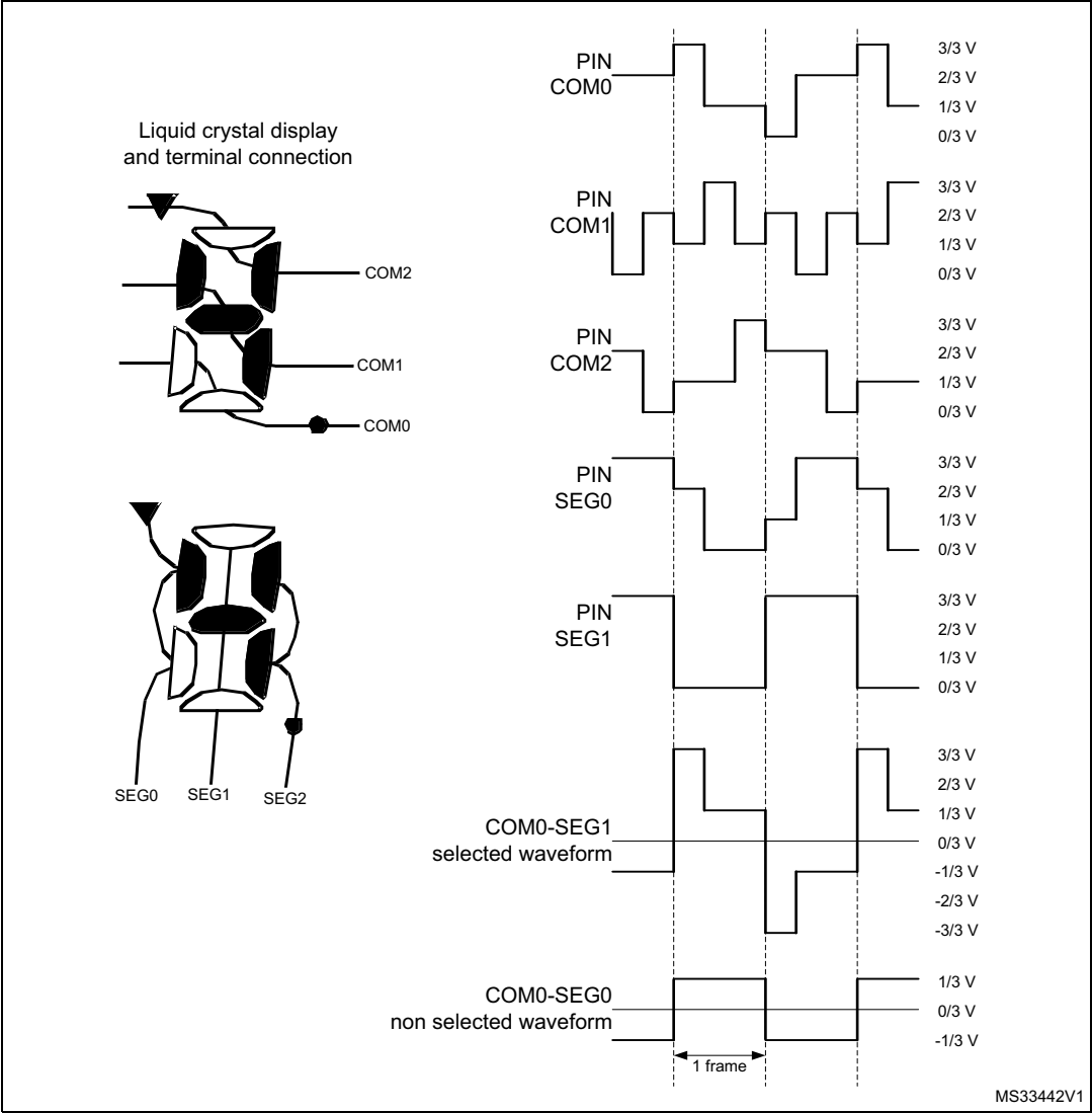
Figure 176. 1/3 duty, 1/3 bias
