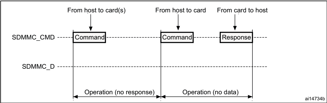
Figure 501. “No response” and “no data” operations
