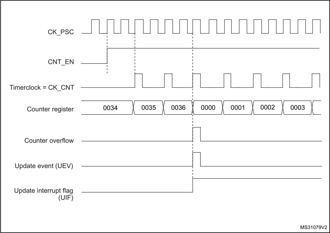
Figure 288. Counter timing diagram, internal clock divided by 2
