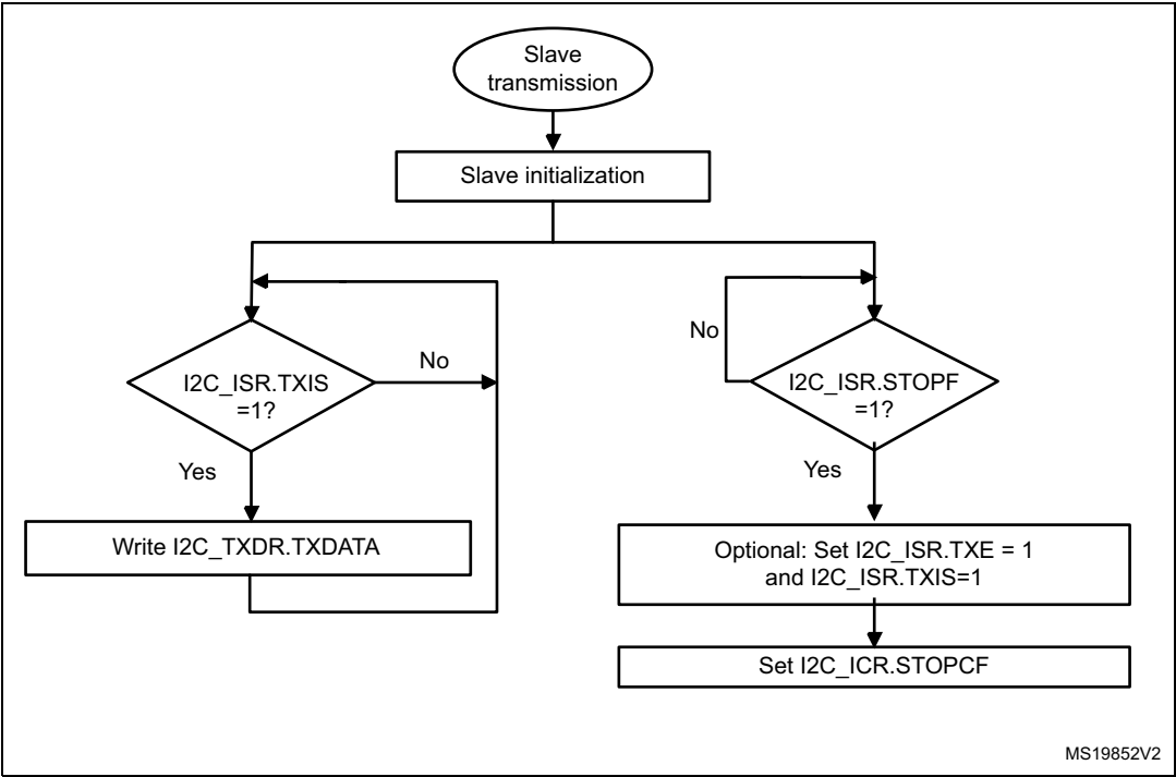
Figure 398. Transfer sequence flow for I2C slave transmitter, NOSTRETCH = 1
