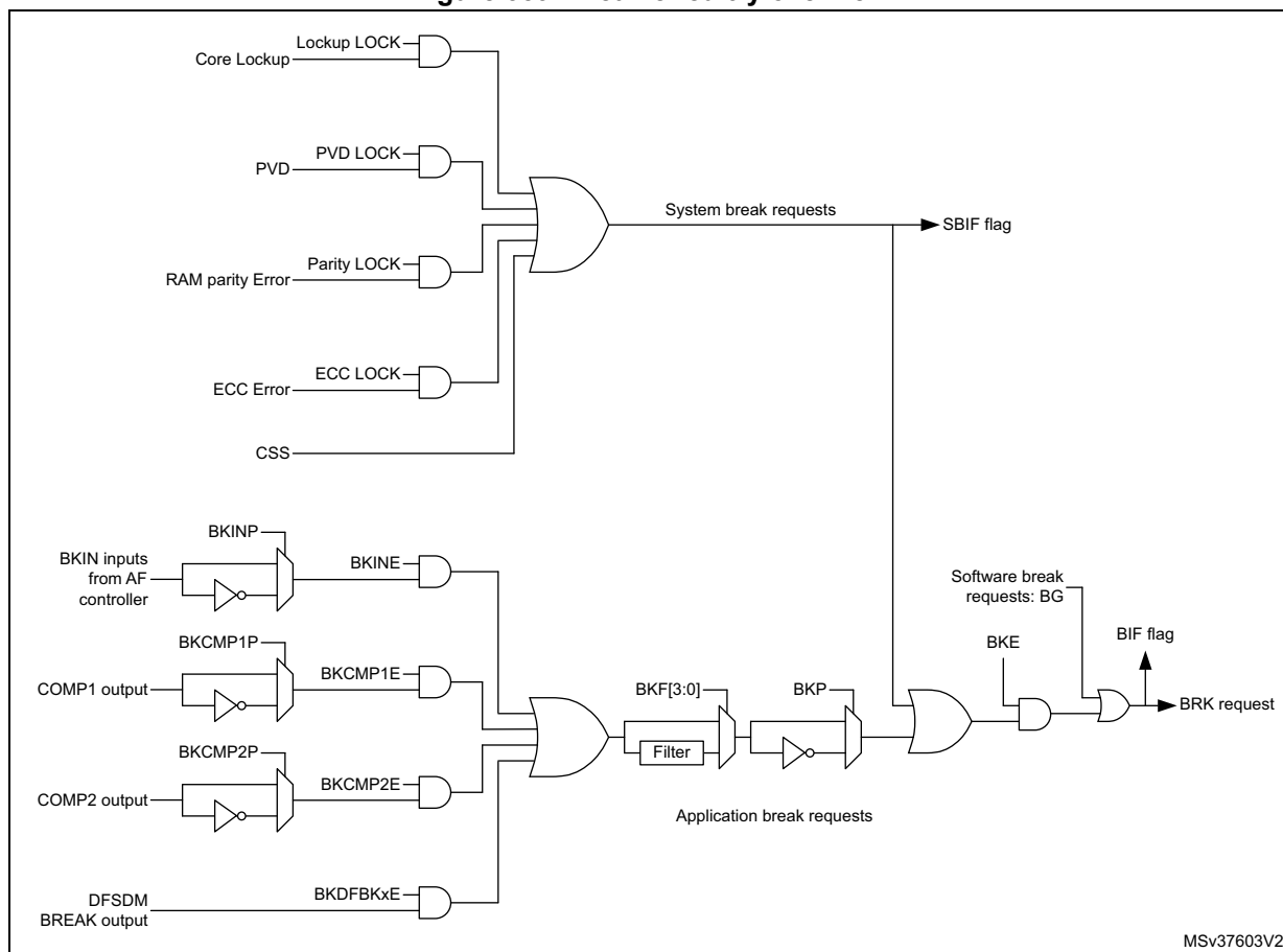
Figure 359. Break circuitry overview
