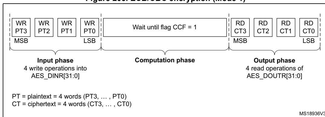
Figure 205. ECB/CBC encryption (Mode 1)
