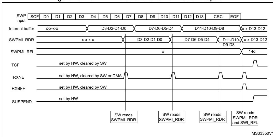
Figure 497. SWPMI No software buffer mode reception
