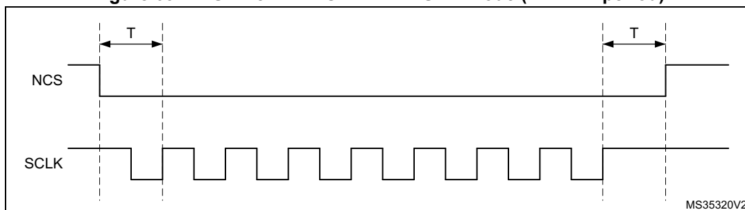
Figure 63. NCS when CKMODE = 1 in SDR mode ( T = \text{CLK period} )
