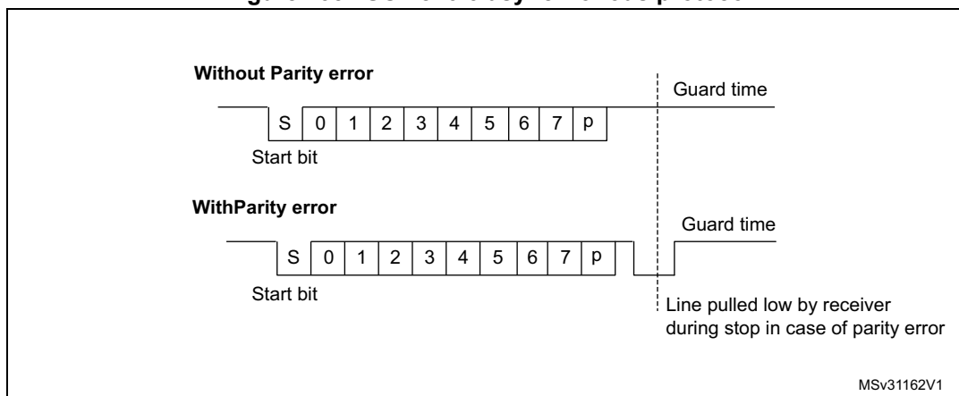
Figure 435. ISO 7816-3 asynchronous protocol
