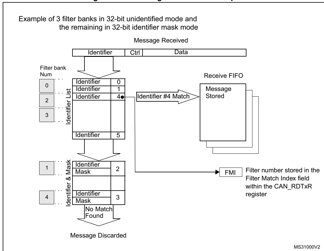
Figure 526. Filtering mechanism example
