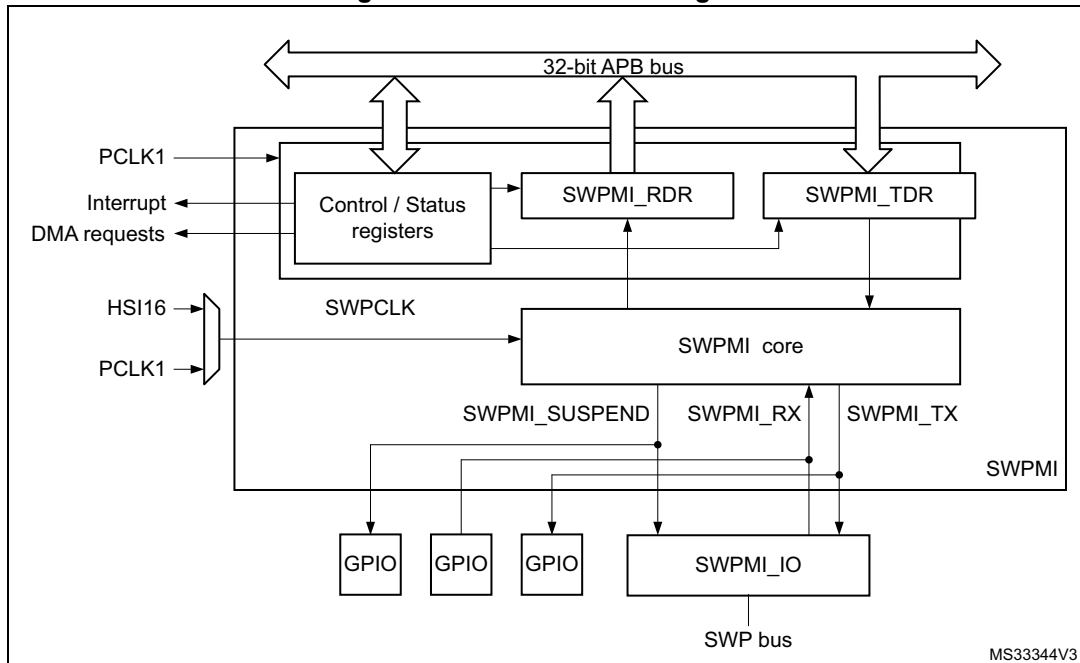
Figure 491. SWPMI block diagram
