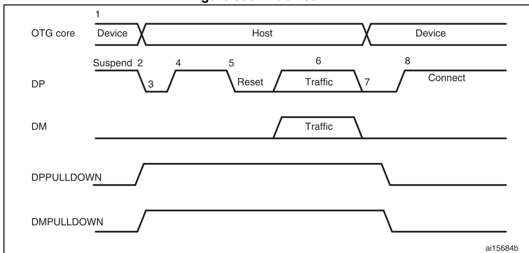
Figure 556. B-device HNP
