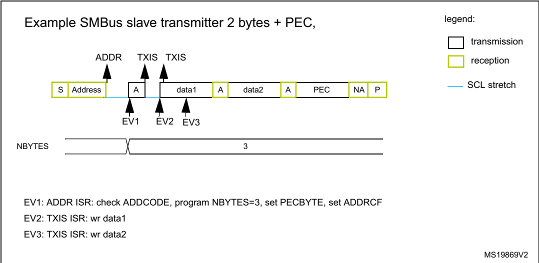
Figure 415. Transfer bus diagram for SMBus slave transmitter (SBC = 1)
