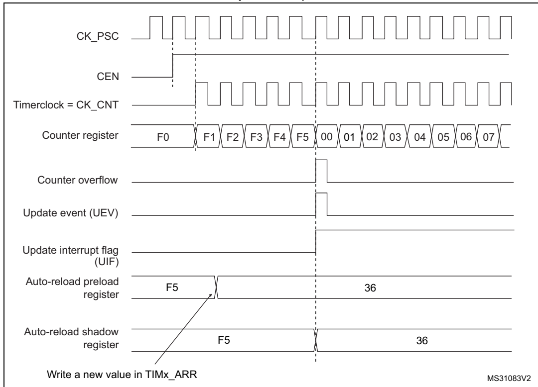
Figure 292. Counter timing diagram, Update event when ARPE=1 (TIMx_ARR preloaded)
