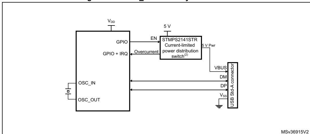
Figure 535. OTG_FS host-only connection
