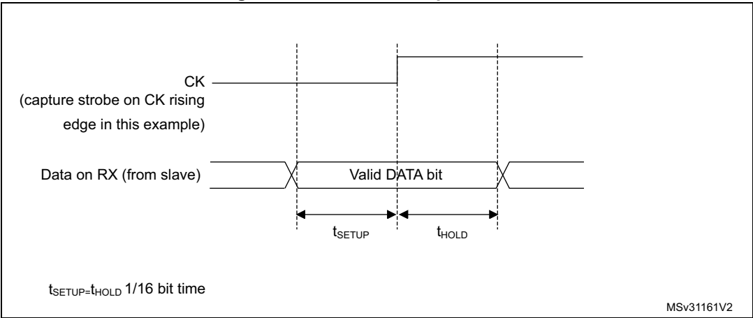
Figure 434. RX data setup/hold time
