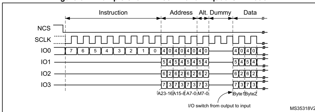
Figure 61. Example of a DDR command in quad-SPI mode
