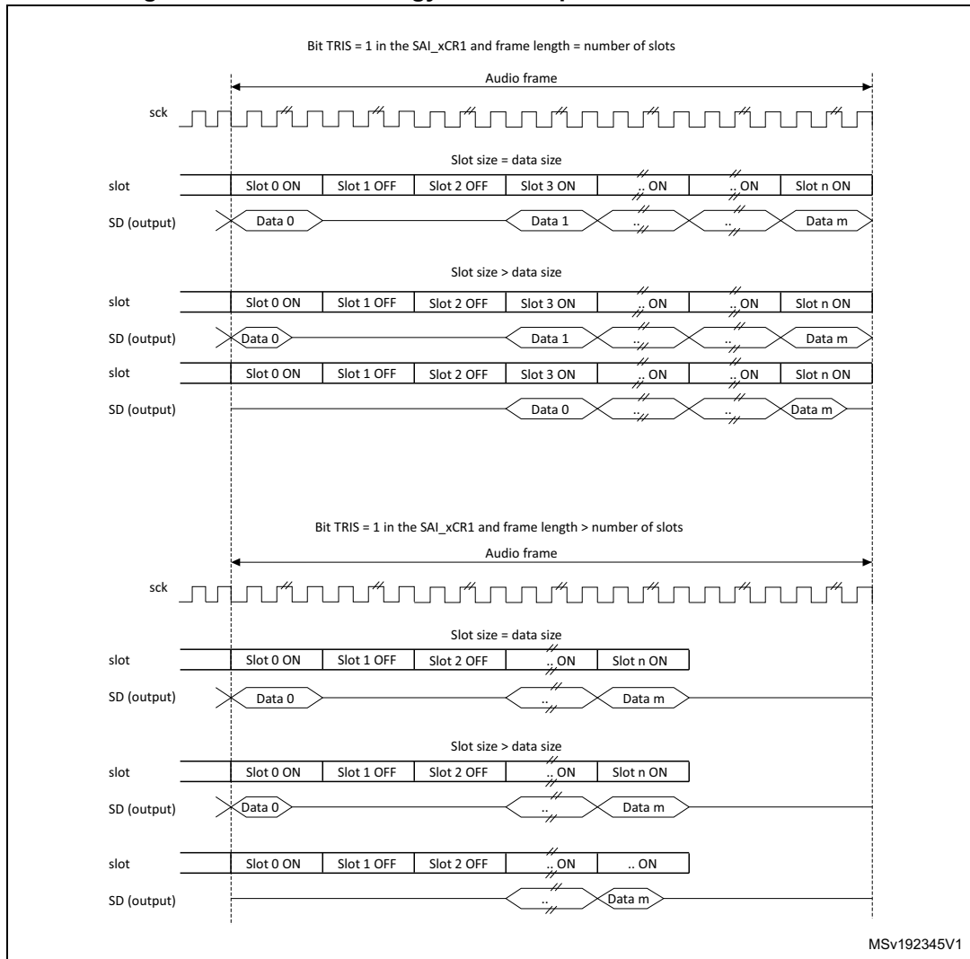
Figure 485. Tristate strategy on SD output line on an inactive slot
