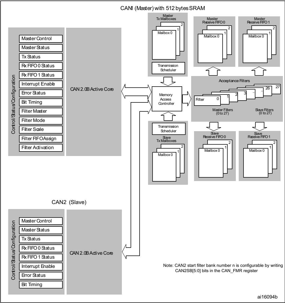
Figure 516. Dual-CAN block diagram
