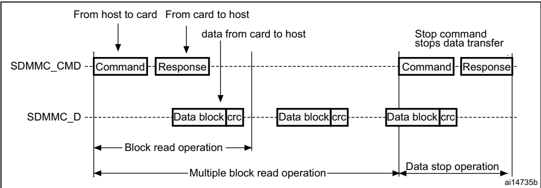
Figure 502. (Multiple) block read operation
