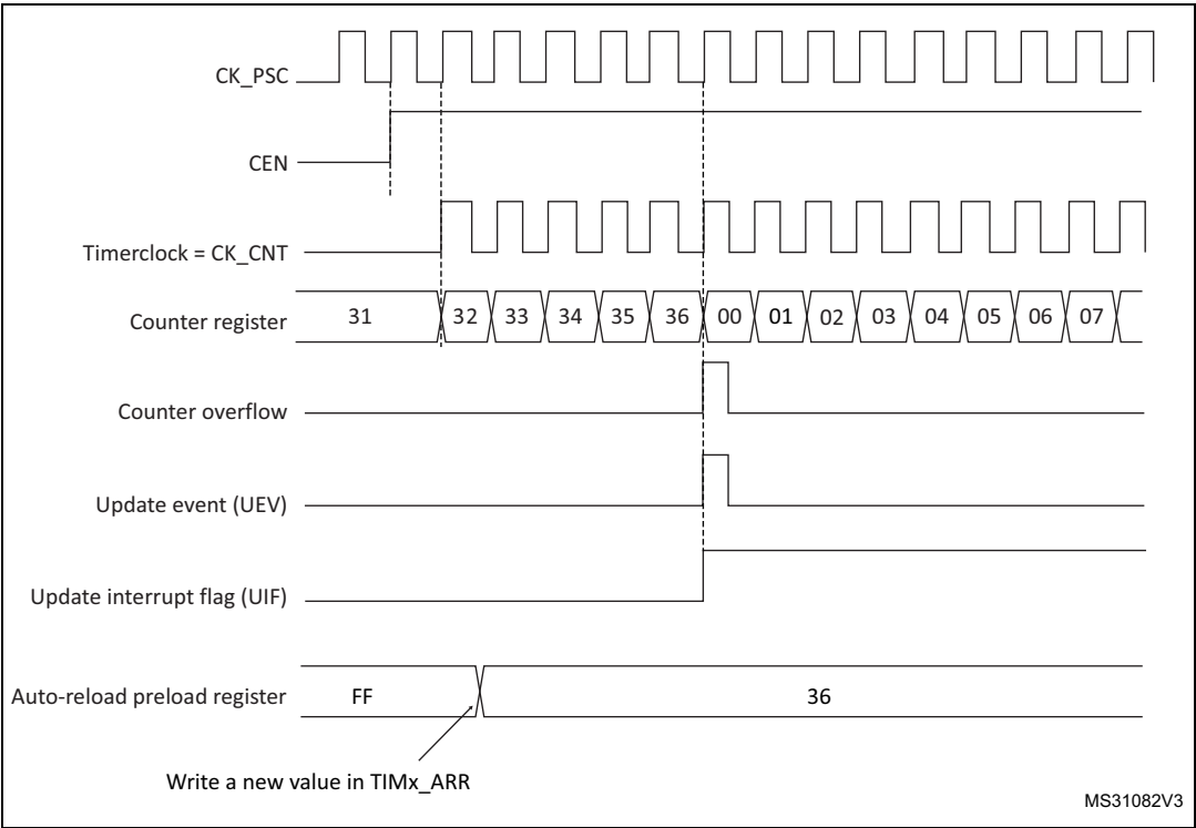
Figure 230. Counter timing diagram, update event when ARPE=0 (TIMx_ARR not preloaded)
