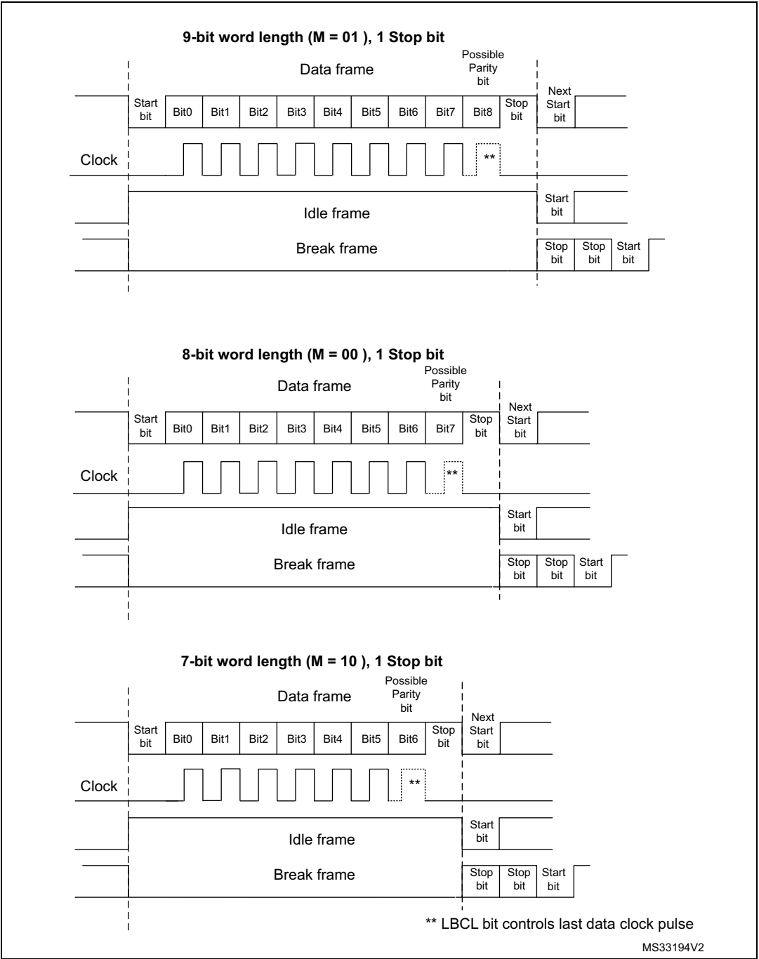
Figure 446. Word length programming
