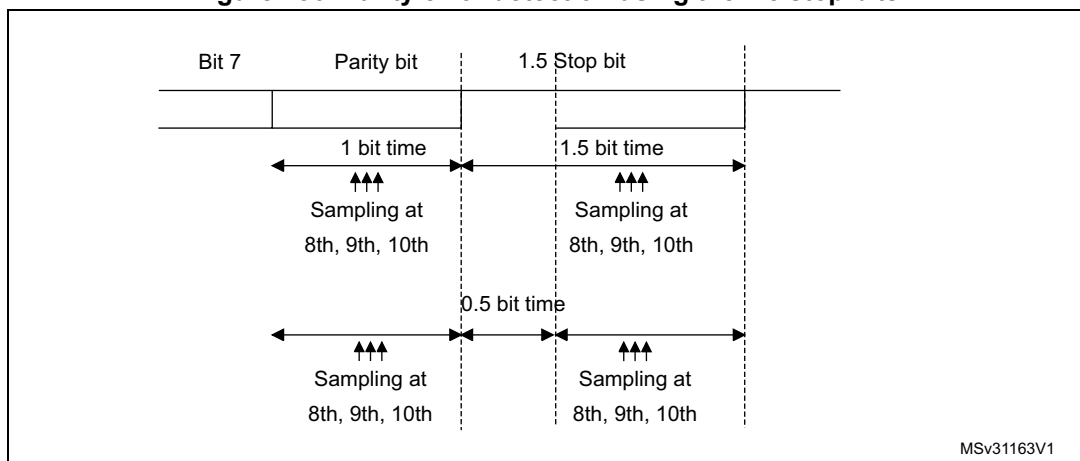
Figure 436. Parity error detection using the 1.5 stop bits
