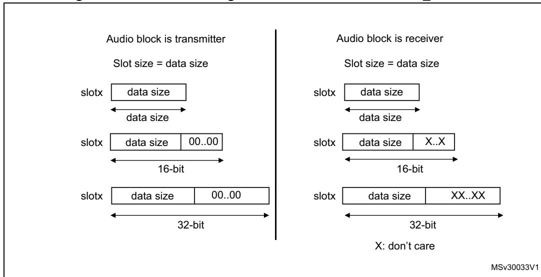
Figure 477. Slot size configuration with FBOFF = 0 in SAI_xSLOTR
