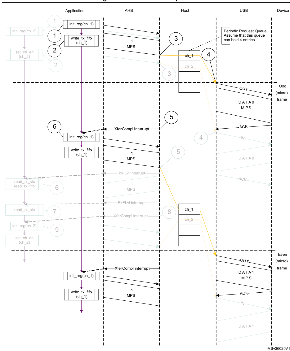
Figure 545. Normal interrupt OUT
