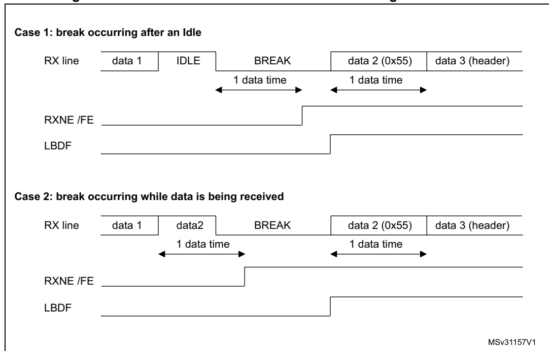
Figure 430. Break detection in LIN mode vs. Framing error detection
