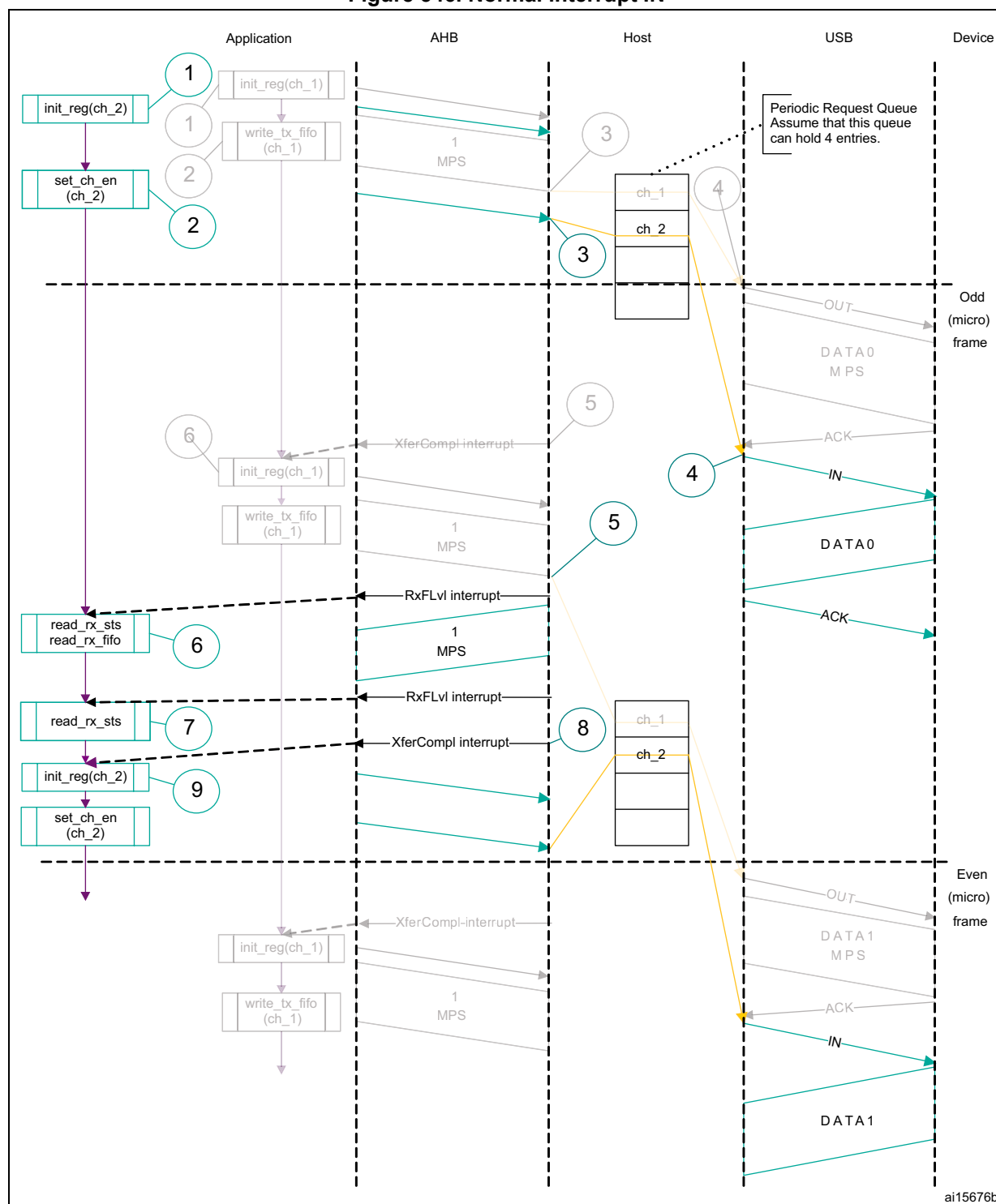
Figure 546. Normal interrupt IN
