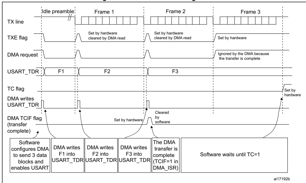
Figure 439. Transmission using DMA
