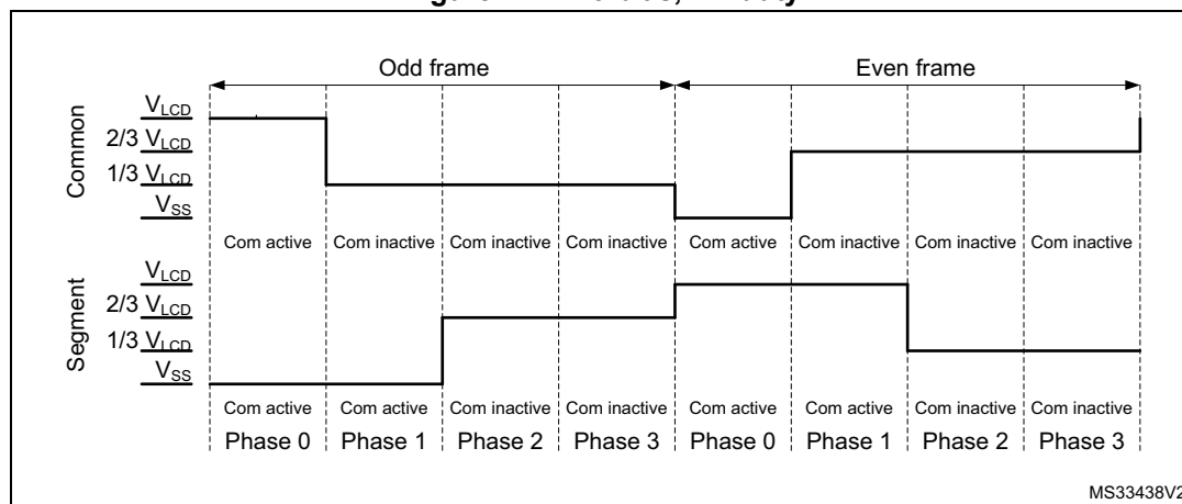
Figure 172. 1/3 bias, 1/4 duty
