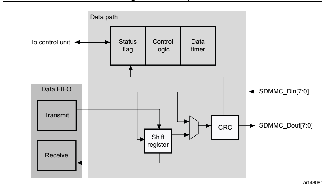
Figure 513. Data path
