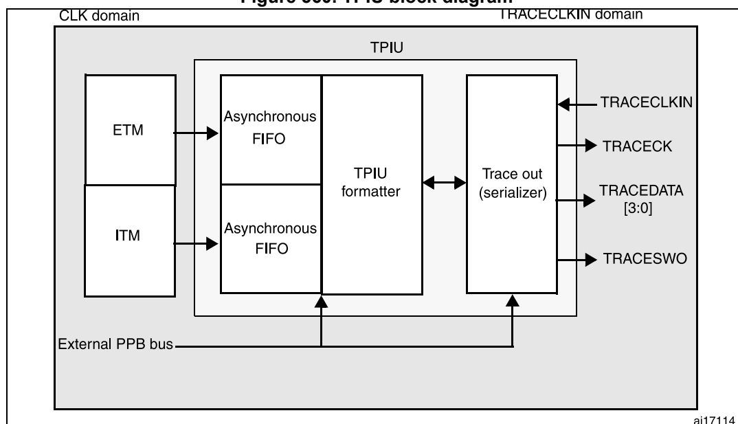
Figure 560. TPIU block diagram
