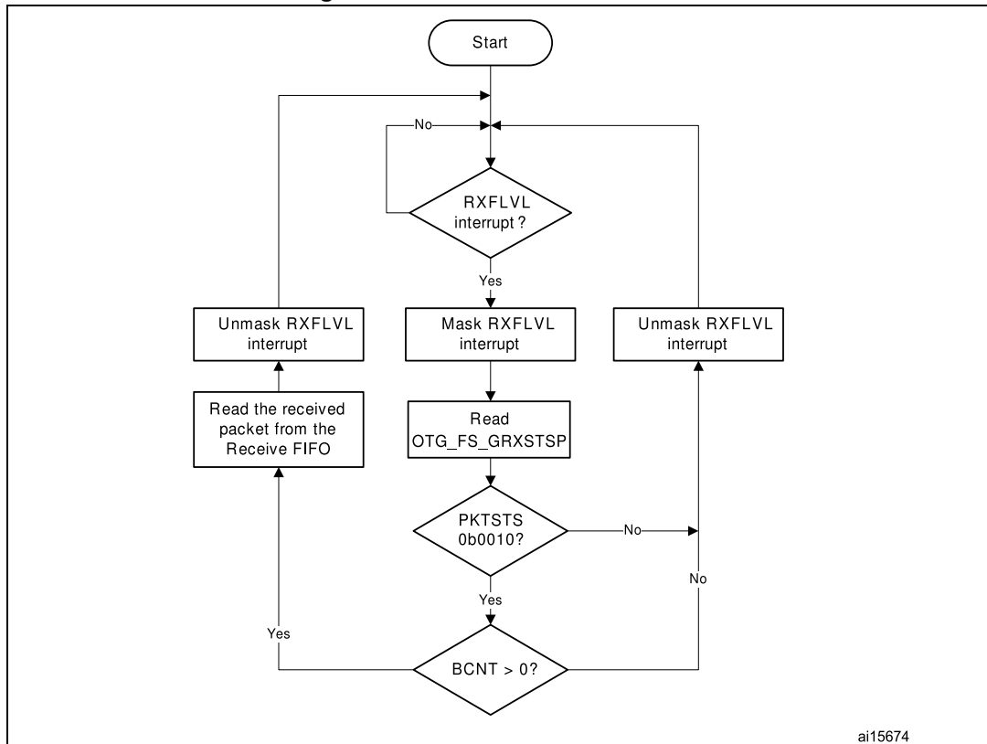
Figure 542. Receive FIFO read task
