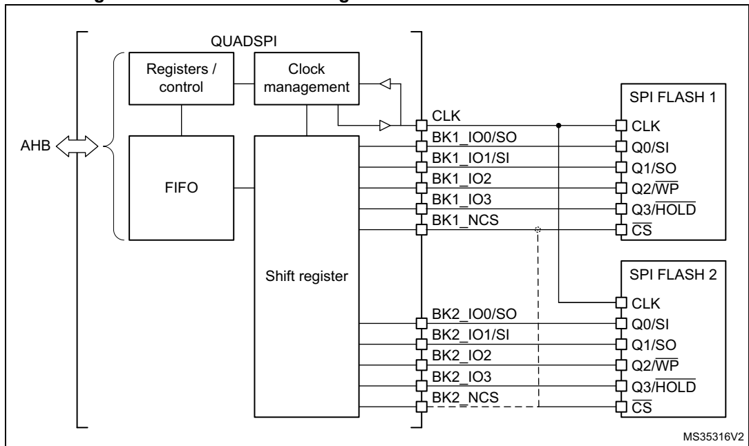
Figure 59. QUADSPI block diagram when dual-flash mode is enabled
