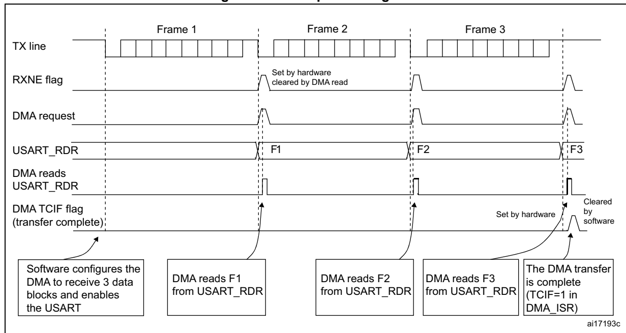
Figure 440. Reception using DMA
