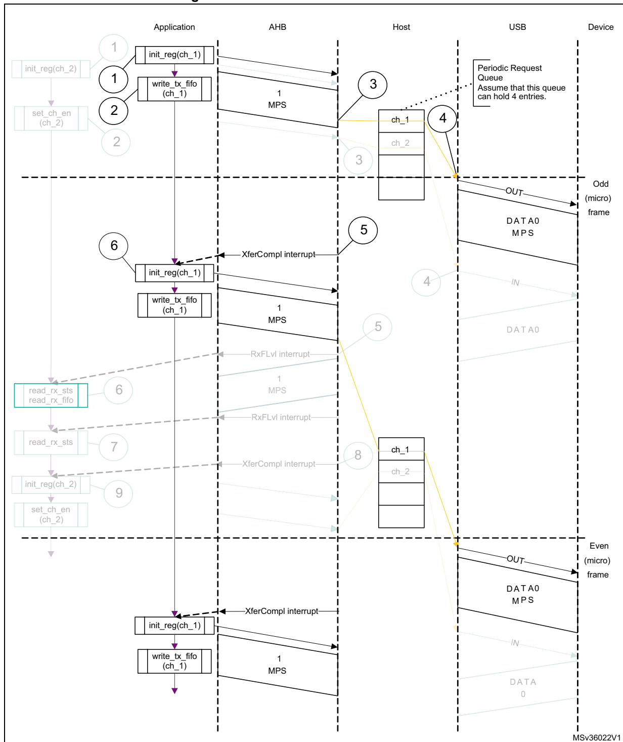
Figure 547. Isochronous OUT transactions
