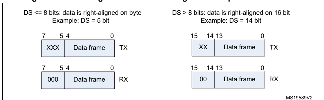
Figure 465. Data alignment when data length is not equal to 8-bit or 16-bit
