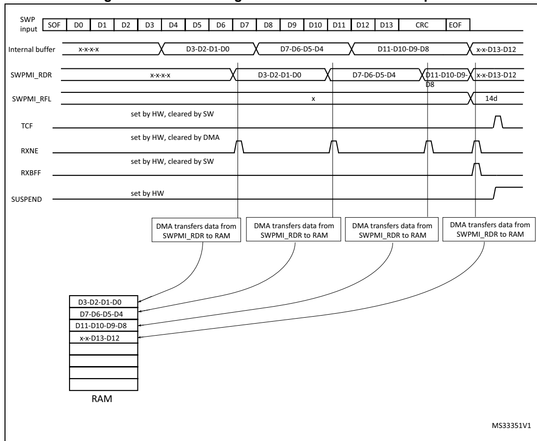
Figure 498. SWPMI single software buffer mode reception
