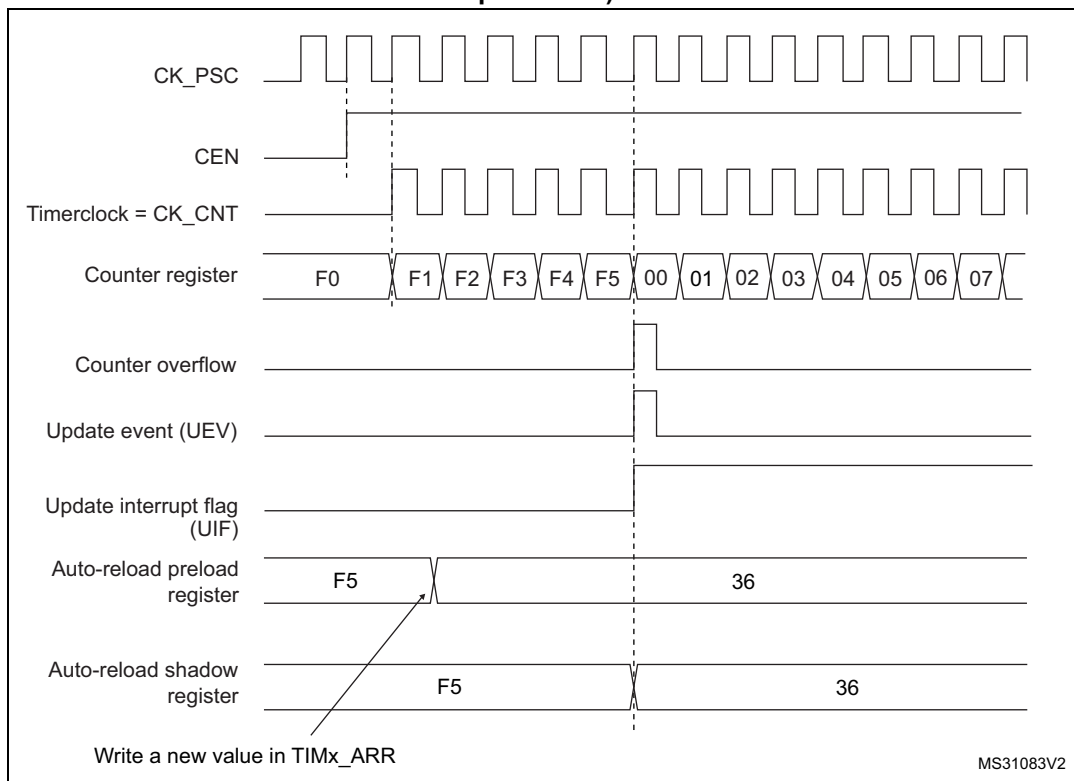
Figure 376. Counter timing diagram, update event when ARPE=1 (TIMx_ARR preloaded)
