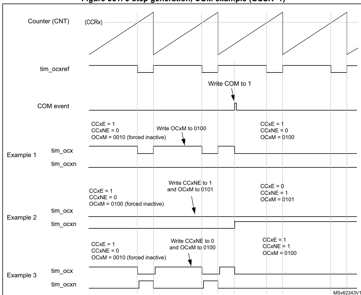
Figure 361. 6-step generation, COM example (OSSR=1)
