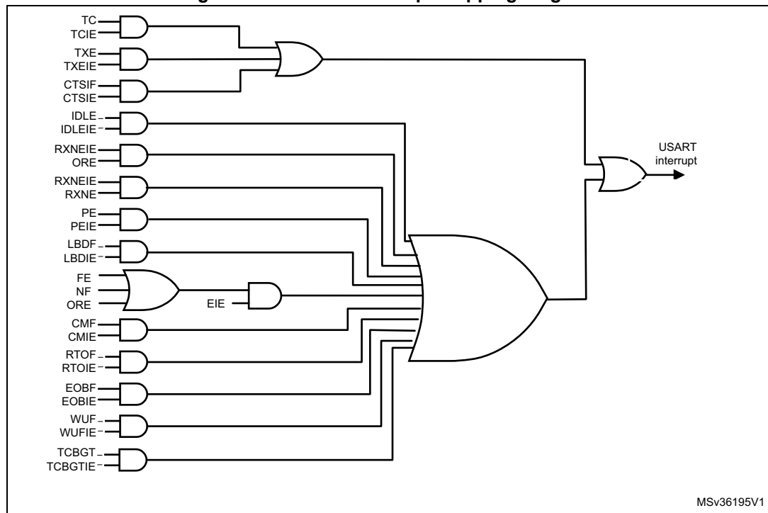
Figure 444. USART interrupt mapping diagram
