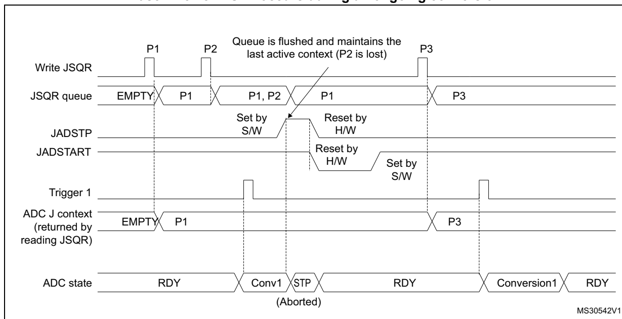
Figure 86. Flushing JSQR queue of context by setting JADSTP = 1 (JQM = 0) Case when JADSTP occurs during an ongoing conversion
