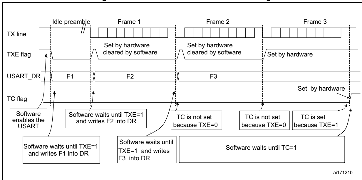
Figure 423. TC/TXE behavior when transmitting
