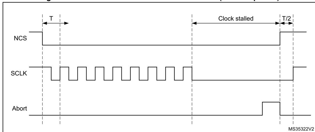
Figure 65. NCS when CKMODE = 1 with an abort (T = CLK period)
