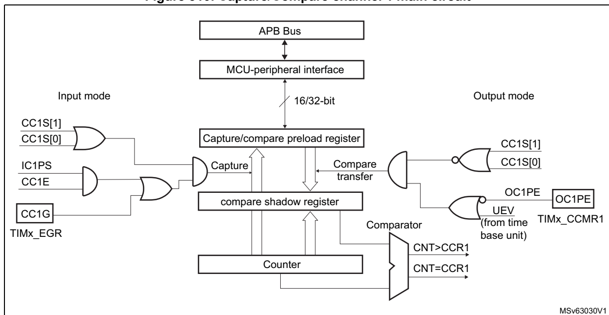
Figure 310. Capture/Compare channel 1 main circuit
