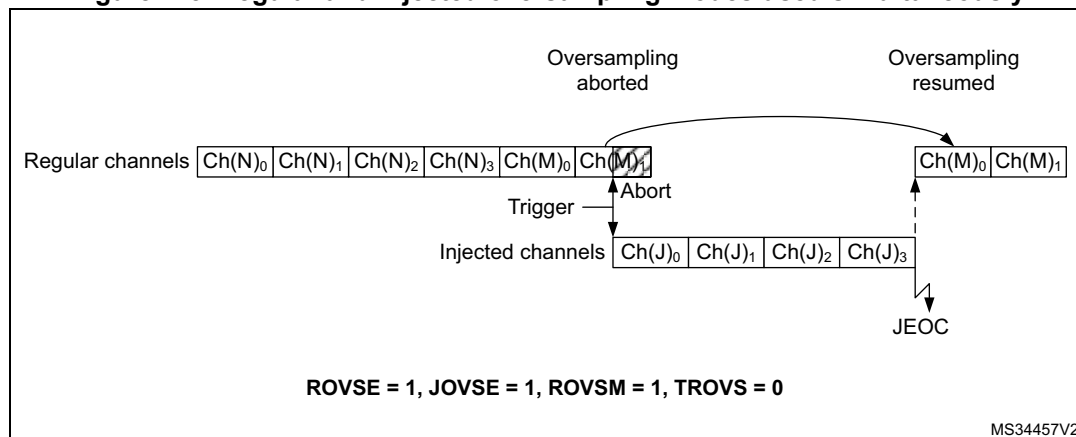
Figure 115. Regular and injected oversampling modes used simultaneously
