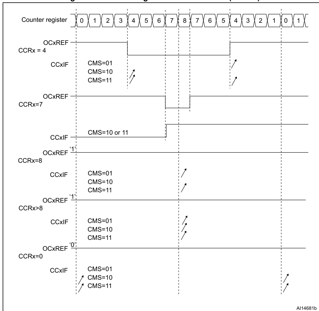
Figure 315. Center-aligned PWM waveforms (ARR=8)
