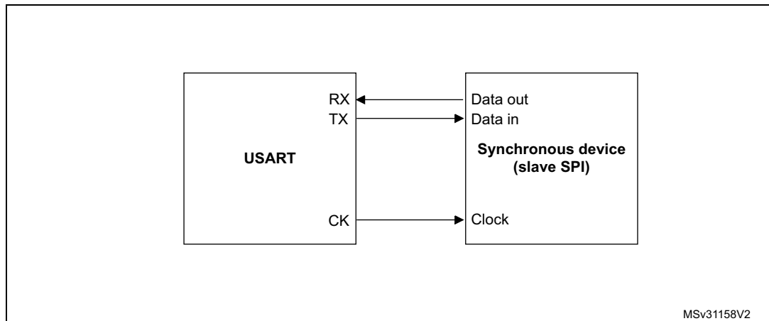
Figure 431. USART example of synchronous transmission
