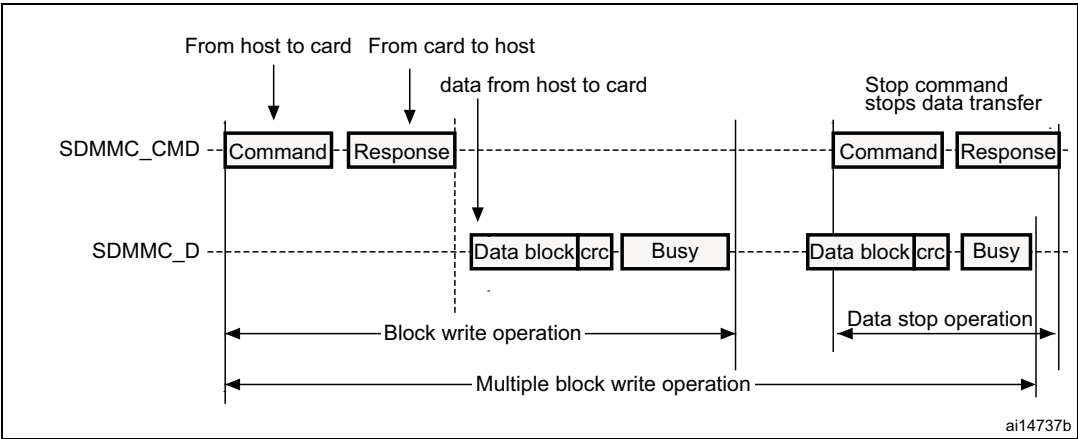
Figure 503. (Multiple) block write operation
