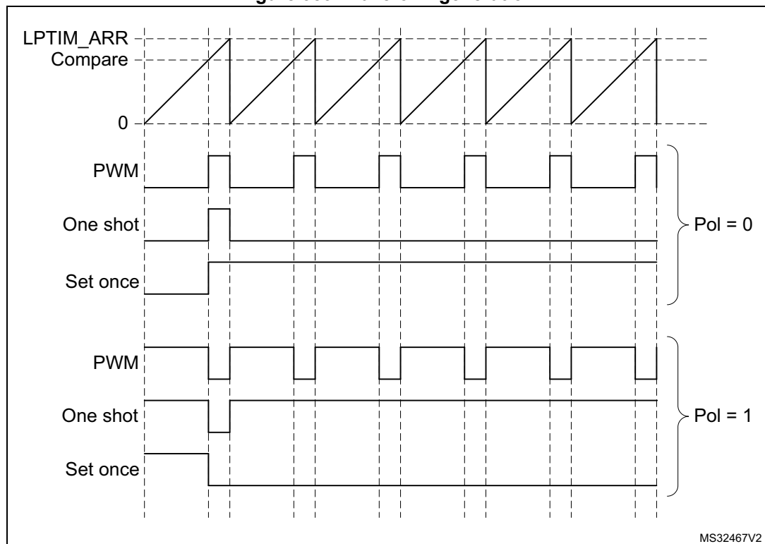
Figure 383. Waveform generation
