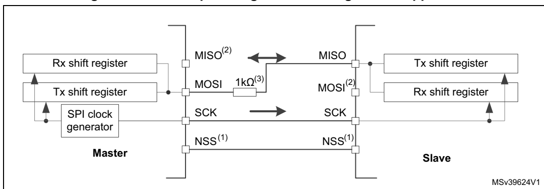
Figure 459. Half-duplex single master/ single slave application
