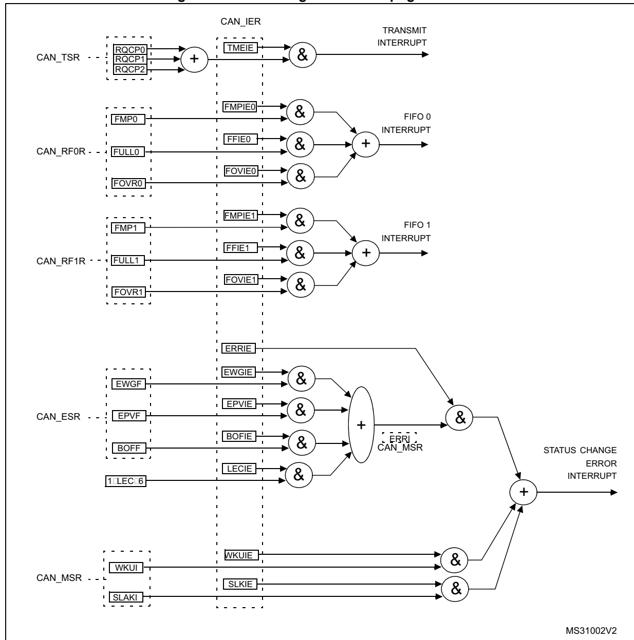
Figure 530. Event flags and interrupt generation
