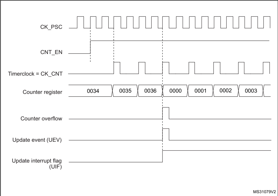
Figure 372. Counter timing diagram, internal clock divided by 2
