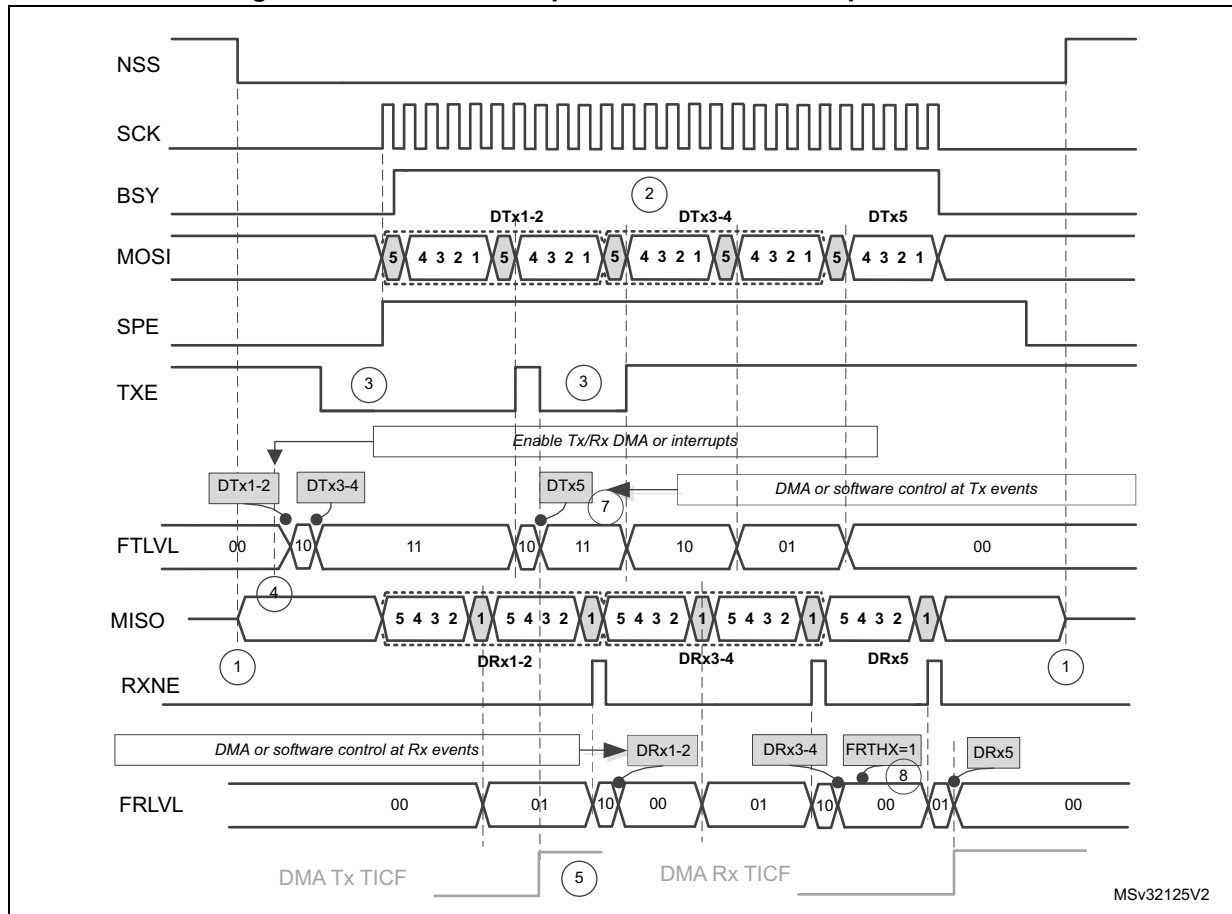
Figure 470. Master full-duplex communication in packed mode
