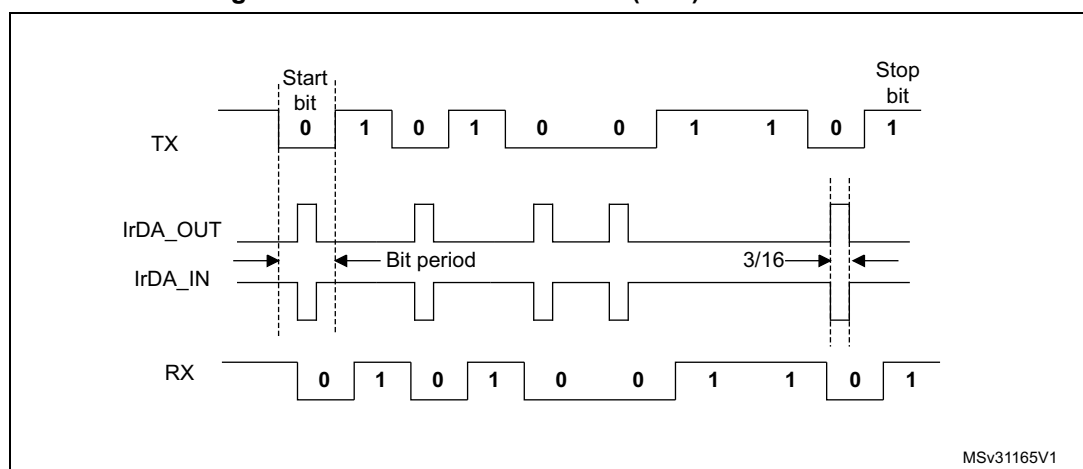
Figure 438. IrDA data modulation (3/16) - normal mode
