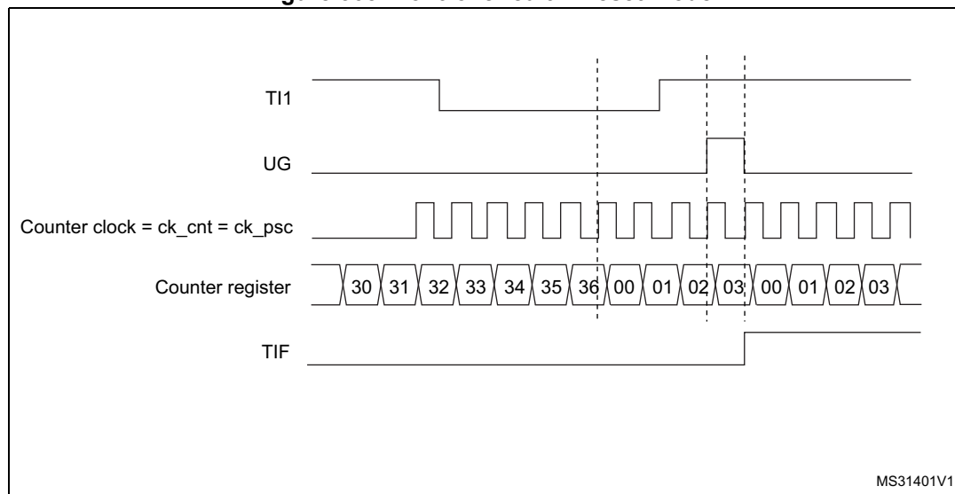
Figure 365. Control circuit in reset mode
