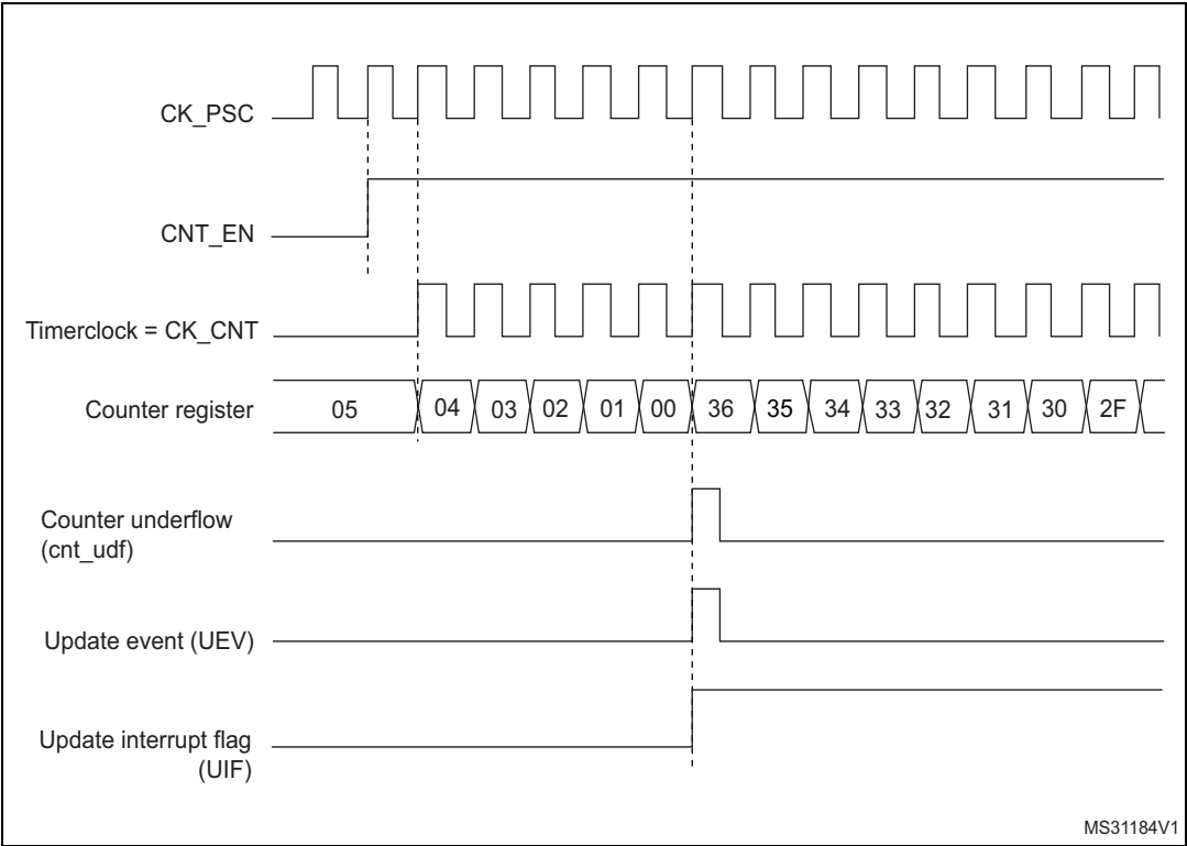
Figure 232. Counter timing diagram, internal clock divided by 1
