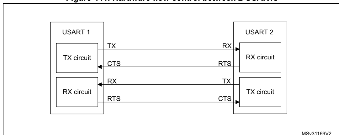
Figure 441. Hardware flow control between 2 USARTs
