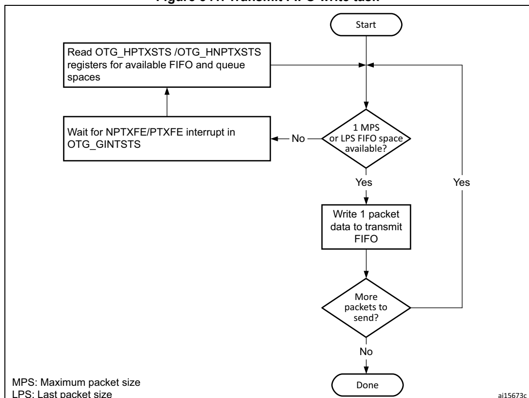
Figure 541. Transmit FIFO write task
