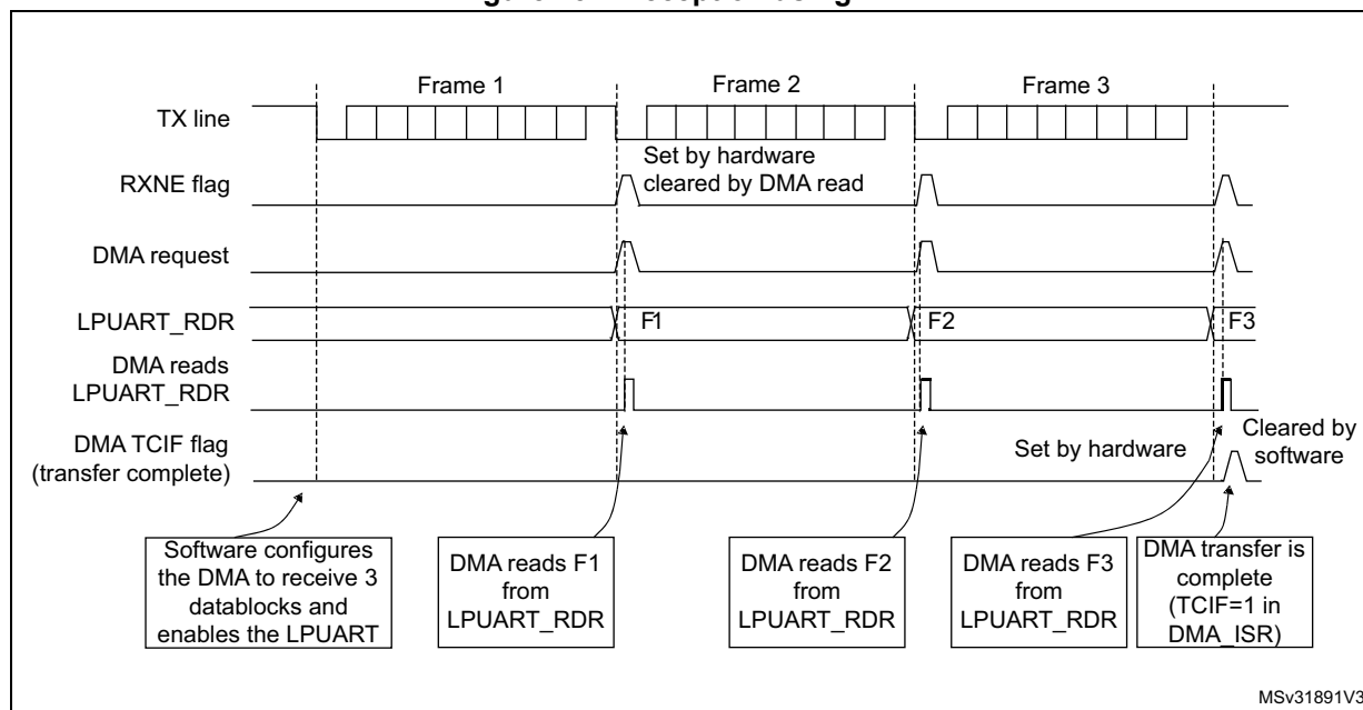
Figure 452. Reception using DMA
