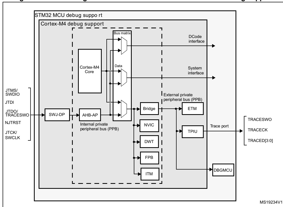
Figure 557. Block diagram of STM32 MCU and Cortex®-M4-level debug support
