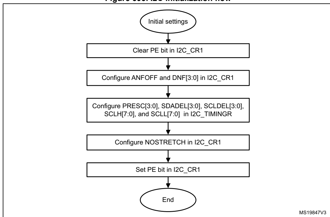
Figure 393. I2C initialization flow
