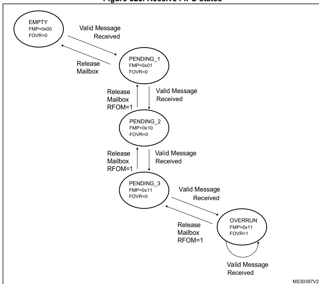
Figure 523. Receive FIFO states
