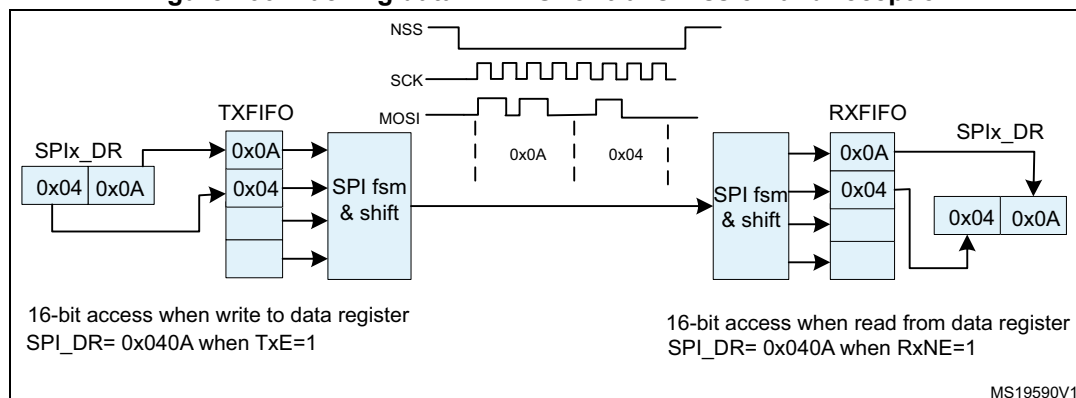
Figure 466. Packing data in FIFO for transmission and reception
