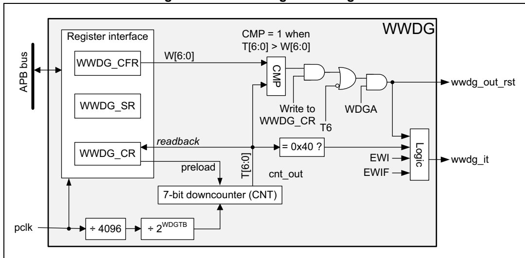
Figure 387. Watchdog block diagram
