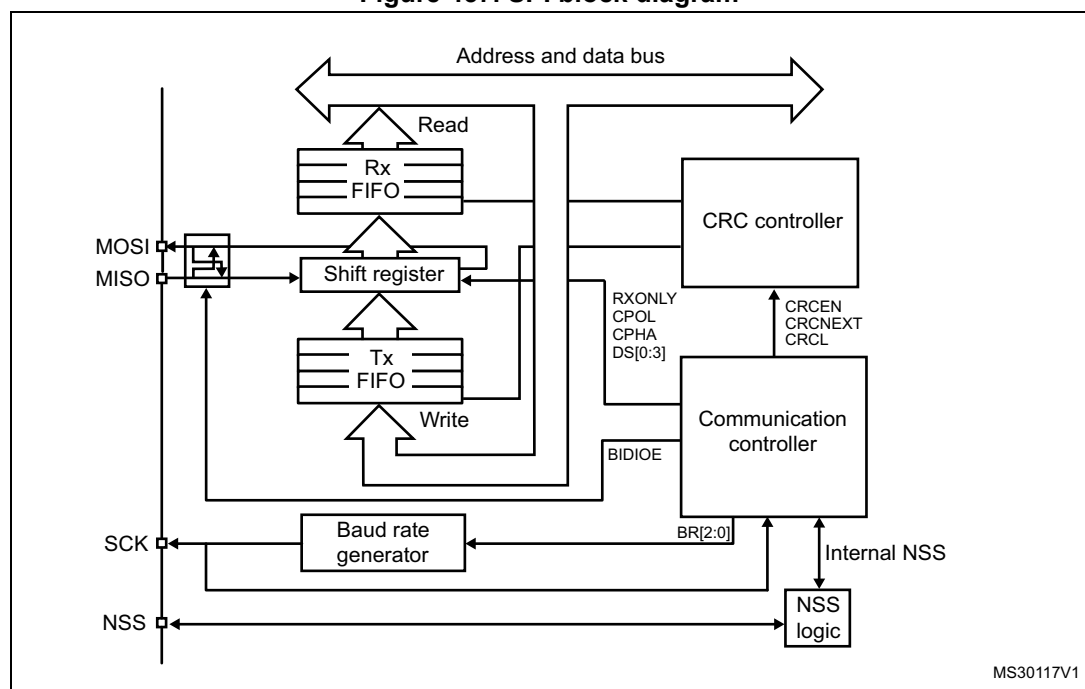
Figure 457. SPI block diagram
