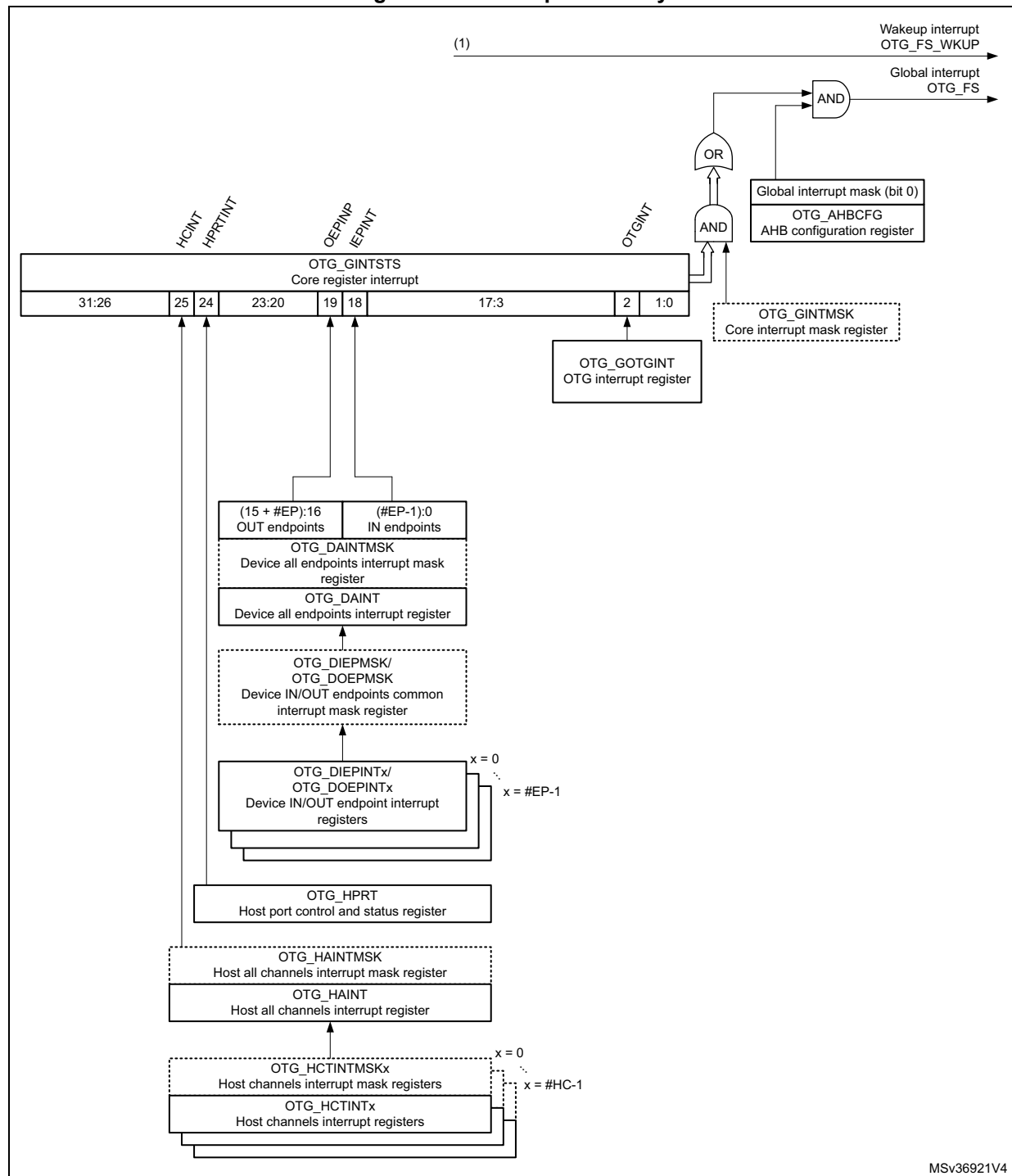
Figure 540. Interrupt hierarchy
