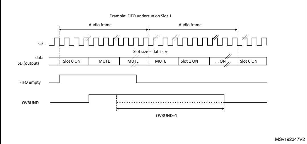
Figure 488. FIFO underrun event
