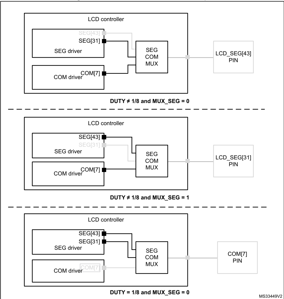
Figure 181. SEG/COM mux feature example
