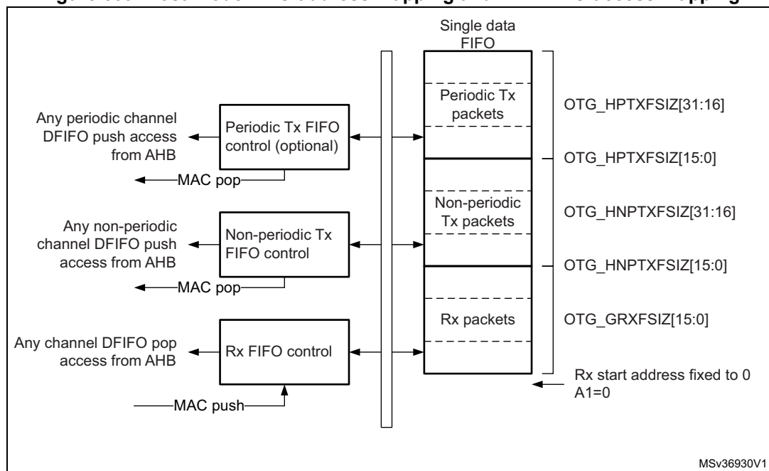
Figure 539. Host-mode FIFO address mapping and AHB FIFO access mapping
