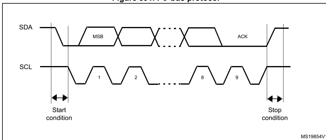
Figure 391. I 2 C-bus protocol
