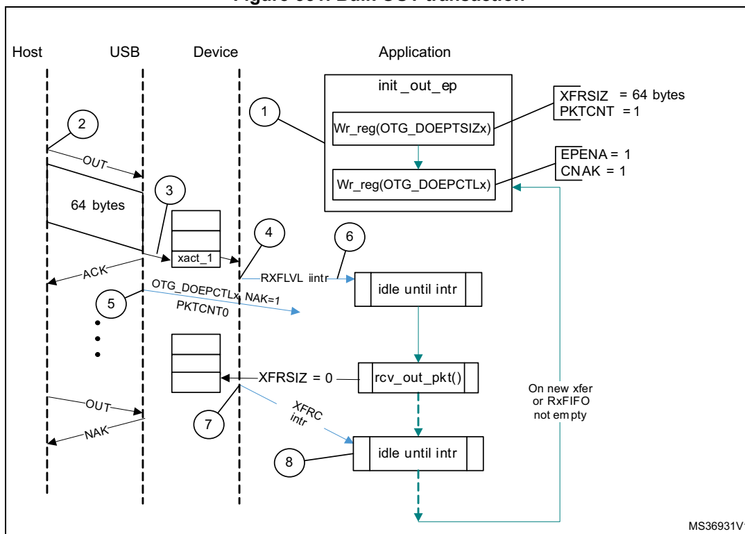
Figure 551. Bulk OUT transaction
