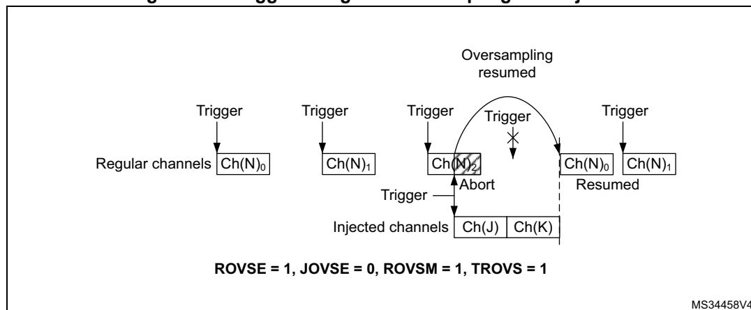
Figure 116. Triggered regular oversampling with injection
