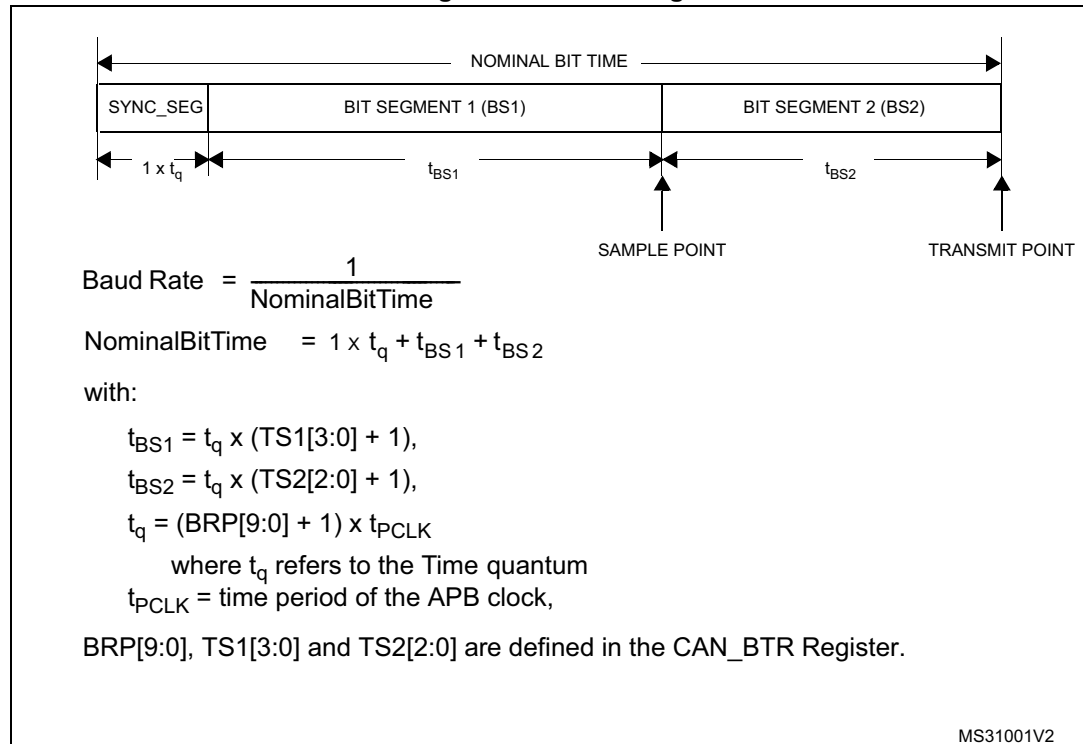
Figure 528. Bit timing
