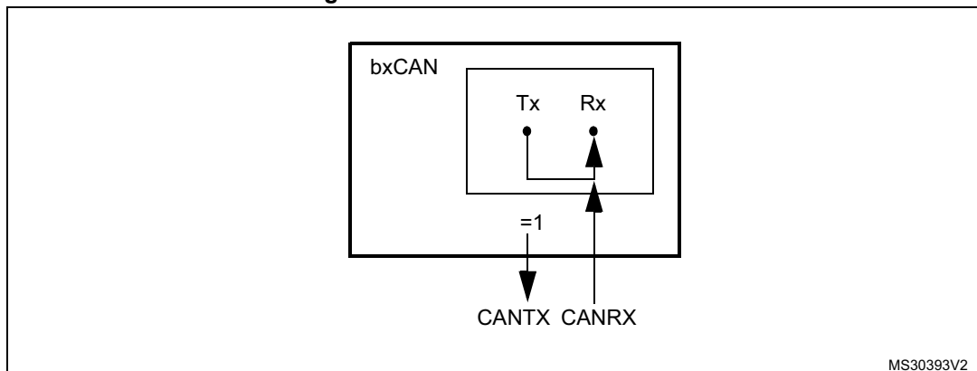
Figure 519. bxCAN in silent mode
