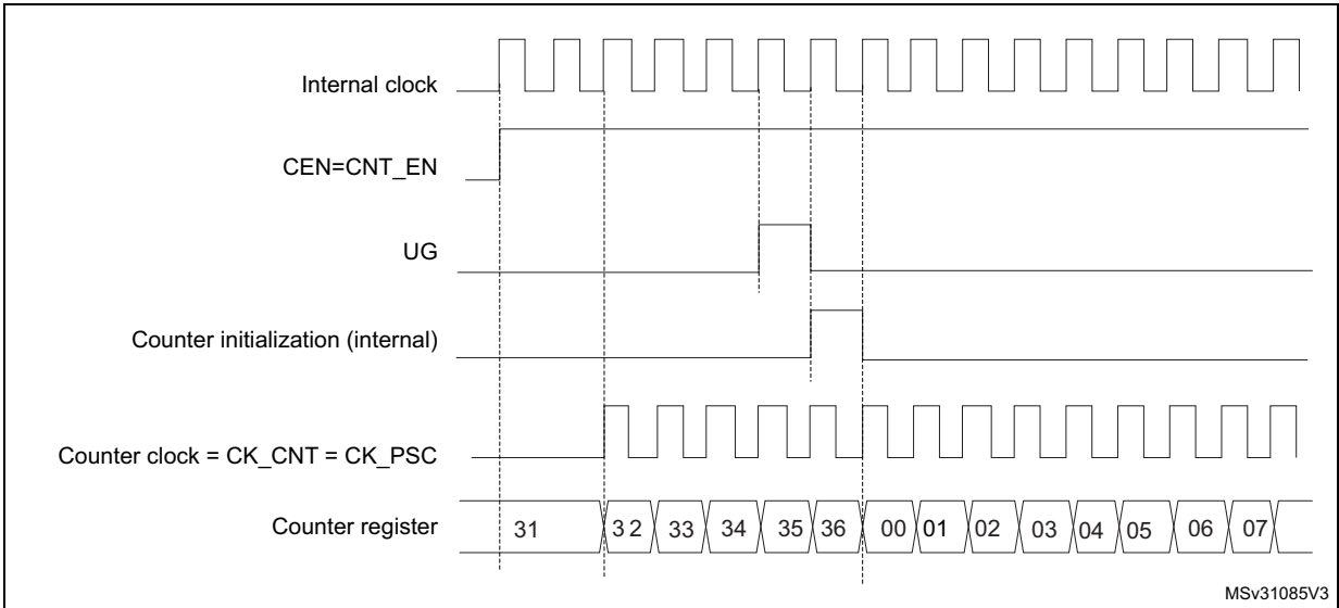
Figure 345. Control circuit in normal mode, internal clock divided by 1
