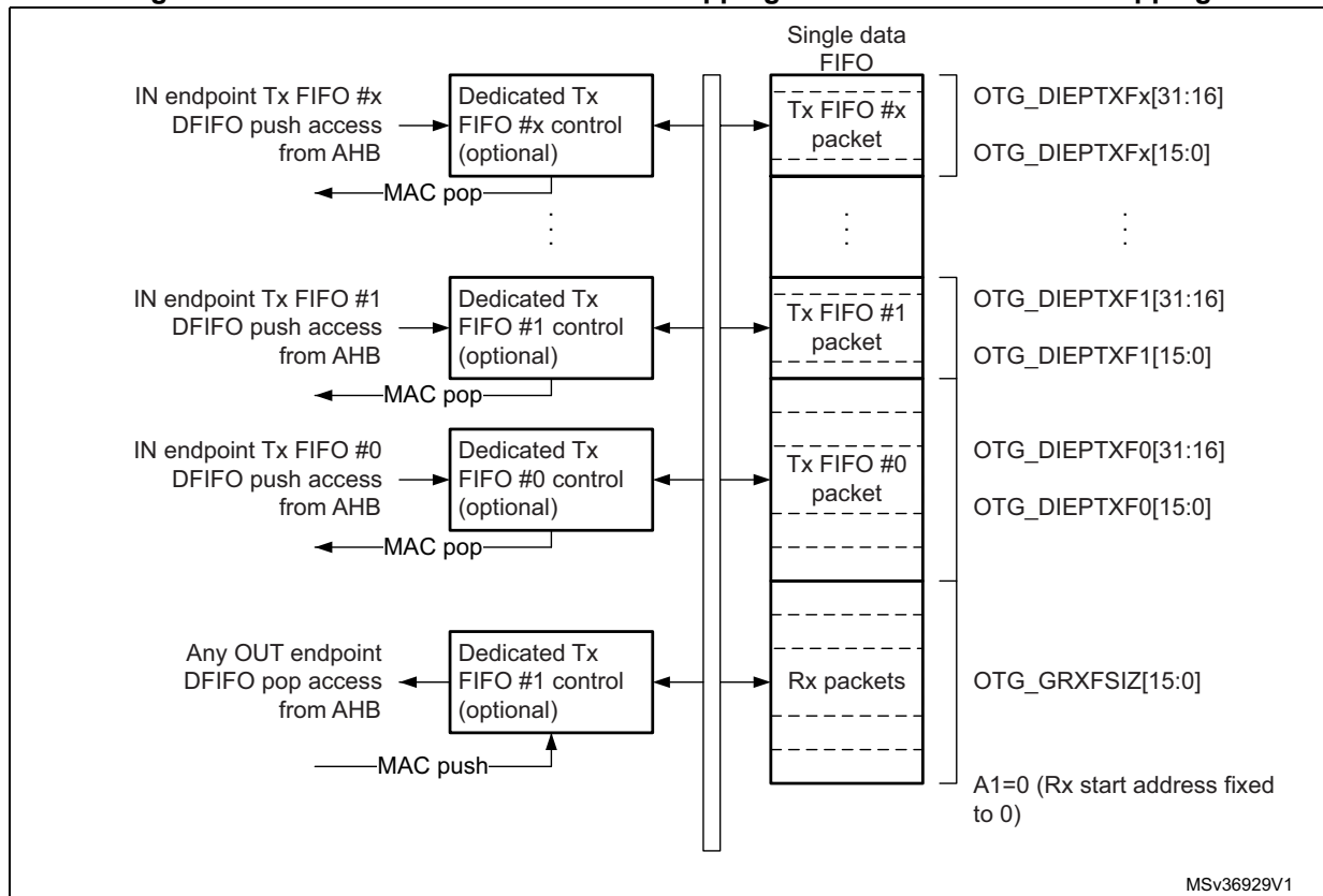
Figure 538. Device-mode FIFO address mapping and AHB FIFO access mapping
