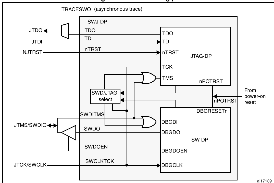
Figure 558. SWJ debug port
