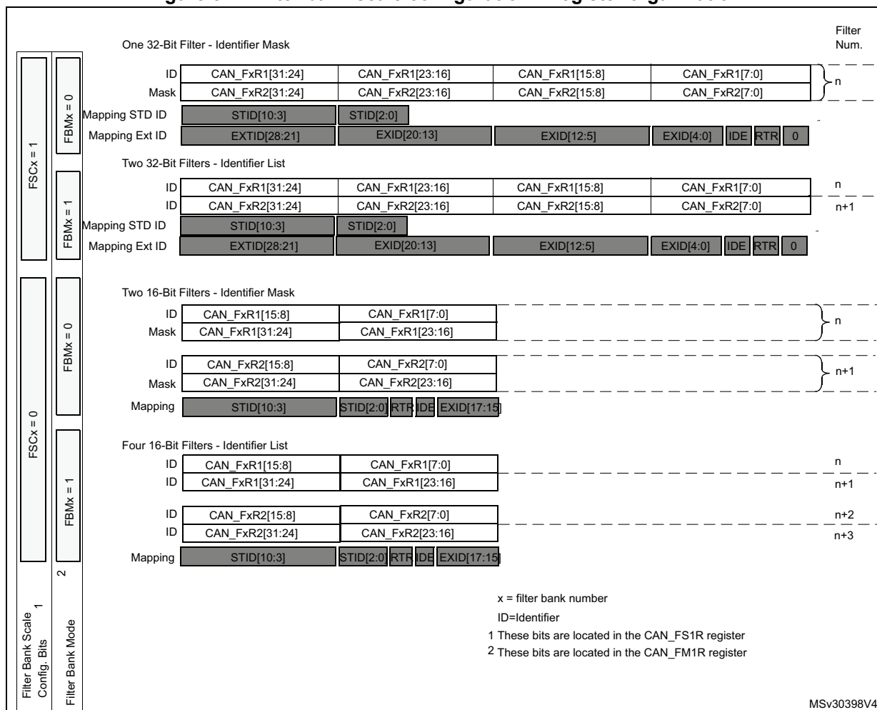
Figure 524. Filter bank scale configuration - Register organization
