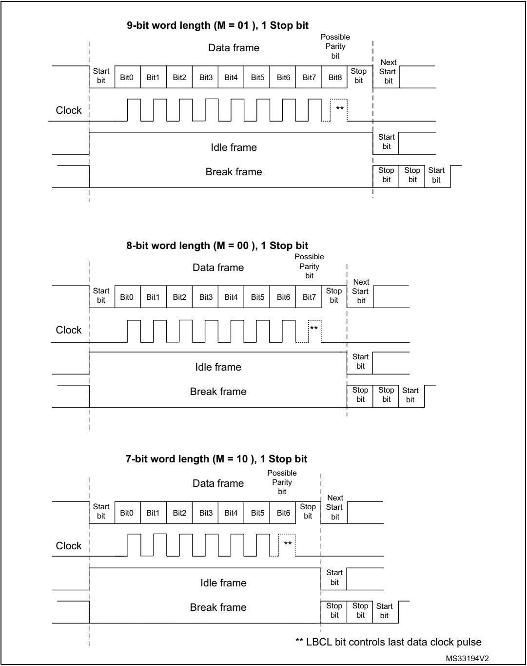
Figure 421. Word length programming
