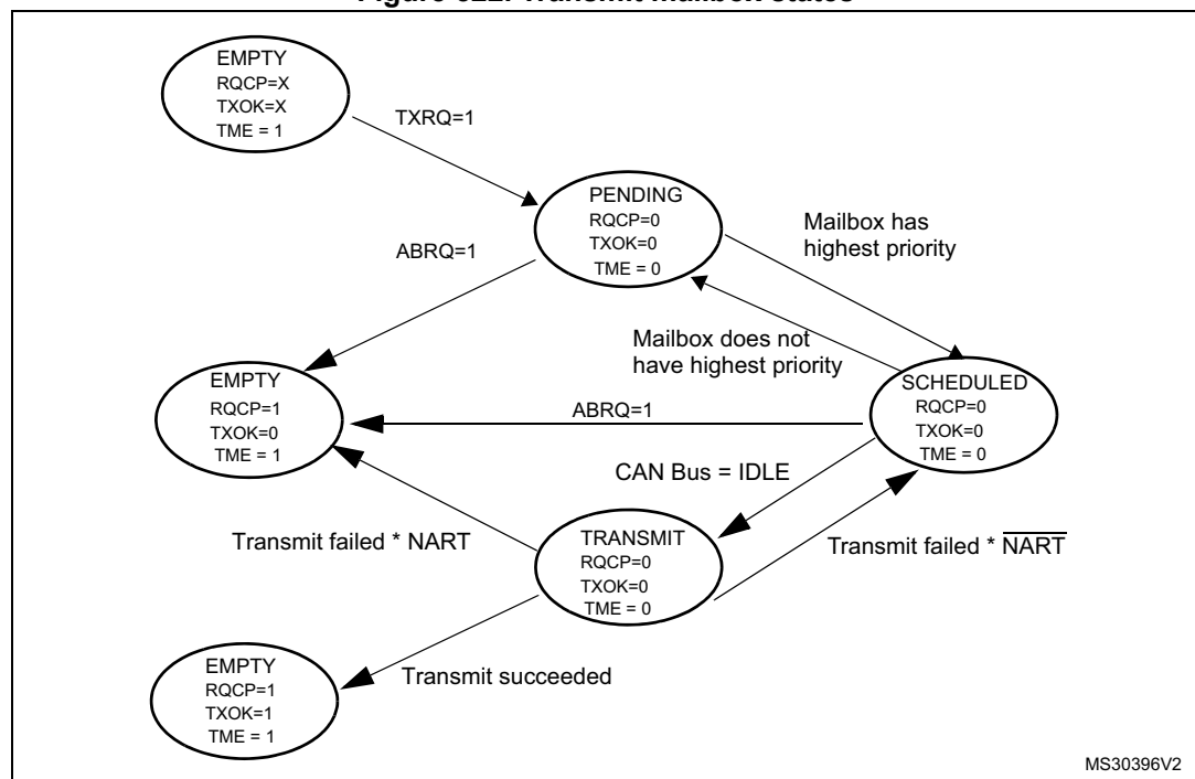
Figure 522. Transmit mailbox states
