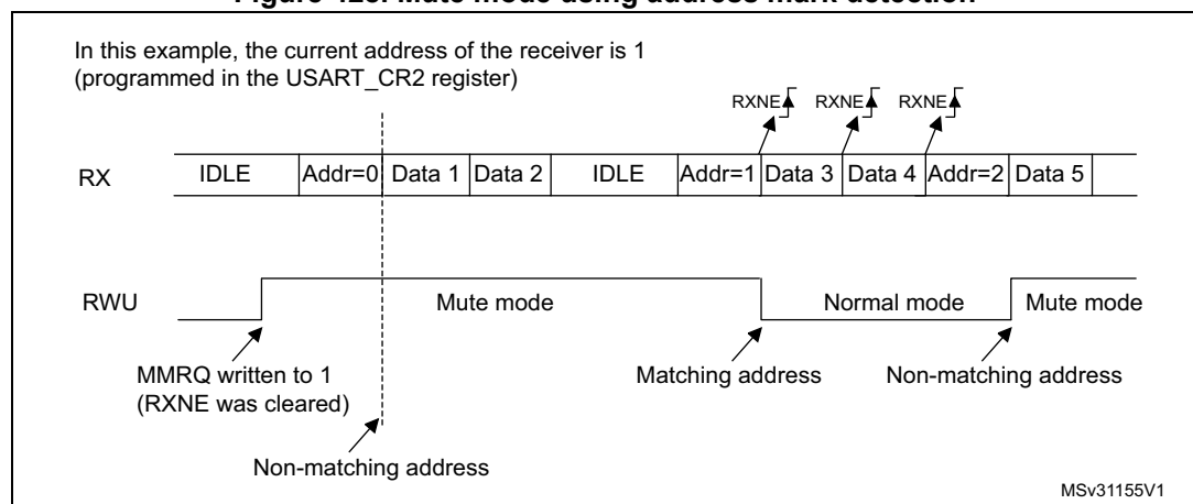
Figure 428. Mute mode using address mark detection
