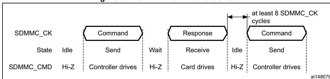
Figure 512. SDMMC command transfer
