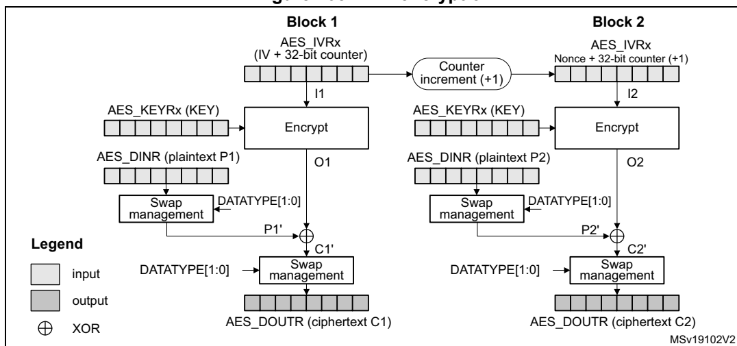
Figure 208. CTR encryption
