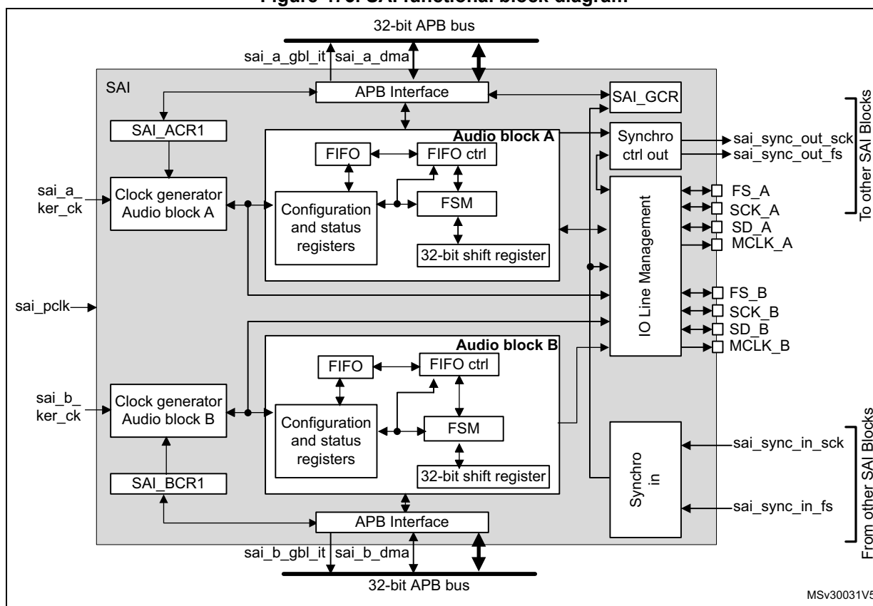
Figure 473. SAI functional block diagram
