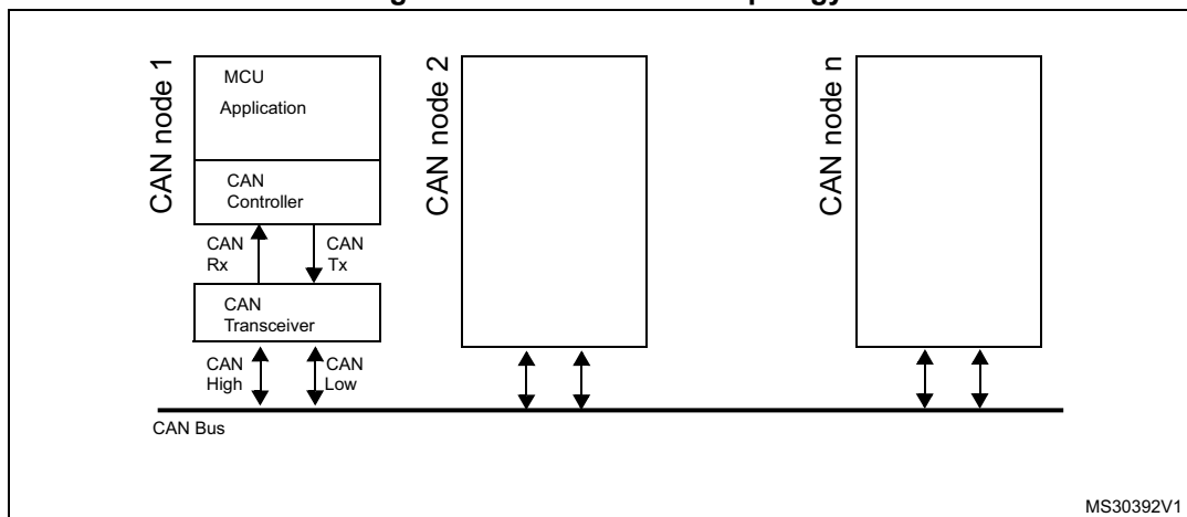
Figure 515. CAN network topology
