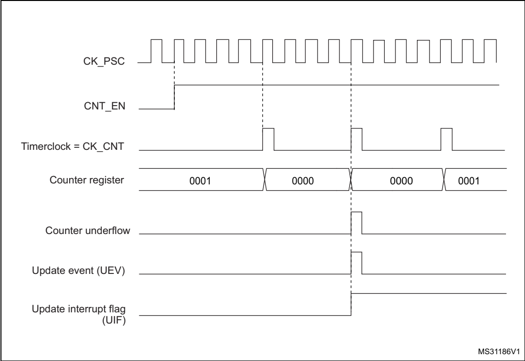
Figure 234. Counter timing diagram, internal clock divided by 4
