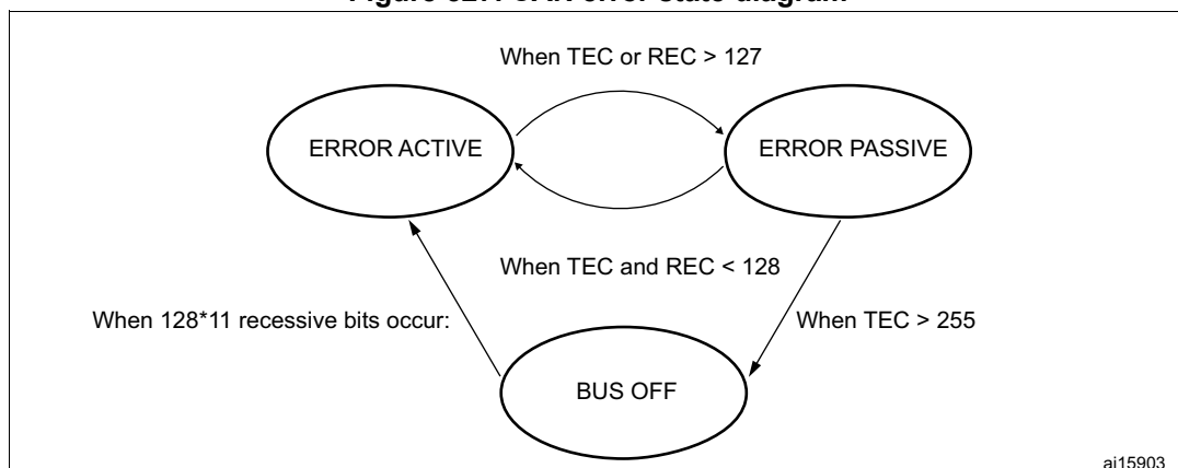
Figure 527. CAN error state diagram
