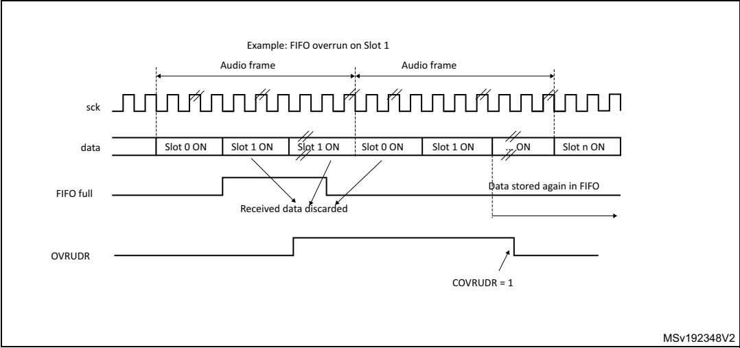
Figure 487. Overrun detection error
