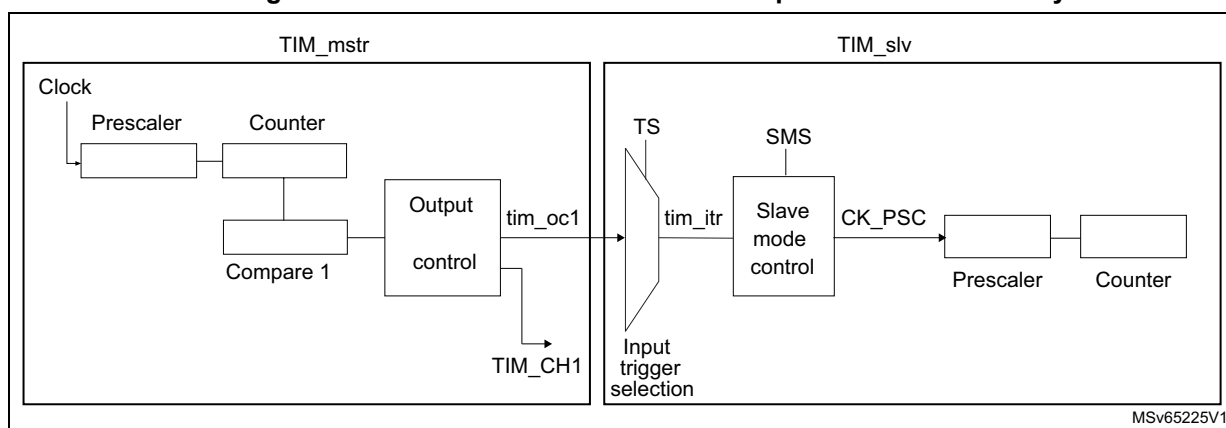
Figure 328. Master/slave connection example with 1 channel only timers
