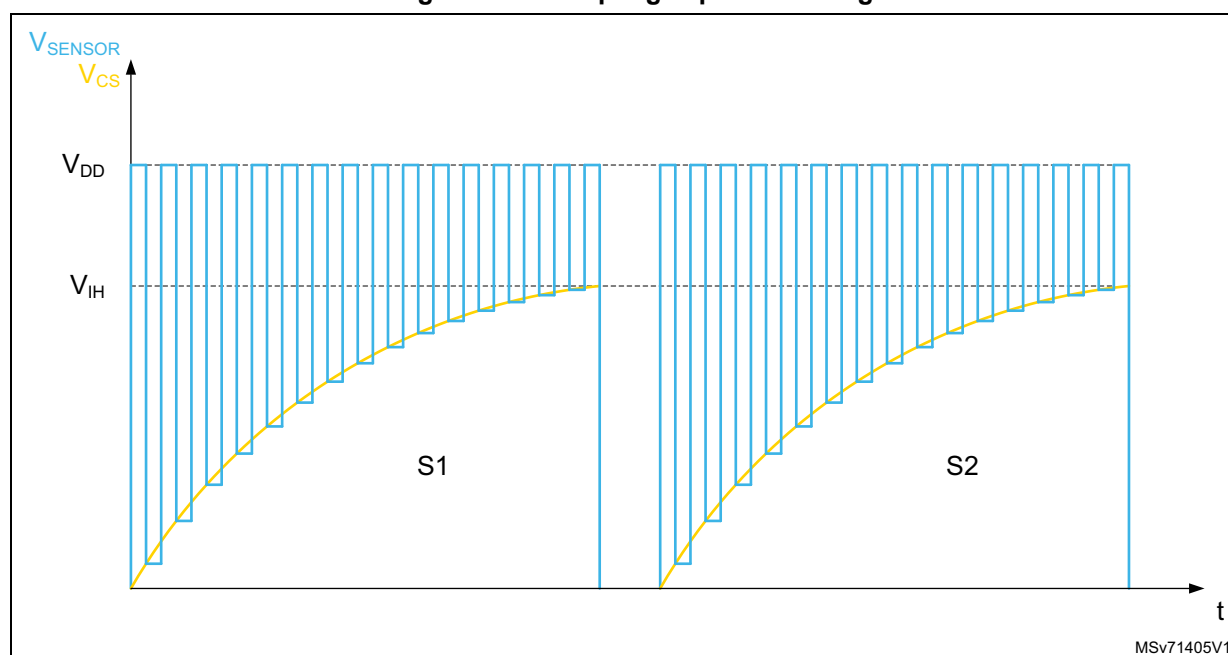
Figure 185. Sampling capacitor voltage variation
