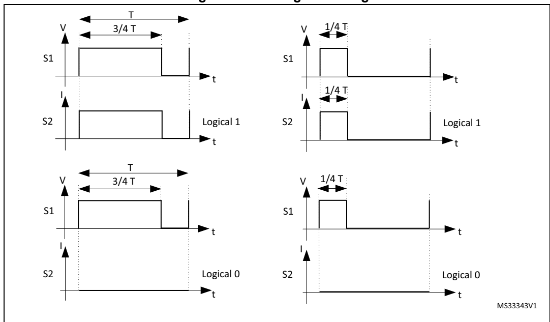
Figure 490. S2 signal coding
