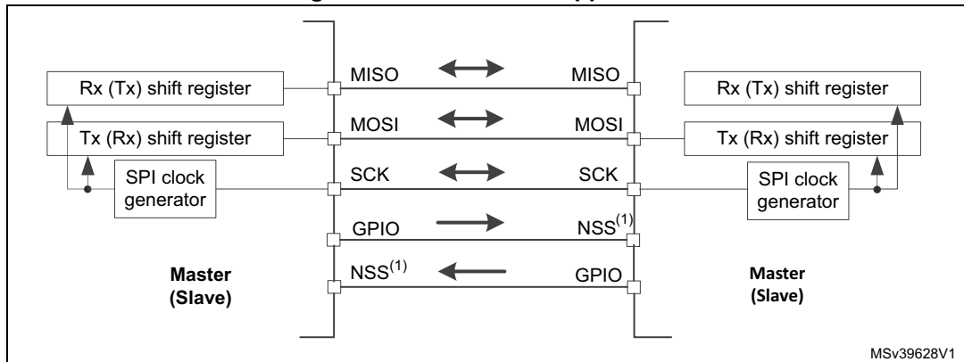
Figure 462. Multimaster application
