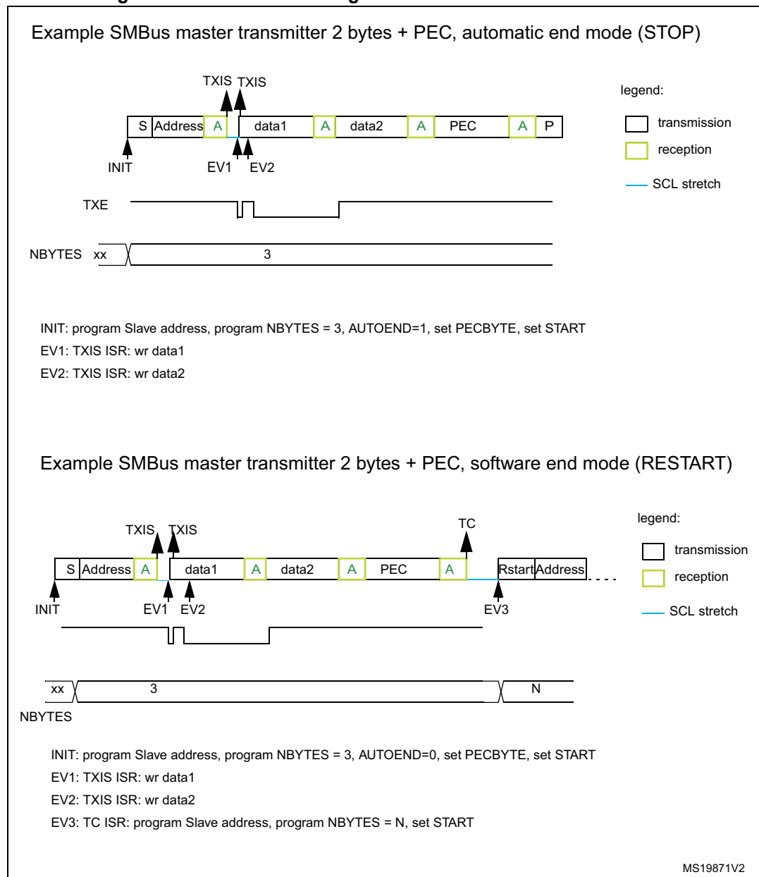
Figure 418. Bus transfer diagrams for SMBus master transmitter
