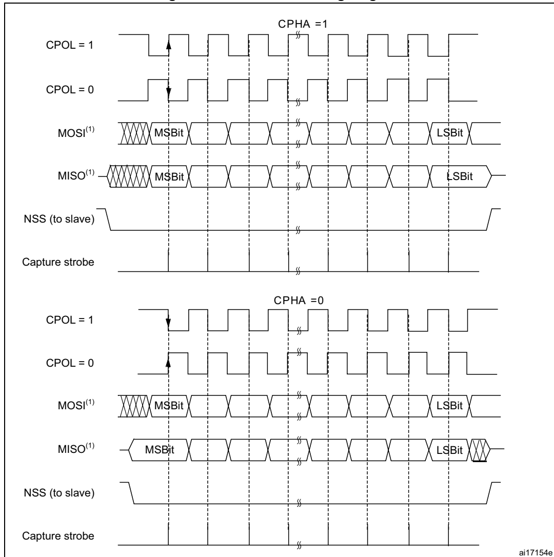
Figure 464. Data clock timing diagram
