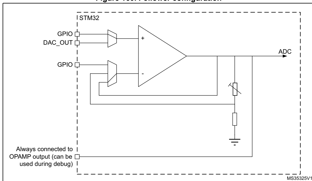
Figure 160. Follower configuration
