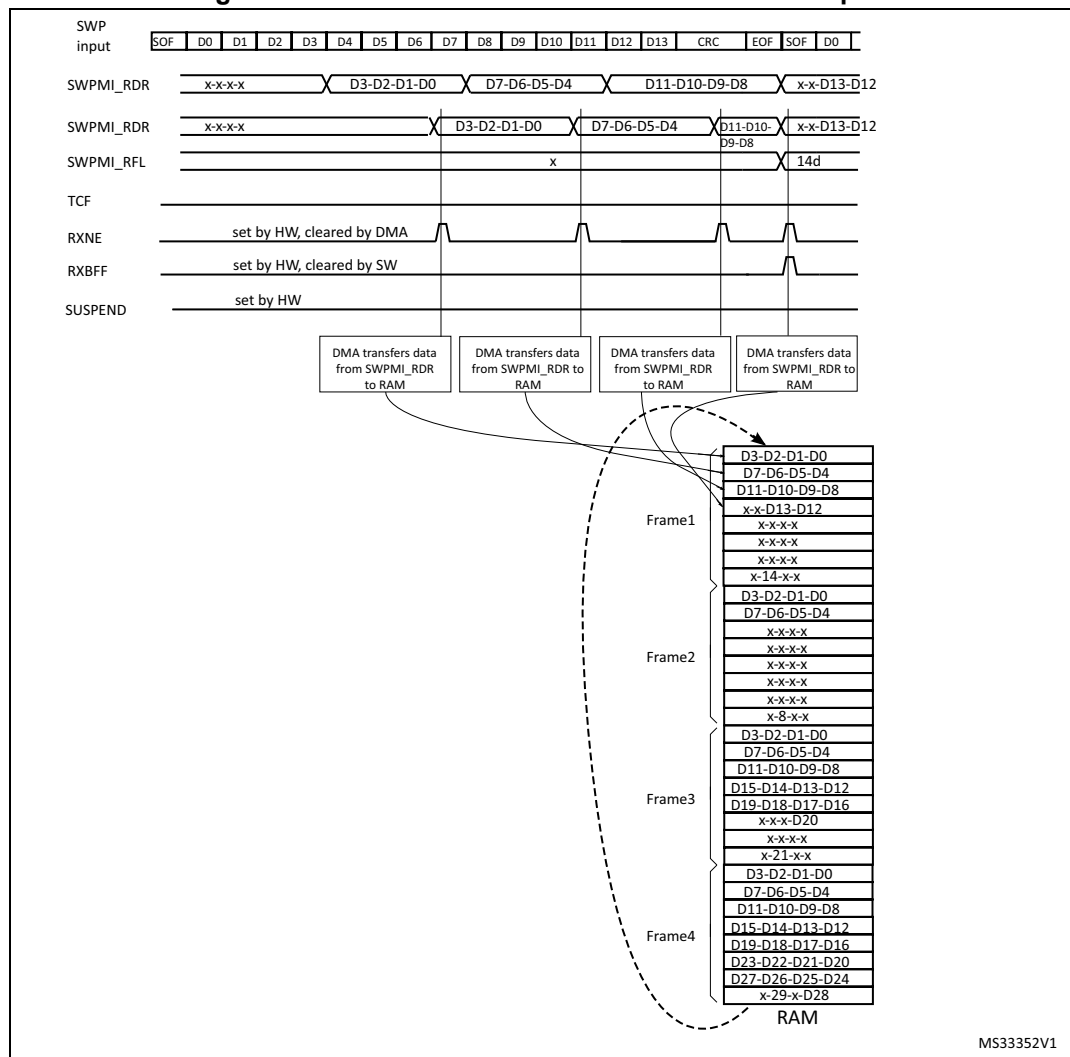
Figure 499. SWPMI Multi software buffer mode reception
