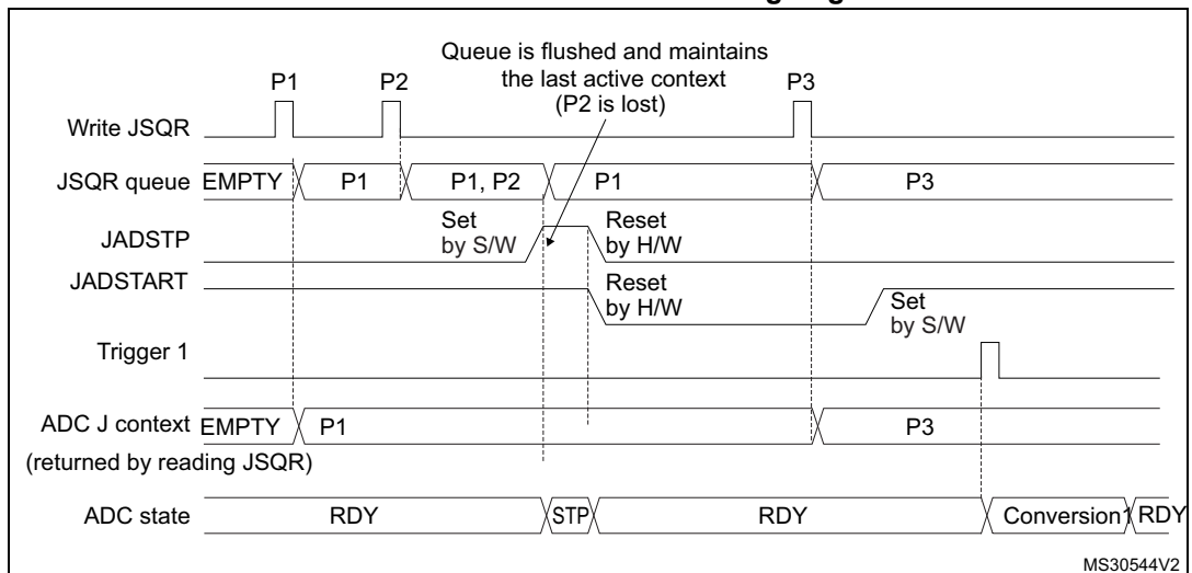
Figure 88. Flushing JSQR queue of context by setting JADSTP = 1 (JQM = 0) Case when JADSTP occurs outside an ongoing conversion
