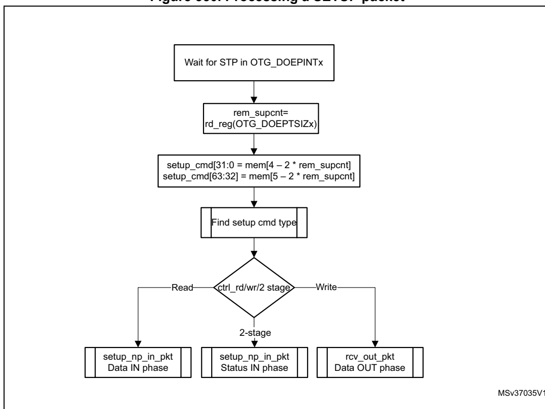
Figure 550. Processing a SETUP packet
