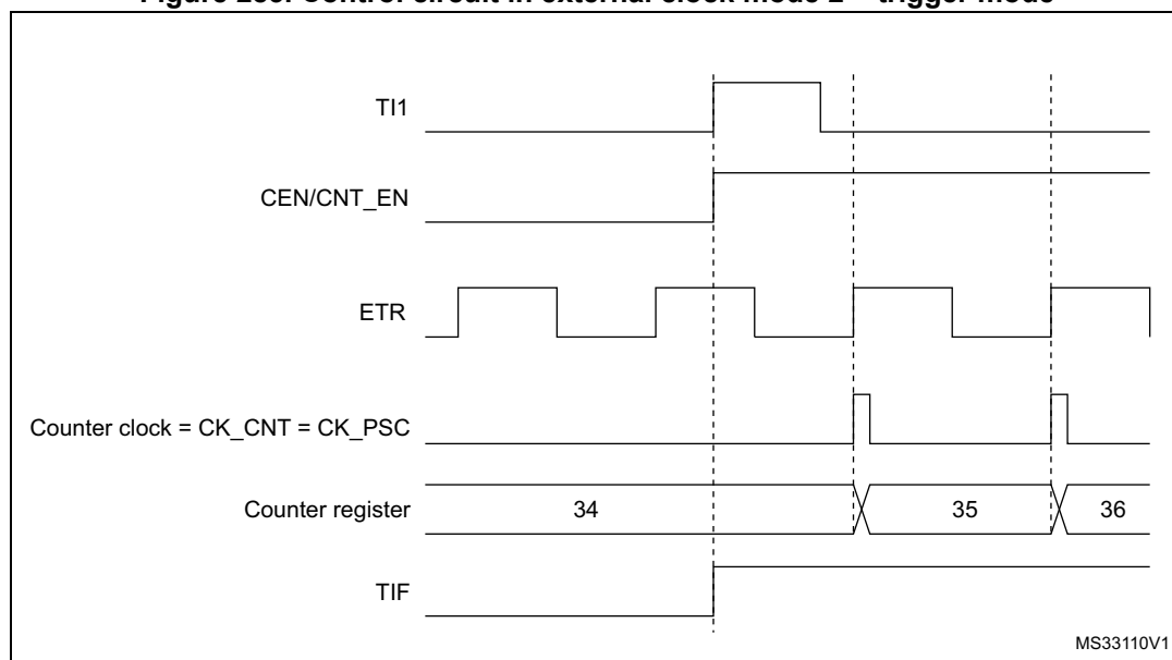
Figure 283. Control circuit in external clock mode 2 + trigger mode
