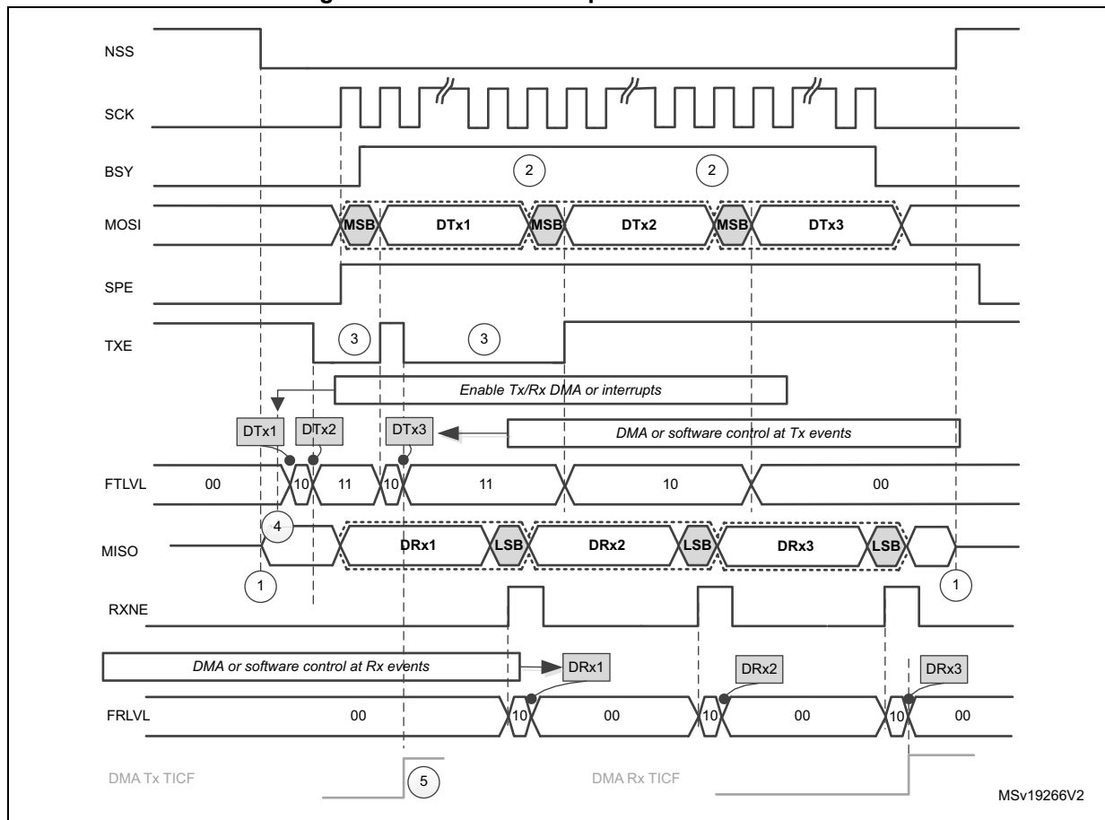
Figure 467. Master full-duplex communication
