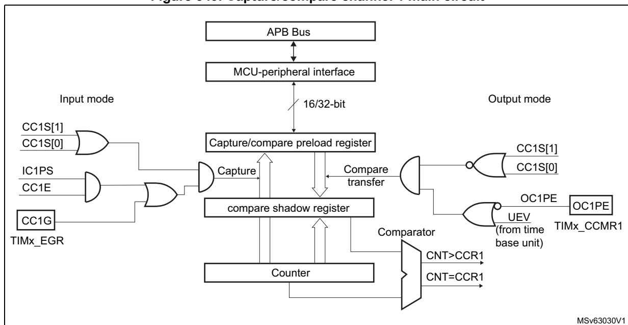
Figure 349. Capture/compare channel 1 main circuit
