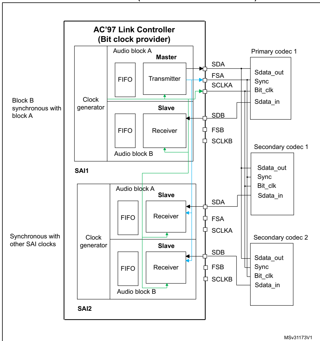
Figure 481. Example of typical AC'97 configuration on devices featuring at least 2 embedded SAIs (three external AC'97 decoders)
