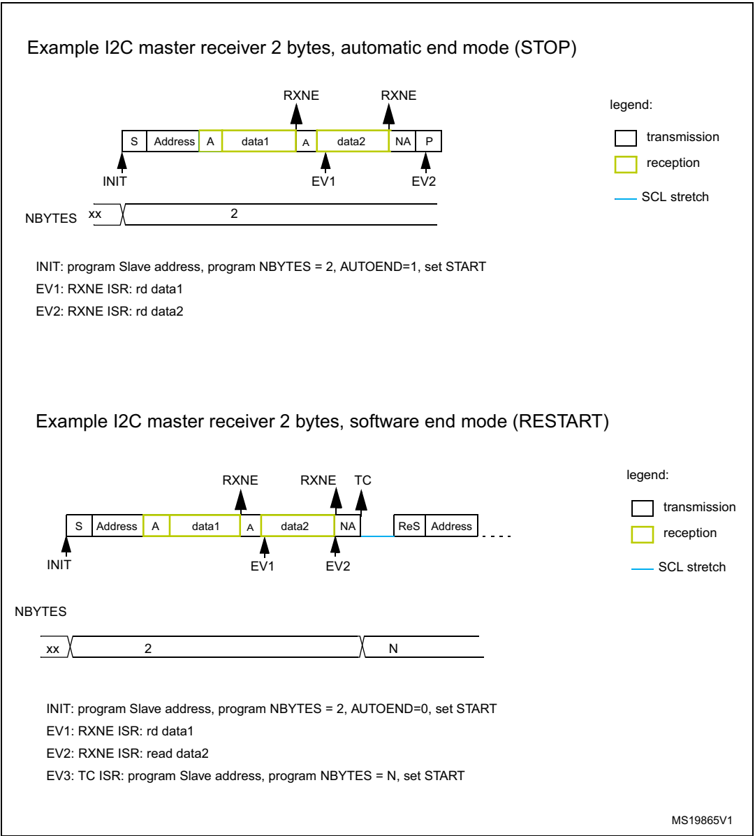
Figure 412. Transfer bus diagrams for I2C master receiver (mandatory events only)
