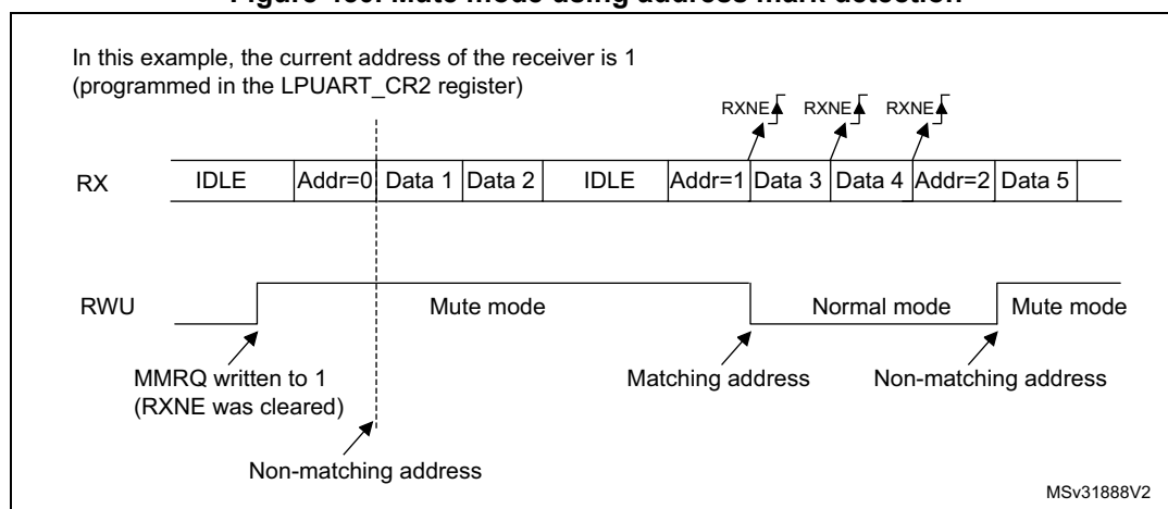
Figure 450. Mute mode using address mark detection
