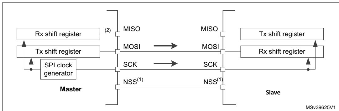
Figure 460. Simplex single master/single slave application (master in transmit-only/ slave in receive-only mode)
