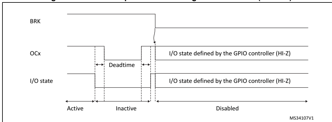
Figure 270. PWM output state following BRK assertion (OSSI=0)
