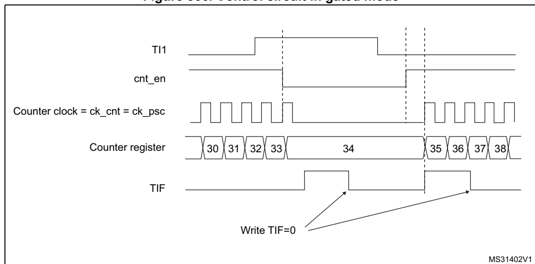
Figure 366. Control circuit in gated mode
