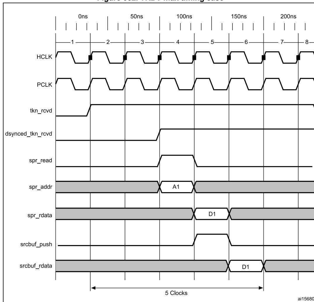
Figure 552. TRDT max timing case
