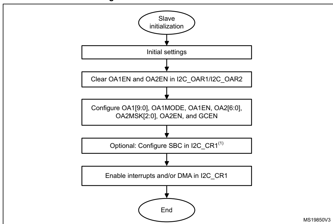
Figure 396. Slave initialization flow
