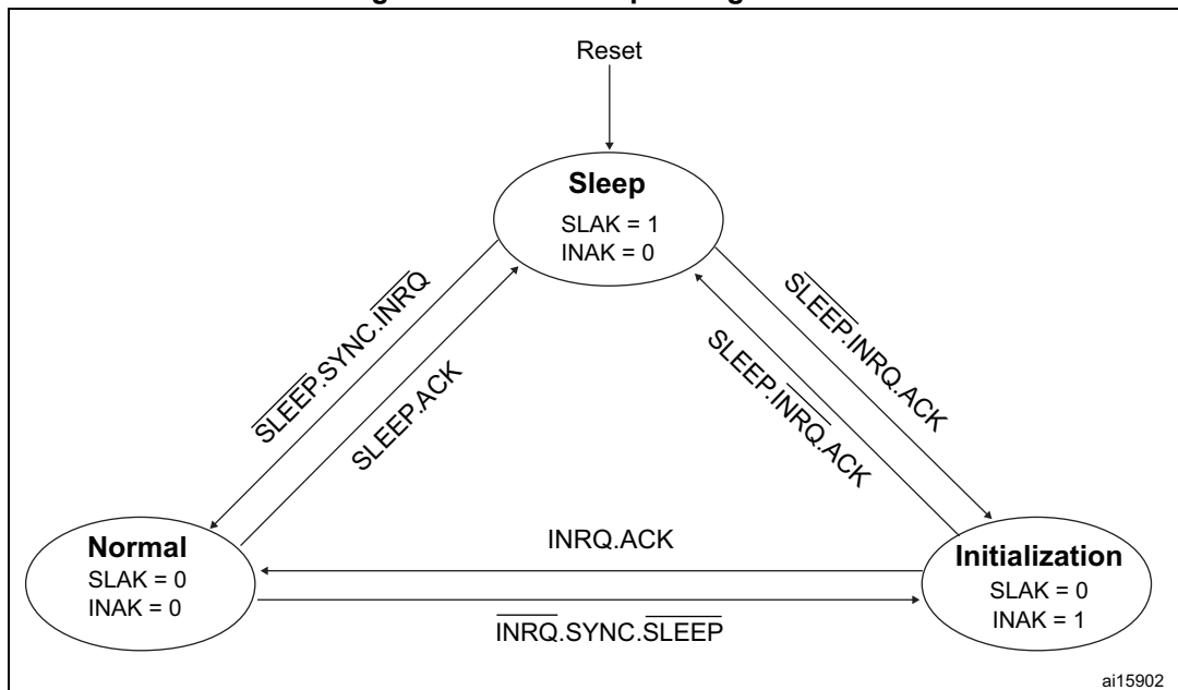
Figure 518. bxCAN operating modes
