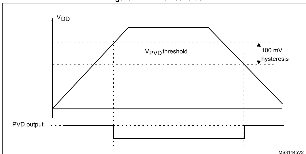
Figure 12. PVD thresholds
