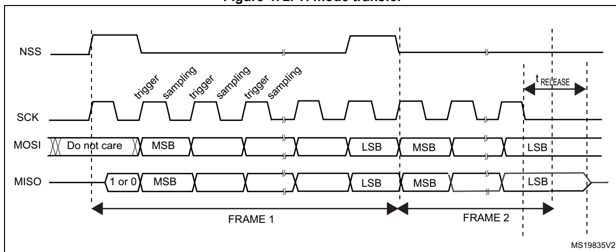
Figure 472. TI mode transfer
