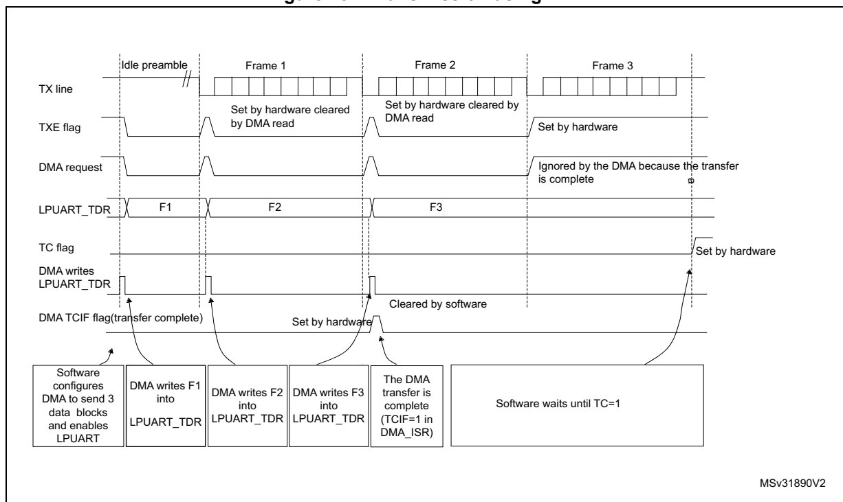
Figure 451. Transmission using DMA
