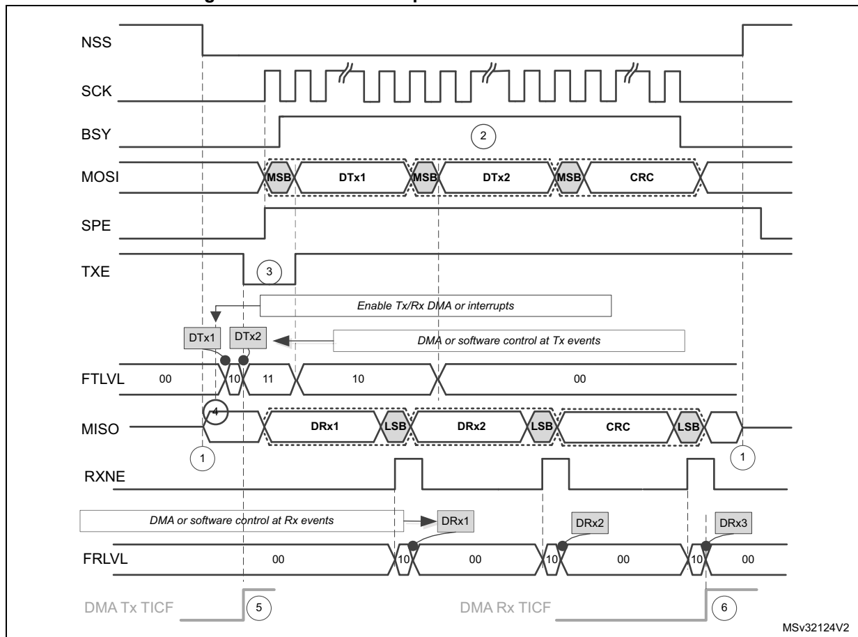
Figure 469. Master full-duplex communication with CRC
