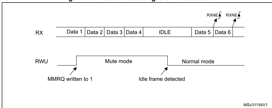
Figure 449. Mute mode using Idle line detection
