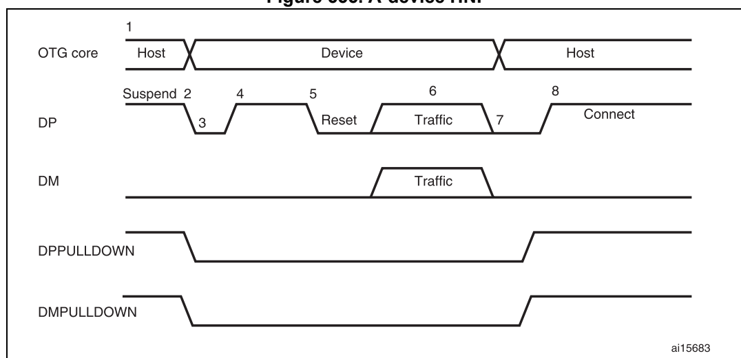
Figure 555. A-device HNP
