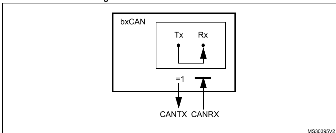
Figure 521. bxCAN in combined mode
