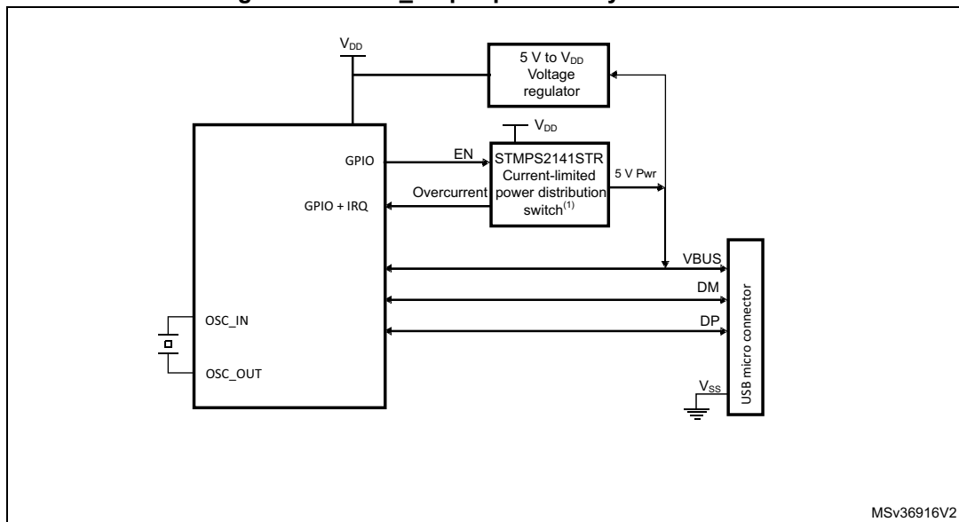
Figure 534. OTG_FS peripheral-only connection
