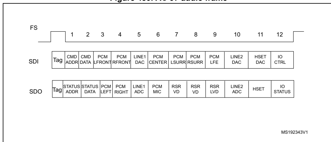
Figure 480. AC'97 audio frame
