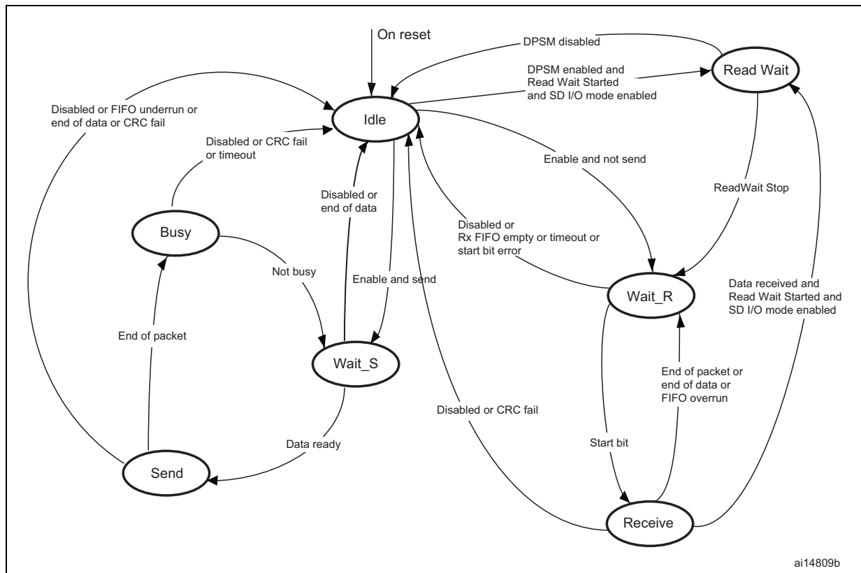
Figure 514. Data path state machine (DPSM)
