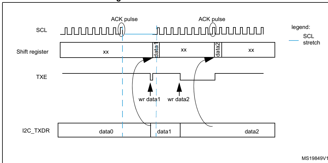
Figure 395. Data transmission
