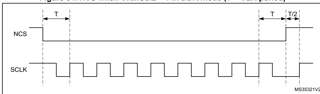
Figure 64. NCS when CKMODE = 1 in DDR mode ( T = \text{CLK period} )
