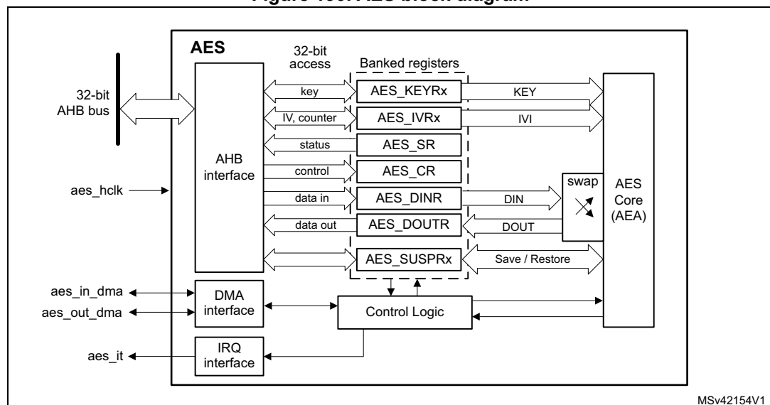
Figure 190. AES block diagram
