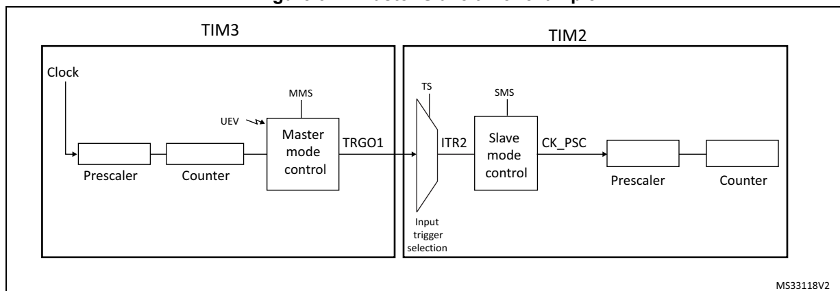
Figure 327. Master/Slave timer example
