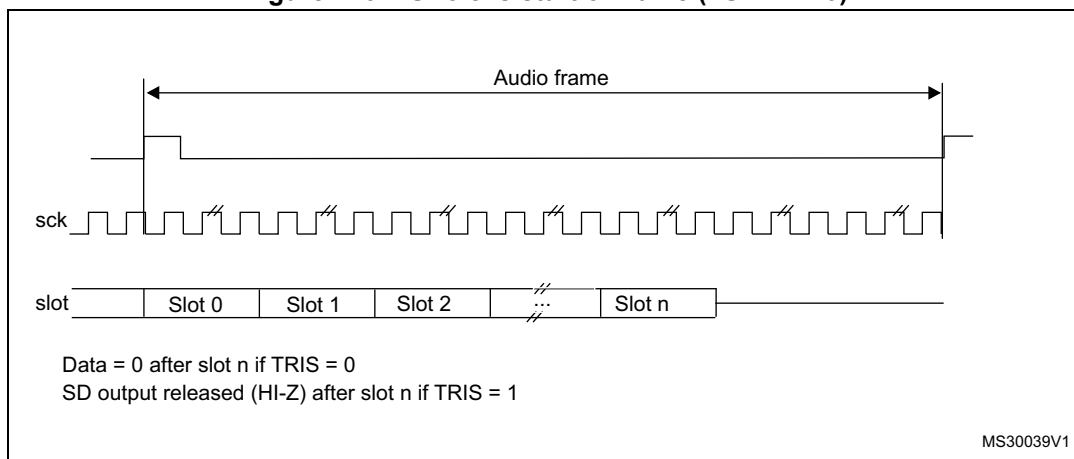
Figure 476. FS role is start of frame (FSDEF = 0)
