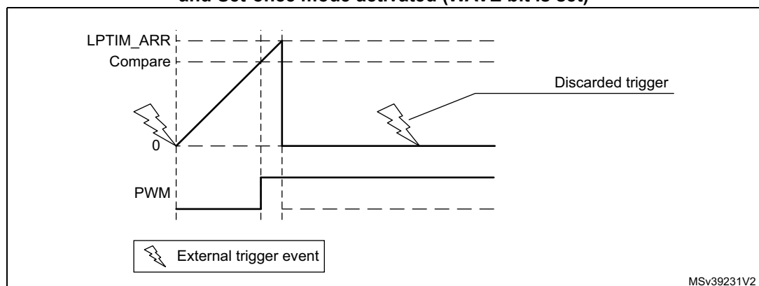
Figure 381. LPTIM output waveform, Single counting mode configuration and Set-once mode activated (WAVE bit is set)
