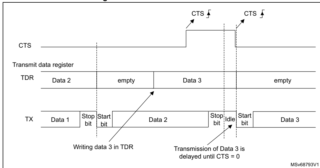
Figure 443. RS232 CTS flow control
