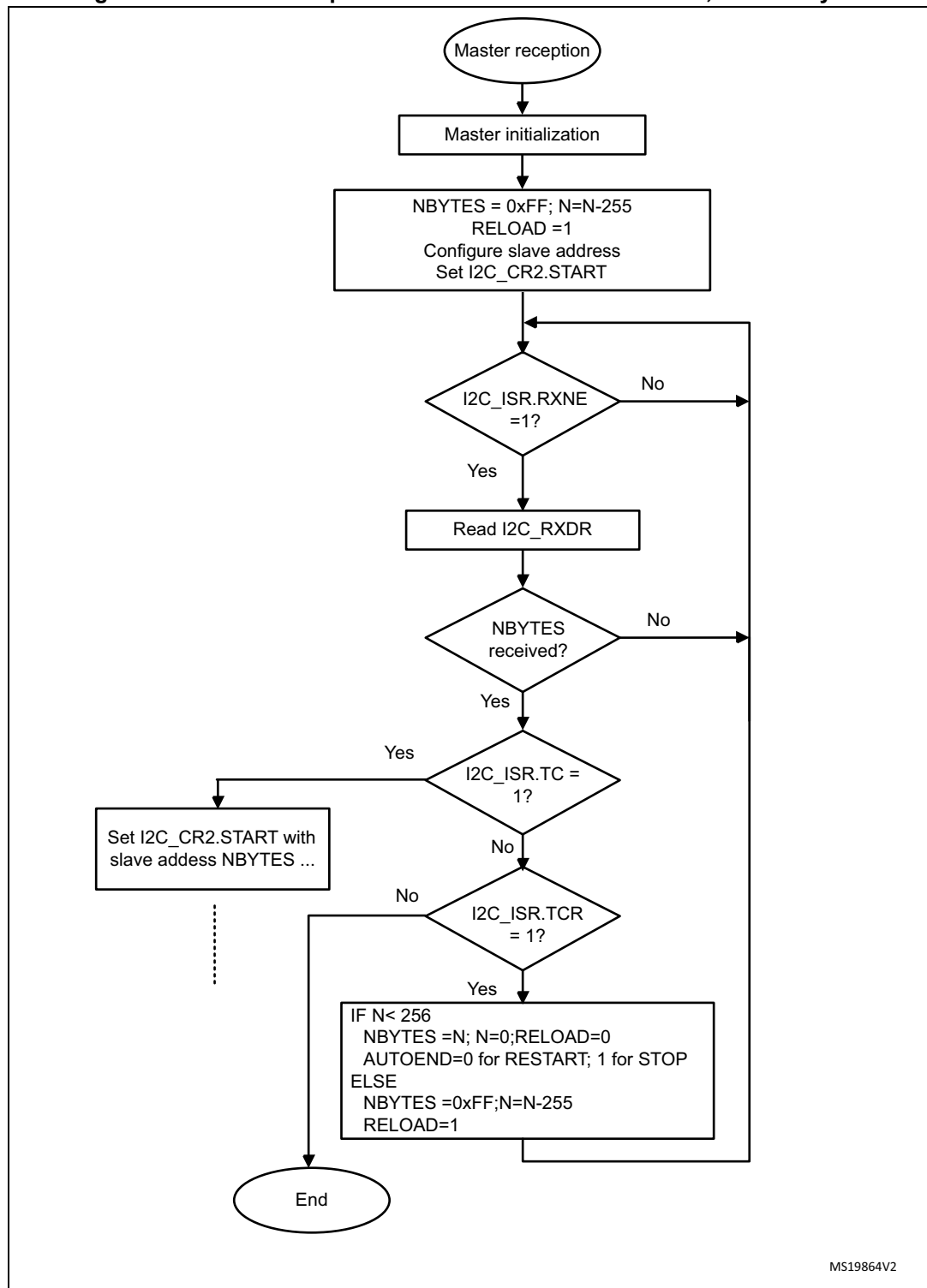
Figure 411. Transfer sequence flow for I2C master receiver, N &gt; 255 bytes
