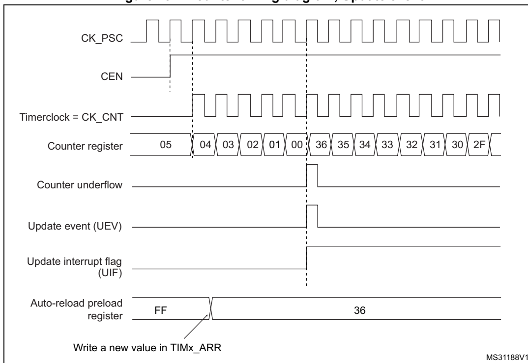
Figure 297. Counter timing diagram, Update event
