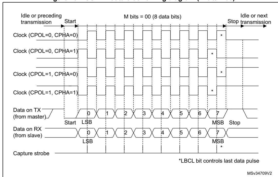
Figure 432. USART data clock timing diagram (M bits = 00)
