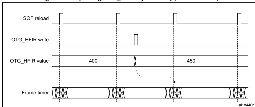
Figure 537. Updating OTG_HFIR dynamically (RLDCTRL = 1)
