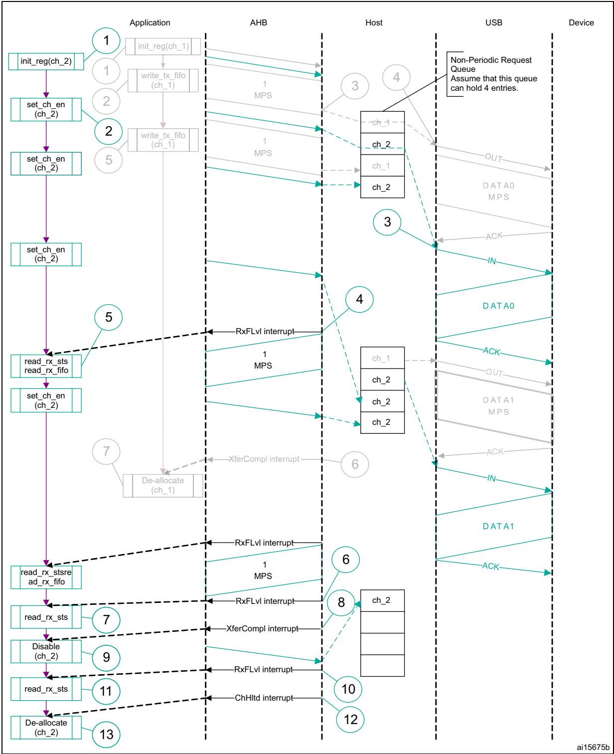
Figure 544. Bulk/control IN transactions
