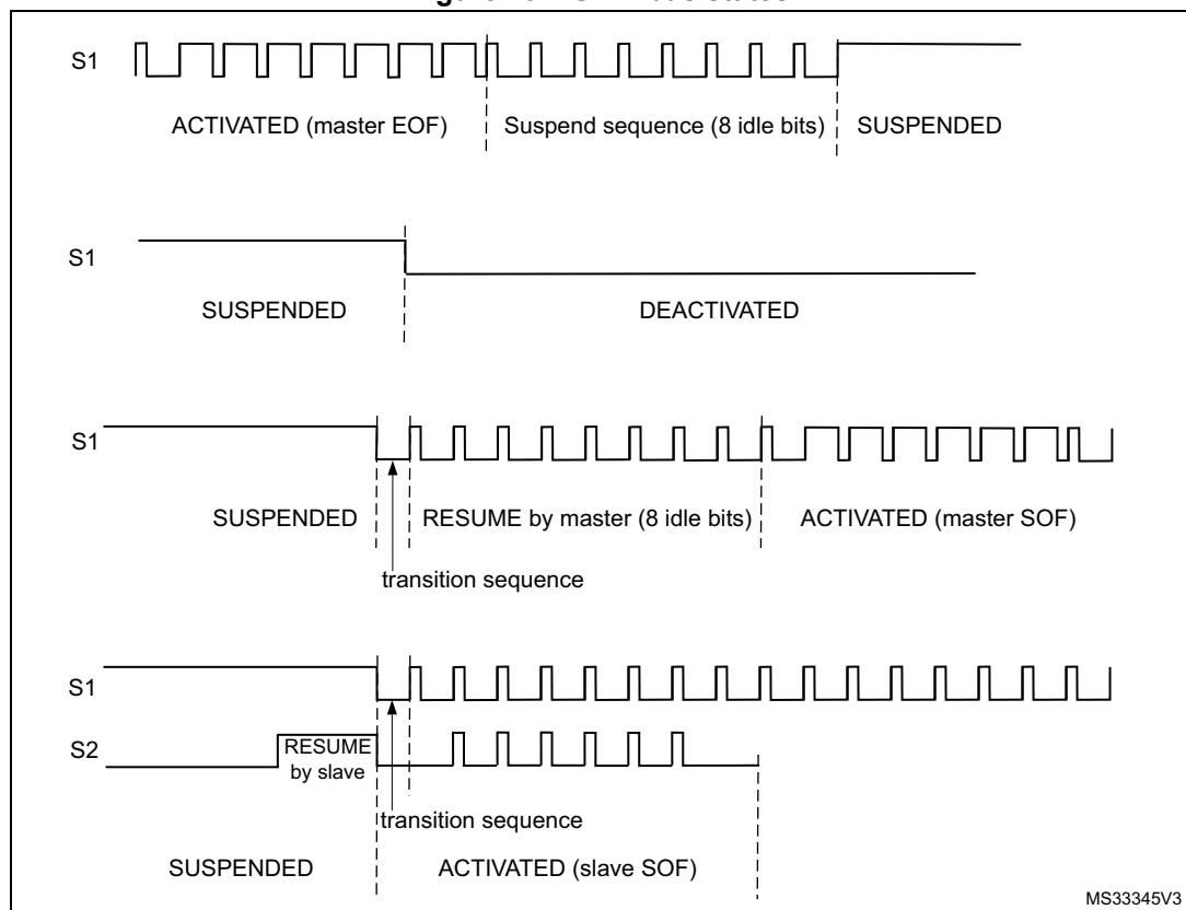
Figure 492. SWP bus states
