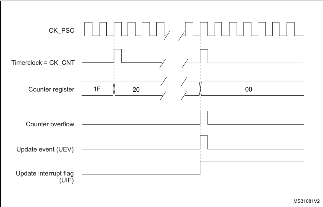
Figure 290. Counter timing diagram, internal clock divided by N
