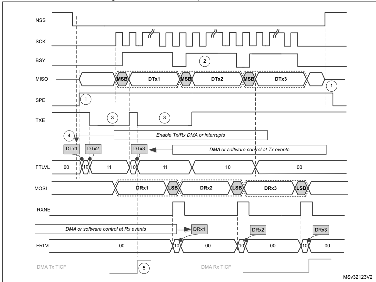
Figure 468. Slave full-duplex communication
