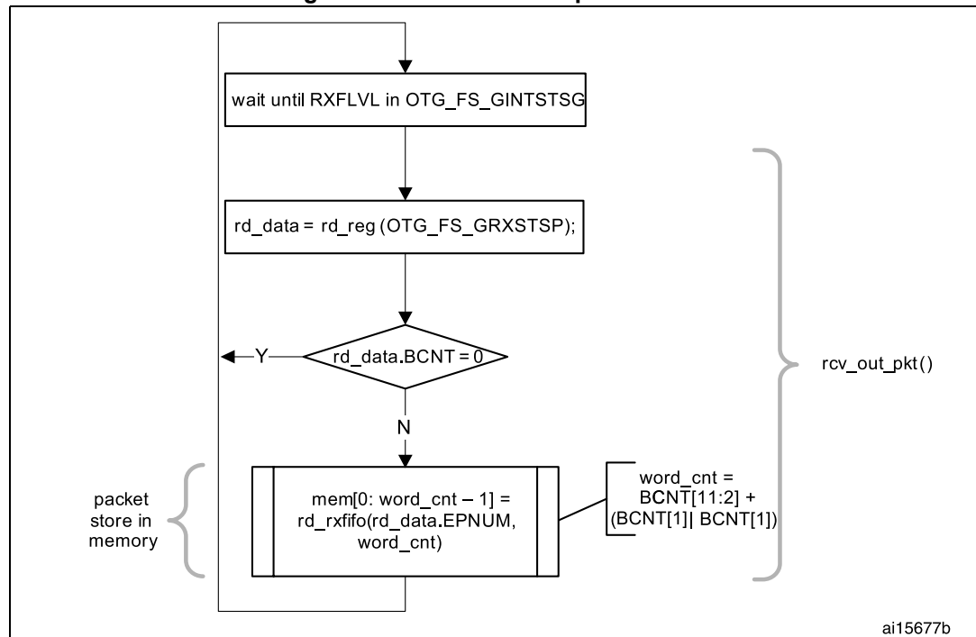
Figure 549. Receive FIFO packet read
