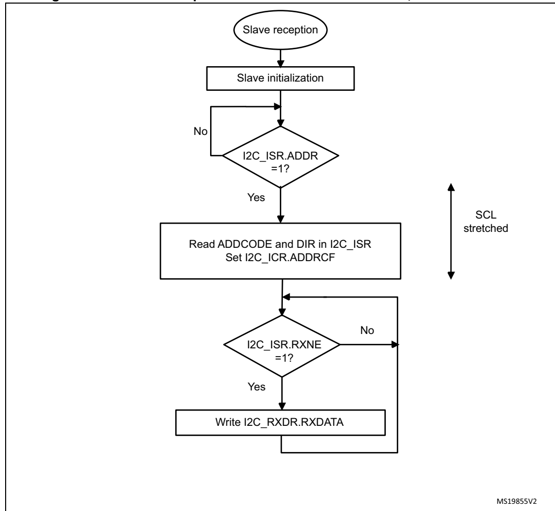
Figure 400. Transfer sequence flow for I2C slave receiver, NOSTRETCH = 0
