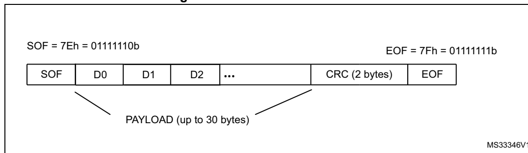
Figure 493. SWP frame structure
