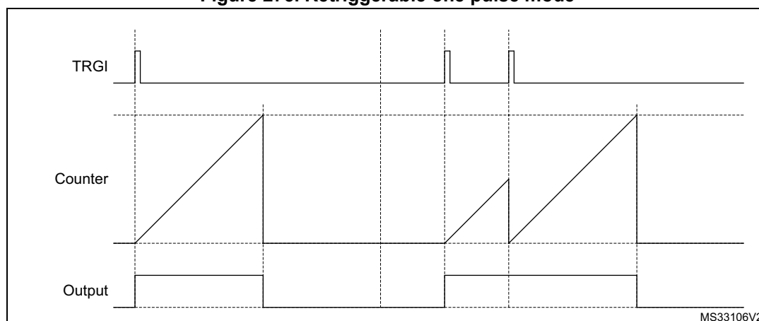
Figure 275. Retriggerable one pulse mode
