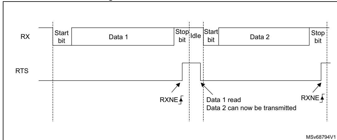
Figure 454. RS232 RTS flow control
