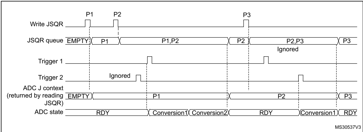
Figure 81. Example of JSQR queue of context (trigger change)
