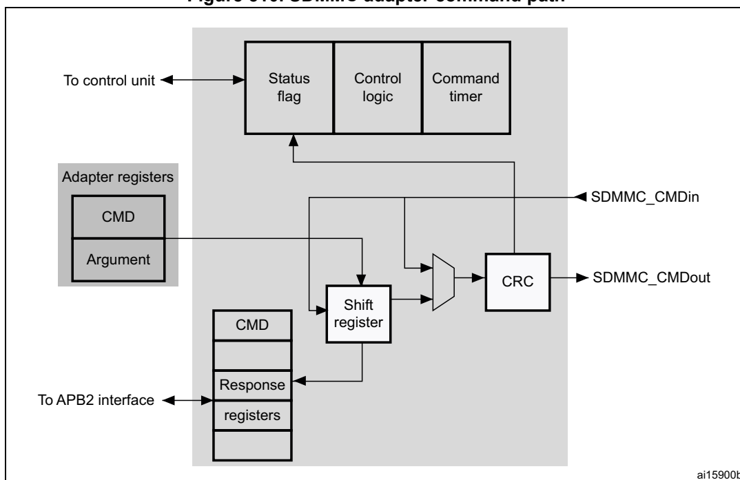
Figure 510. SDMMC adapter command path
