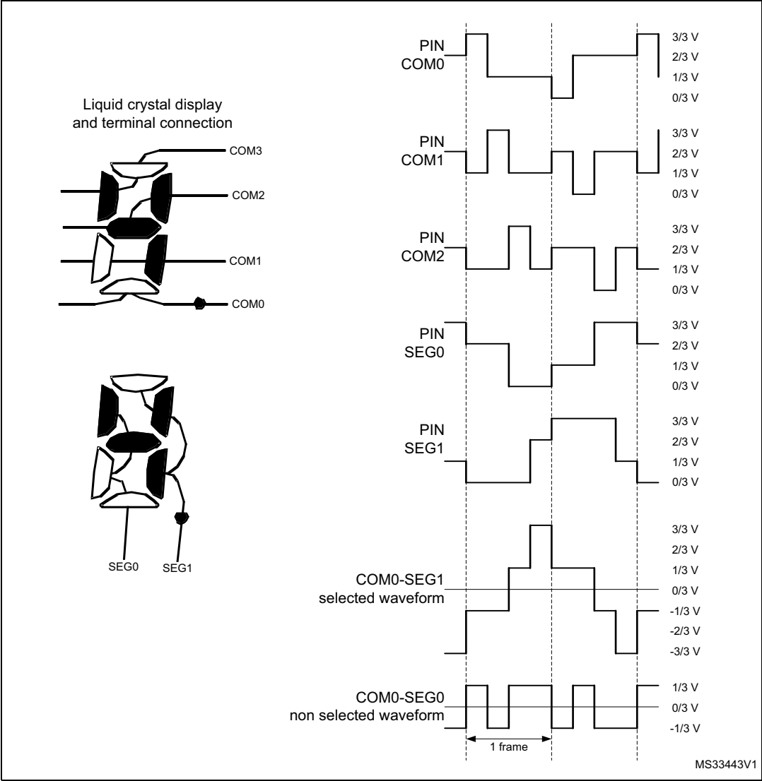
Figure 177. 1/4 duty, 1/3 bias
