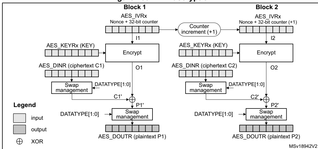
Figure 209. CTR decryption
