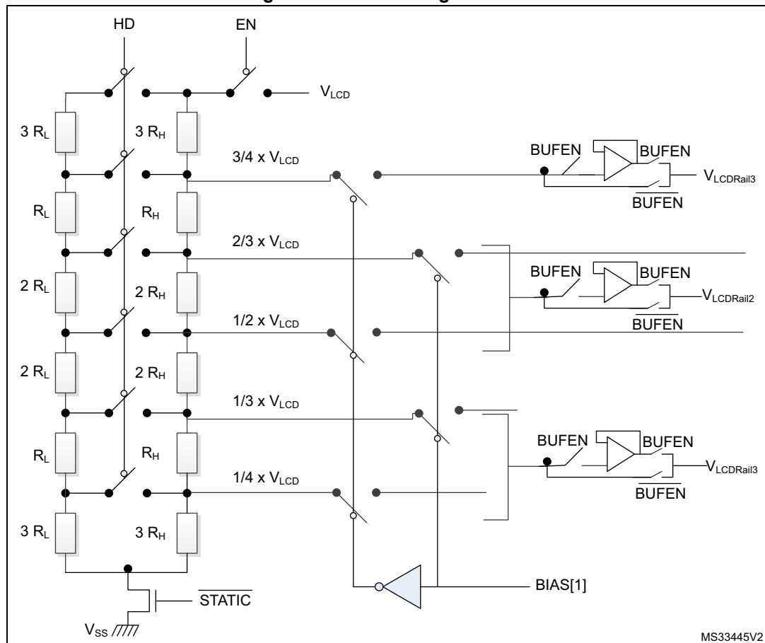
Figure 179. LCD voltage control
