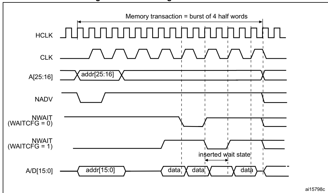
Figure 54. Synchronous multiplexed read mode waveforms - NOR, PSRAM (CRAM)
