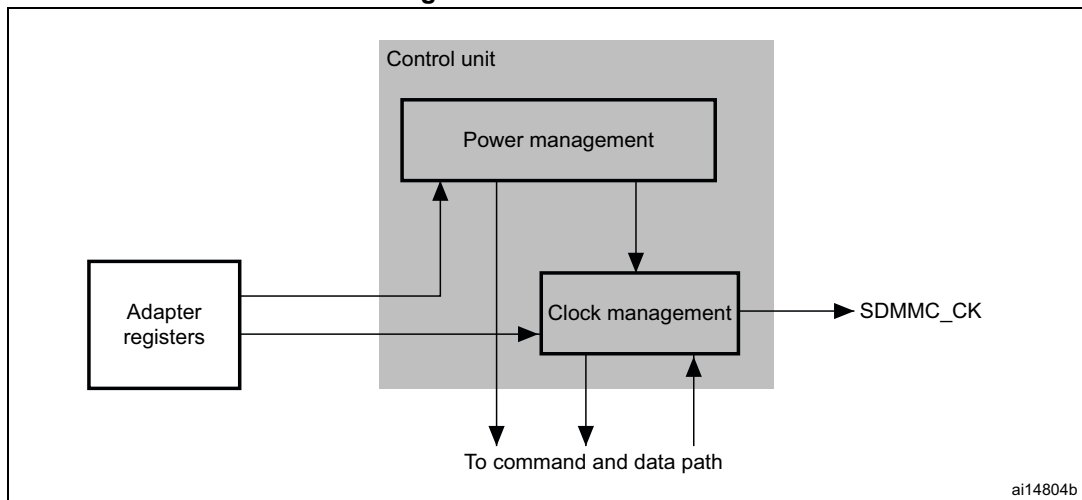
Figure 508. Control unit
