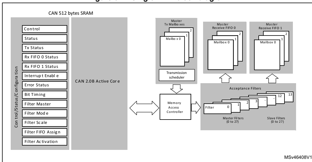
Figure 517. Single-CAN block diagram
