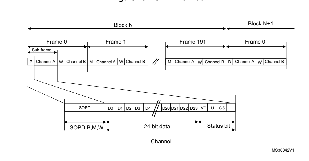
Figure 482. SPDIF format
