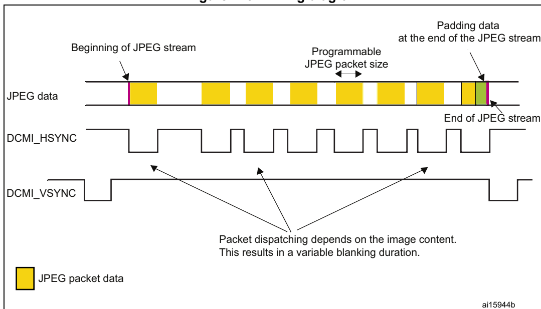
Figure 149. Timing diagram
