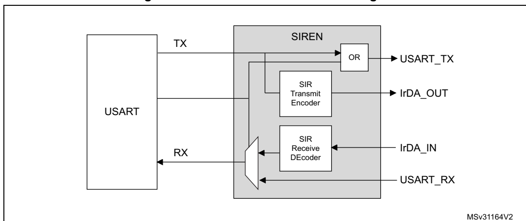
Figure 437. IrDA SIR ENDEC- block diagram
