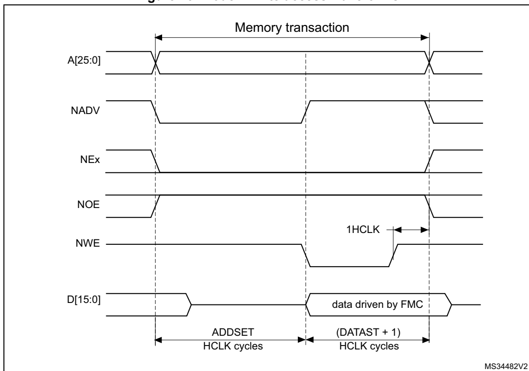
Figure 43. Mode 2 write access waveforms
