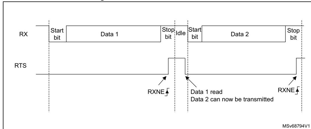
Figure 442. RS232 RTS flow control
