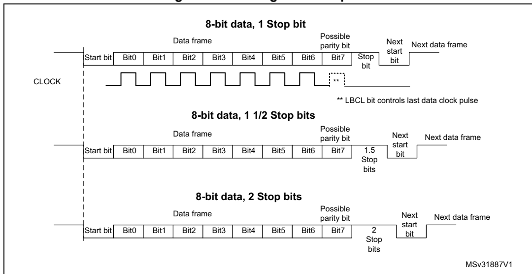
Figure 422. Configurable stop bits
