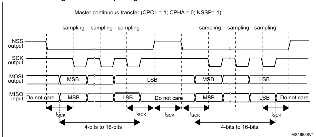
Figure 471. NSSP pulse generation in Motorola SPI master mode
