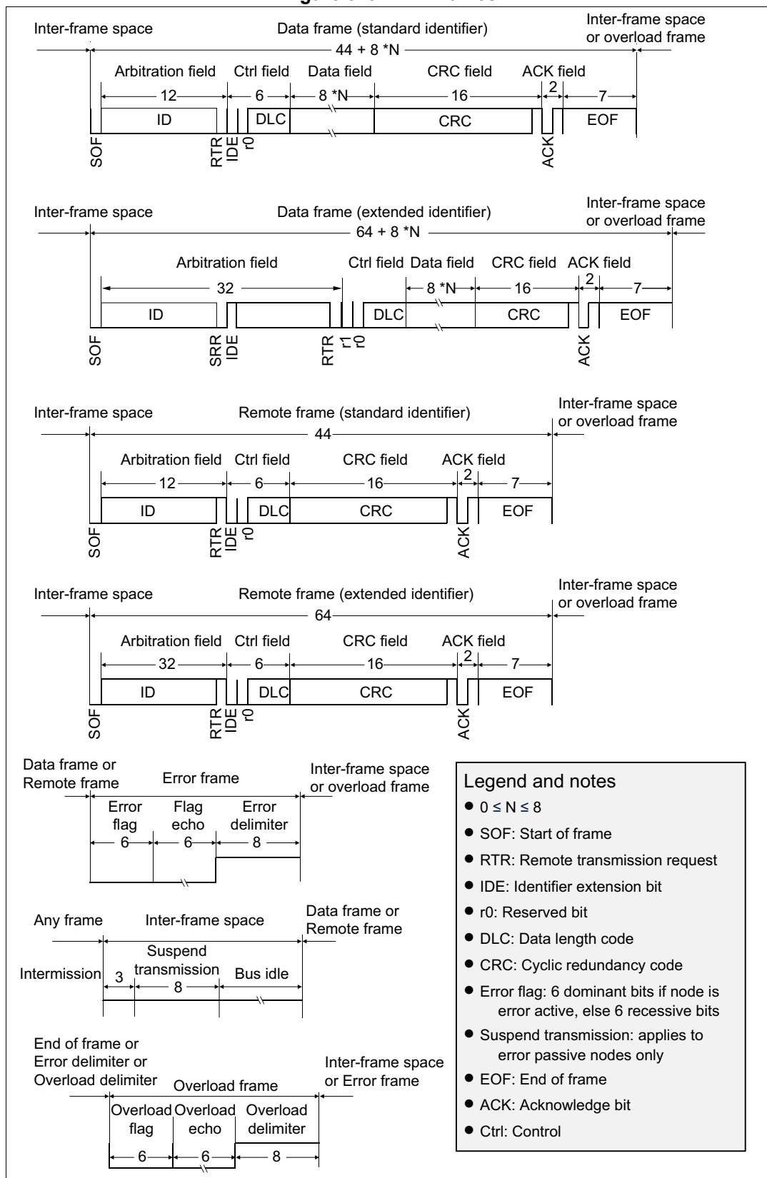
Figure 529. CAN frames
