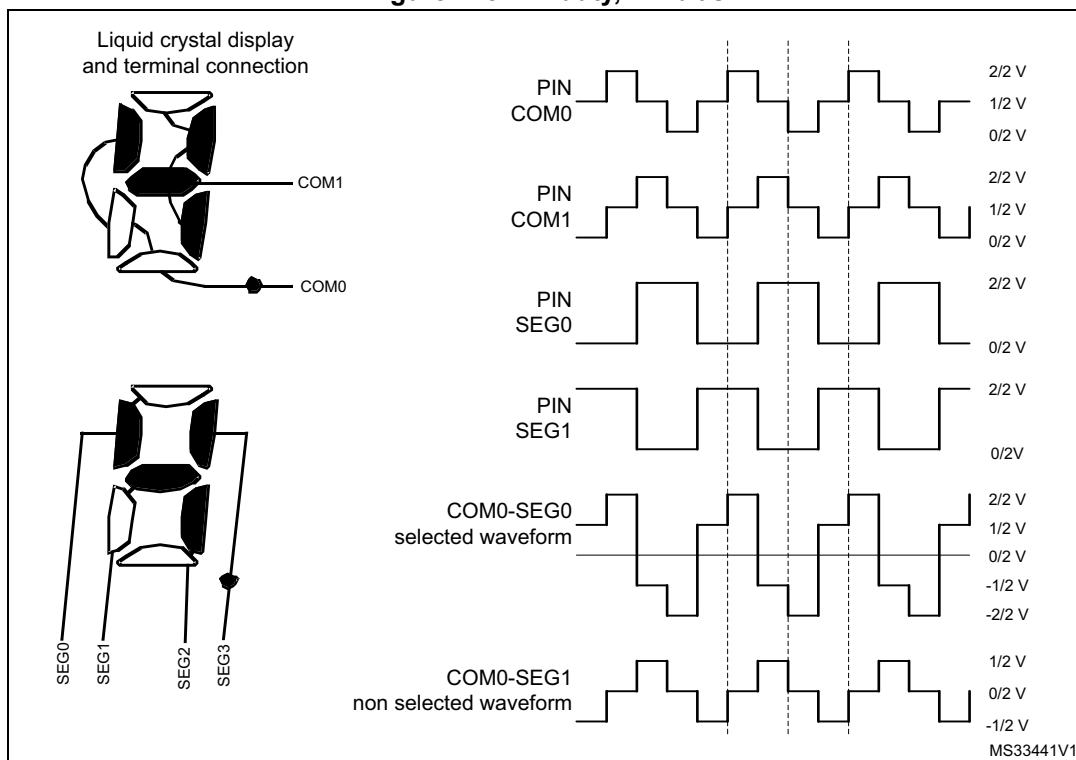
Figure 175. 1/2 duty, 1/2 bias
