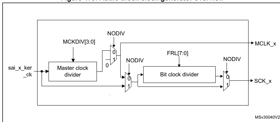
Figure 479. Audio block clock generator overview
