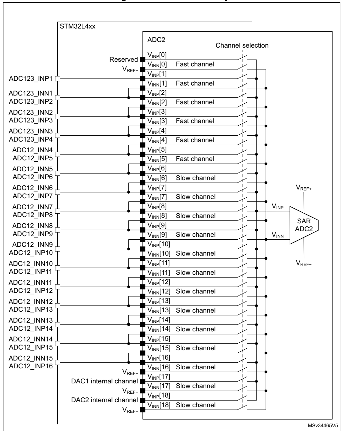
Figure 69. ADC2 connectivity
