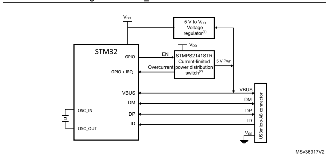
Figure 533. OTG_FS A-B device connection
