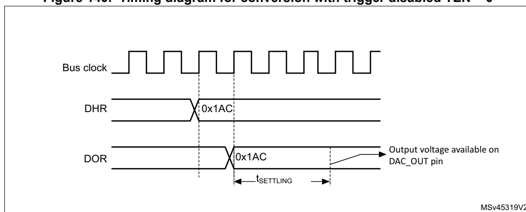
Figure 140. Timing diagram for conversion with trigger disabled TEN = 0
