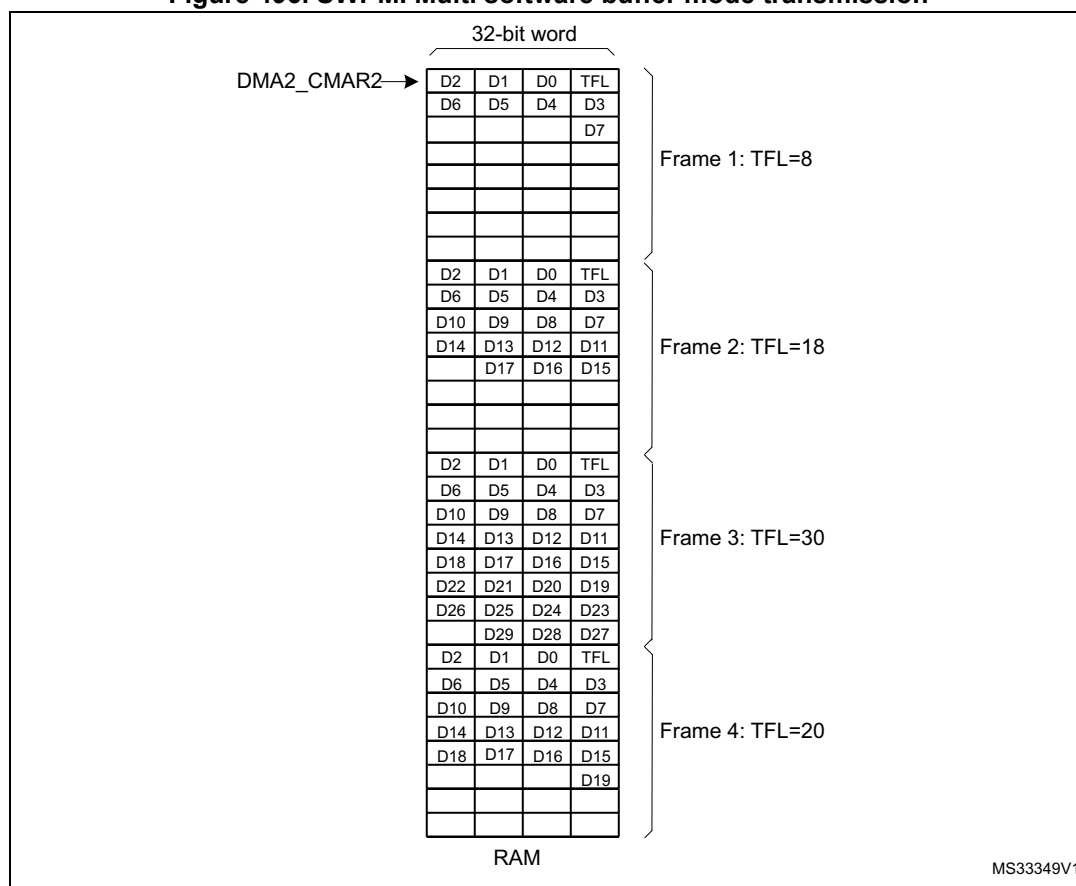
Figure 496. SWPMI Multi software buffer mode transmission
