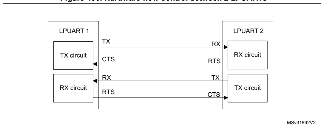
Figure 453. Hardware flow control between 2 LPUARTs
