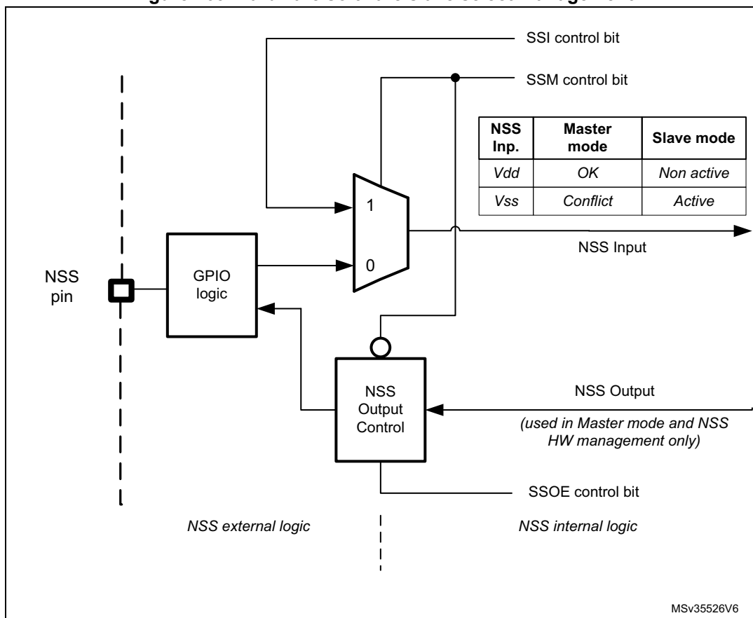
Figure 463. Hardware/software slave select management
