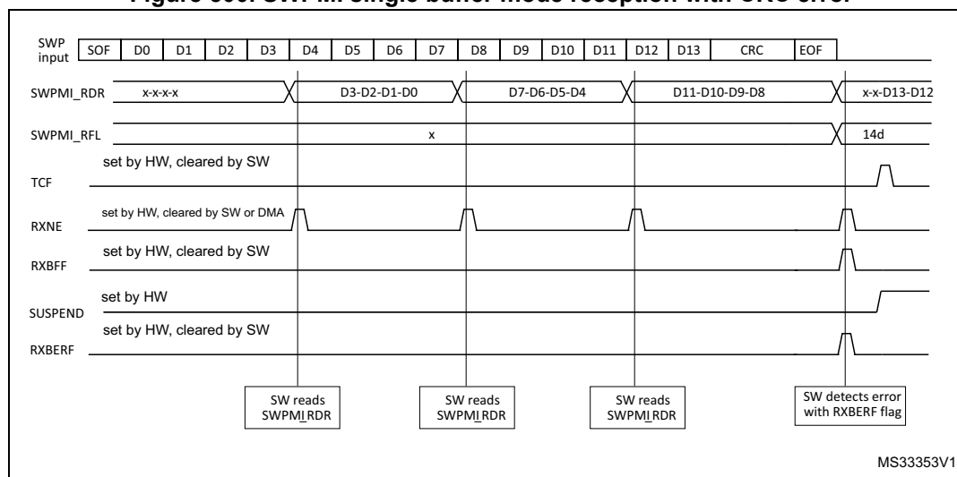
Figure 500. SWPMI single buffer mode reception with CRC error
