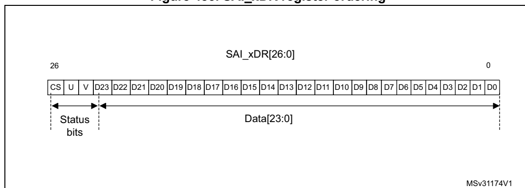
Figure 483. SAI_xDR register ordering
