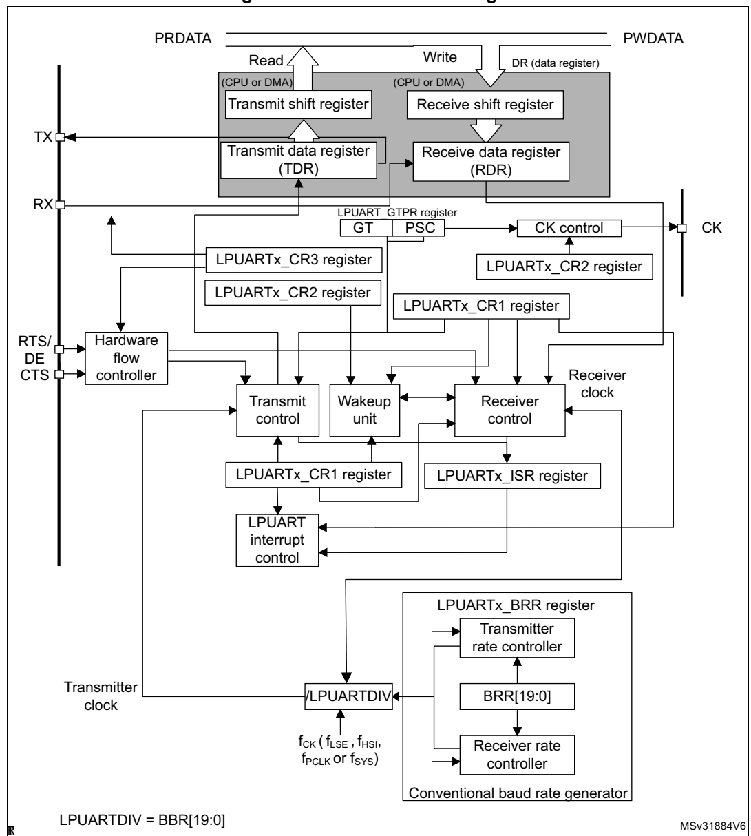
Figure 445. LPUART block diagram
