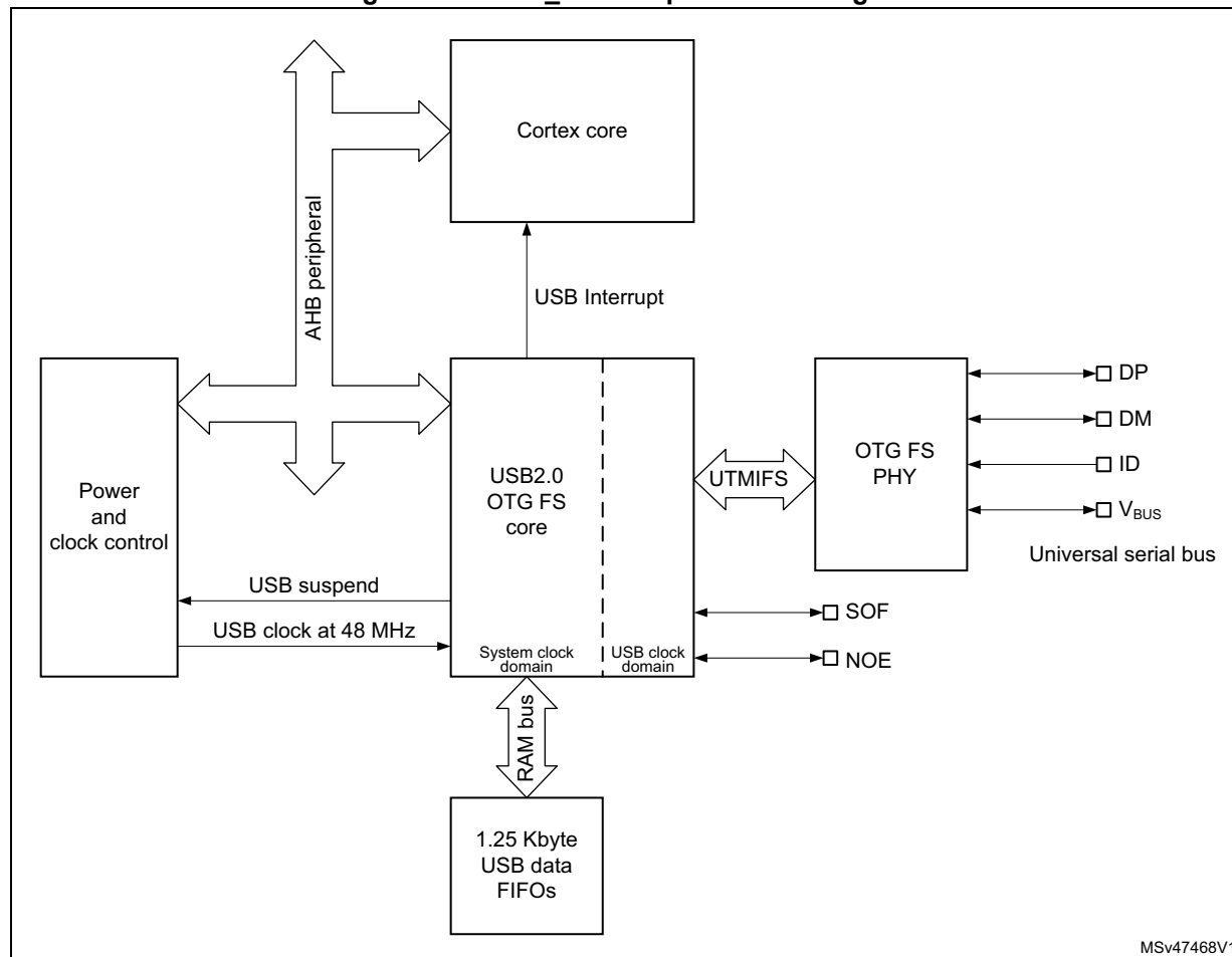
Figure 532. OTG_FS full-speed block diagram
