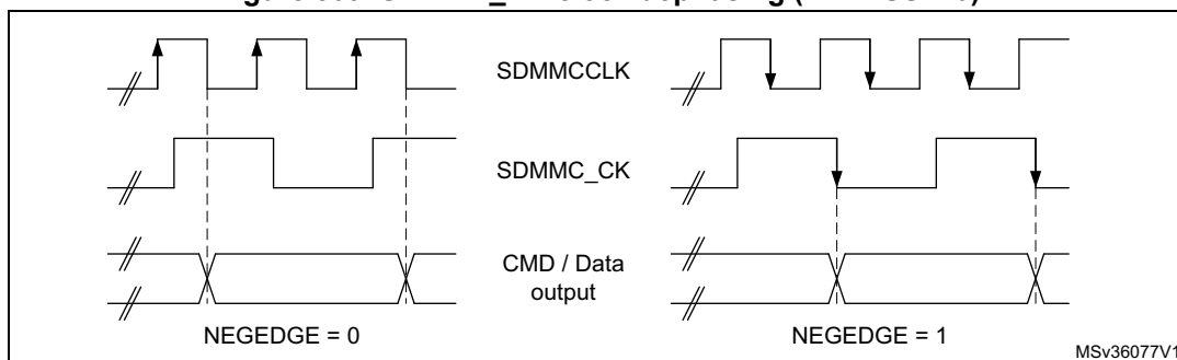
Figure 509. SDMMC_CLK clock dephasing (BYPASS = 0)
