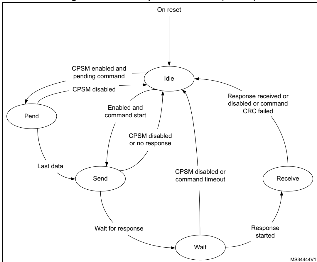
Figure 511. Command path state machine (SDMMC)
