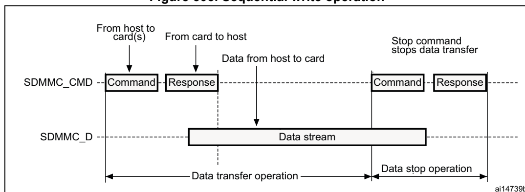
Figure 505. Sequential write operation
