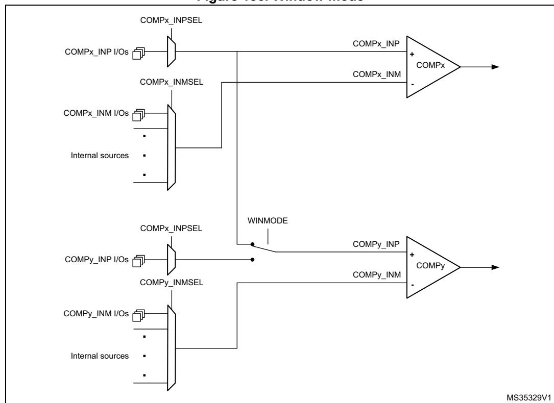
Figure 156. Window mode
