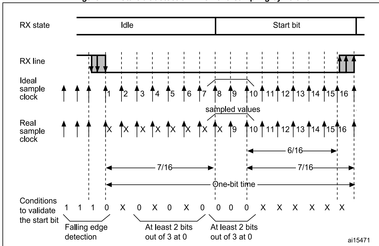
Figure 424. Start bit detection when oversampling by 16 or 8
