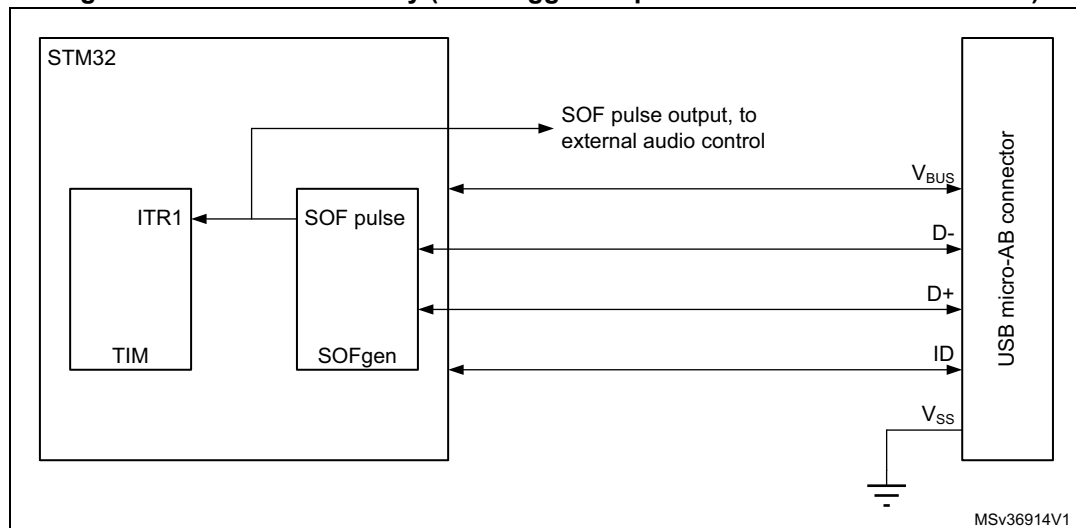
Figure 536. SOF connectivity (SOF trigger output to TIM and ITR1 connection)
