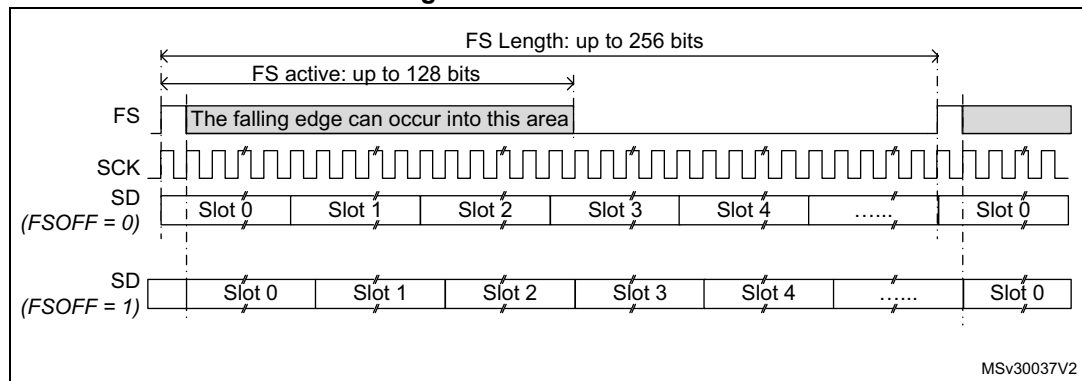
Figure 474. Audio frame
