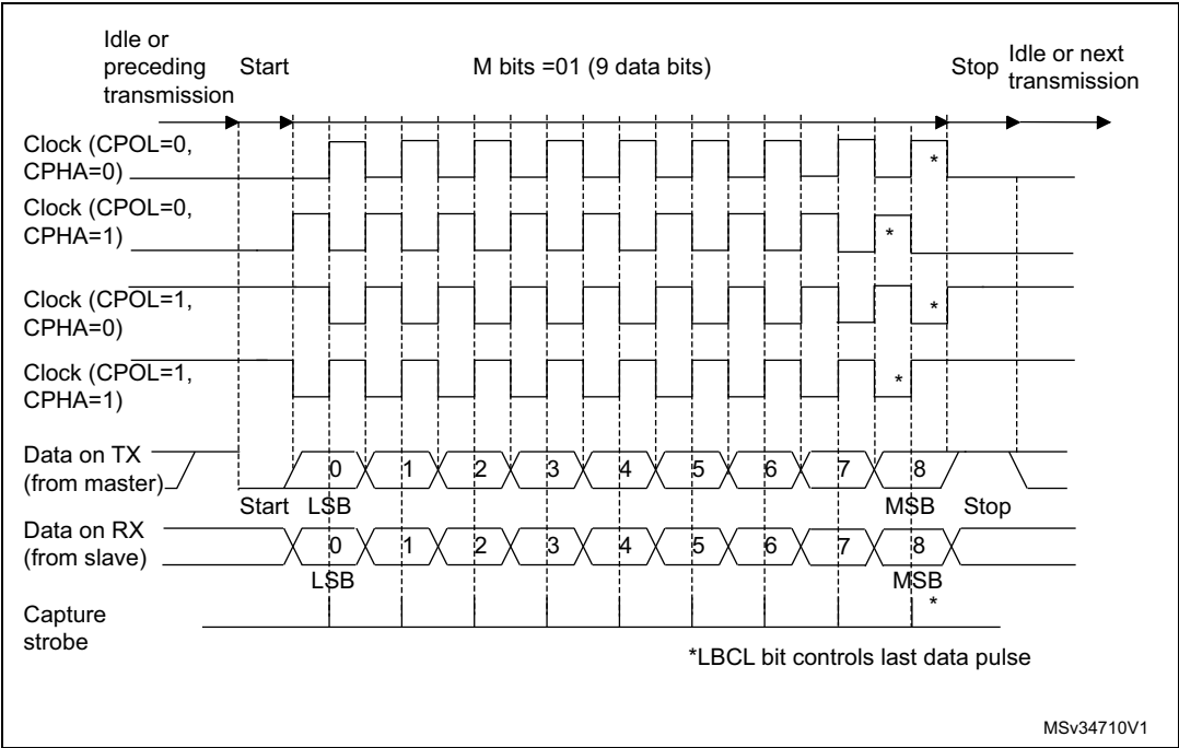
Figure 433. USART data clock timing diagram (M bits = 01)
