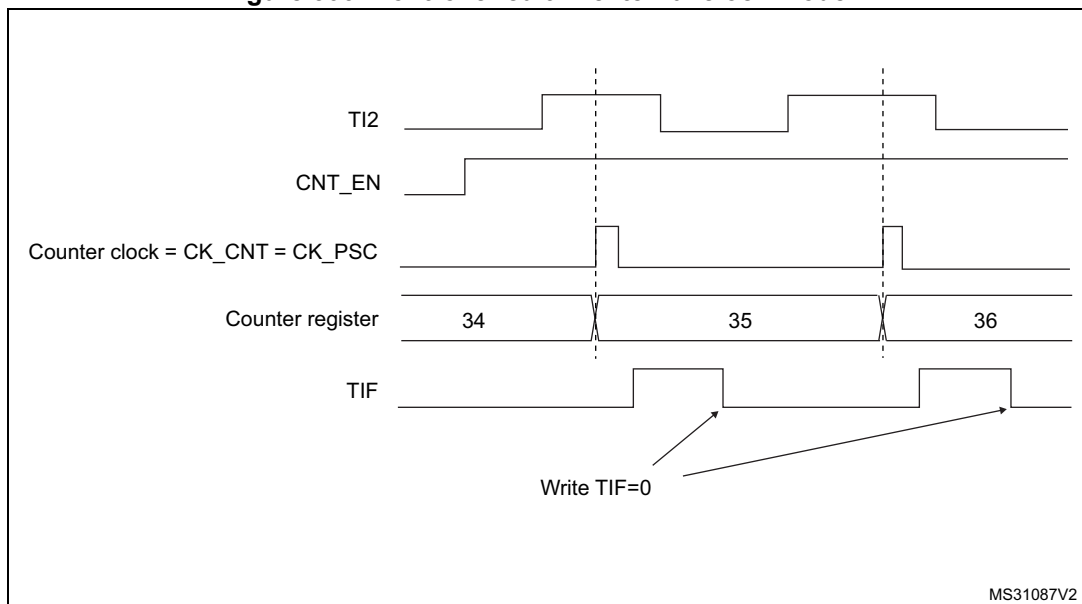
Figure 306. Control circuit in external clock mode 1
