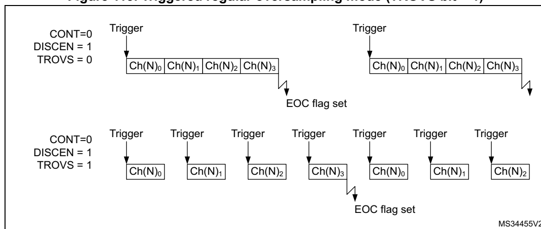
Figure 113. Triggered regular oversampling mode (TROVS bit = 1)
