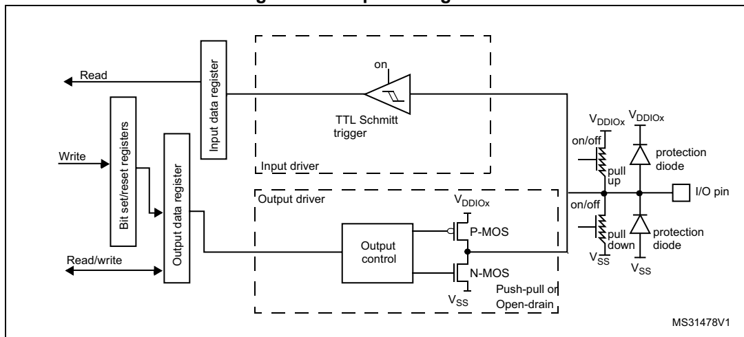
Figure 26. Output configuration
