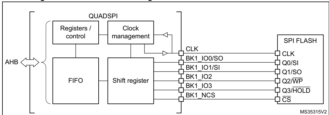
Figure 58. QUADSPI block diagram when dual-flash mode is disabled
