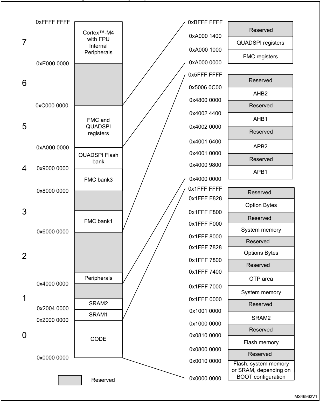
Figure 4. Memory map for STM32L49x/L4Ax devices
