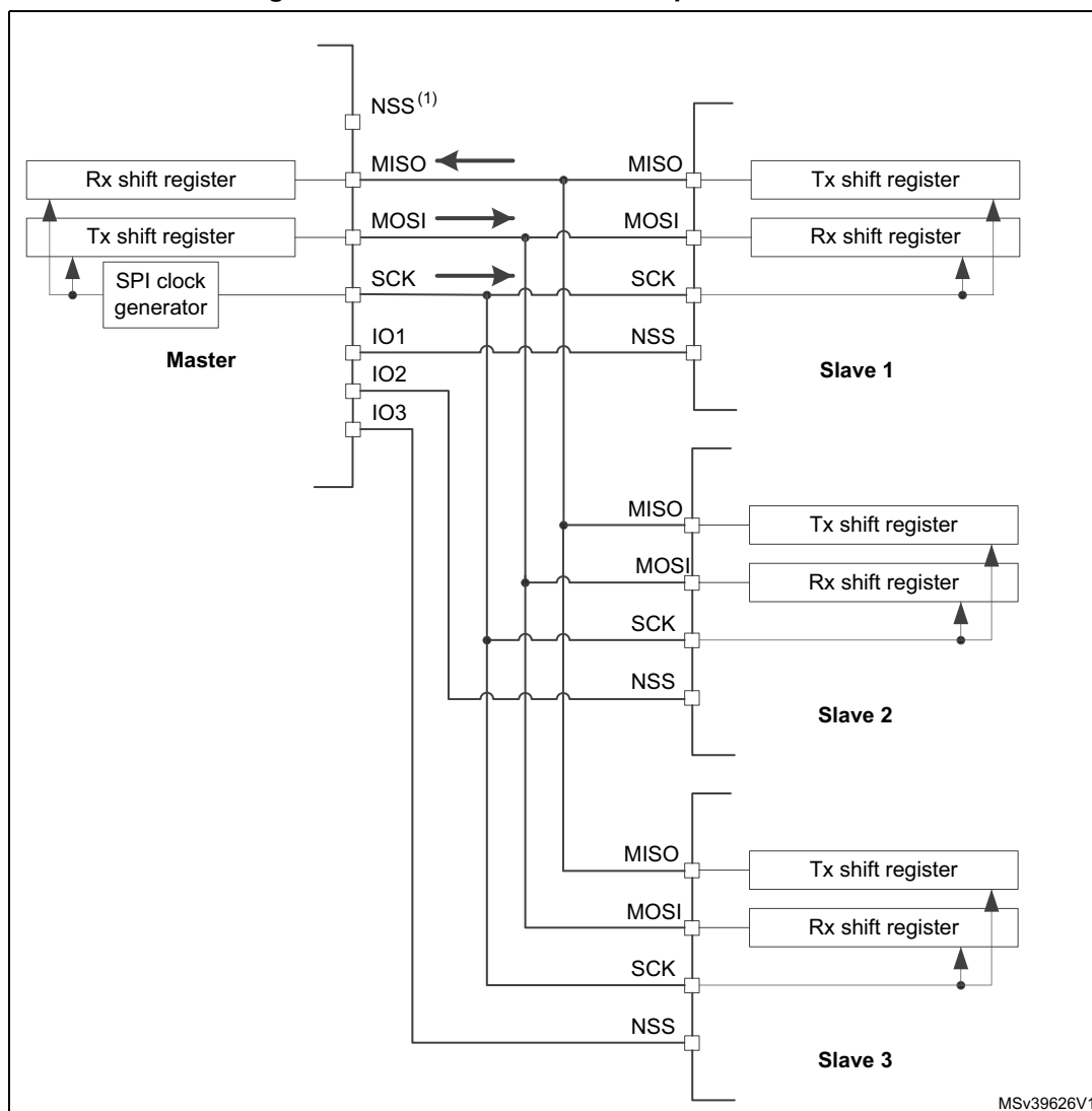
Figure 461. Master and three independent slaves
