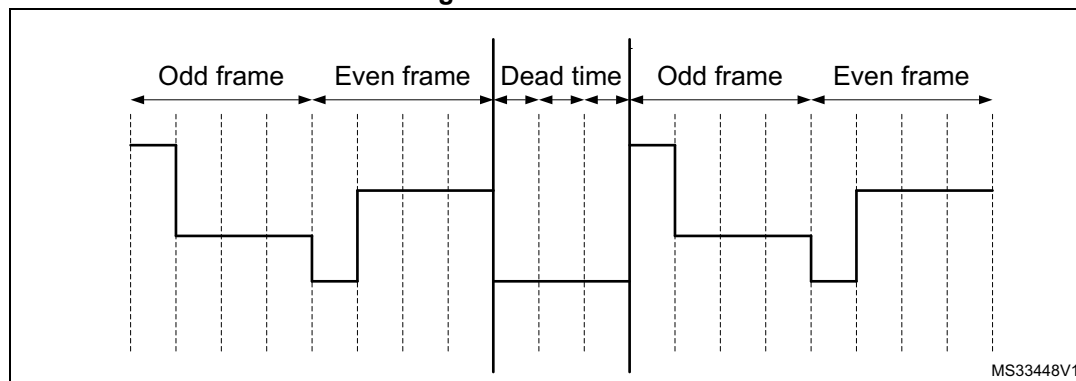
Figure 180. Deadtime
