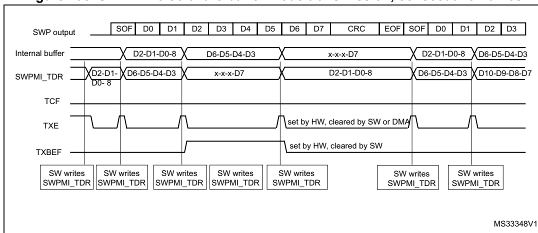
Figure 495. SWPMI No software buffer mode transmission, consecutive frames
