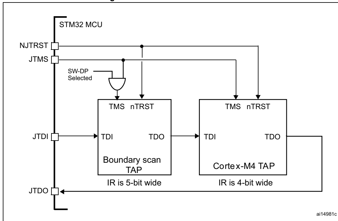
Figure 559. JTAG TAP connections
