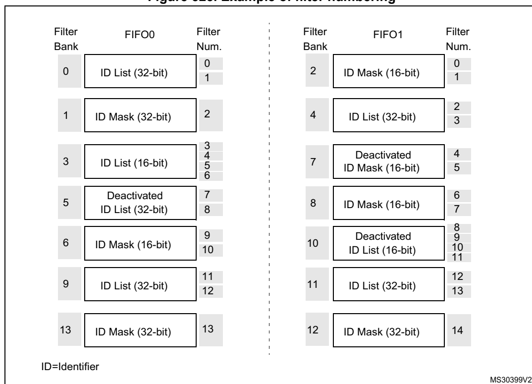
Figure 525. Example of filter numbering
