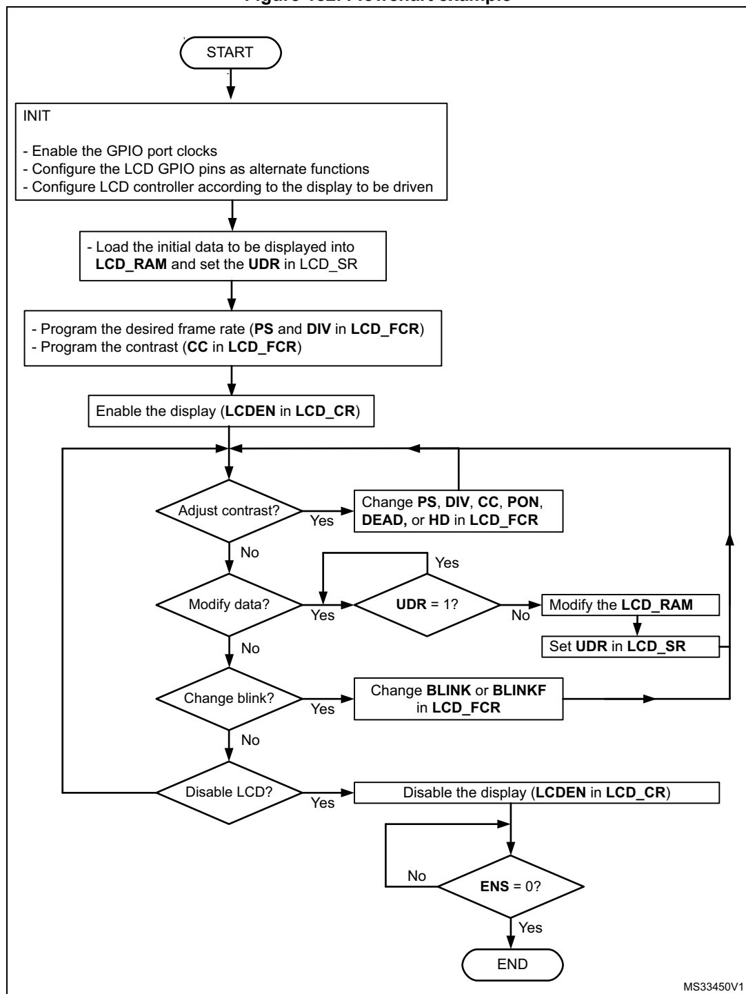
Figure 182. Flowchart example
