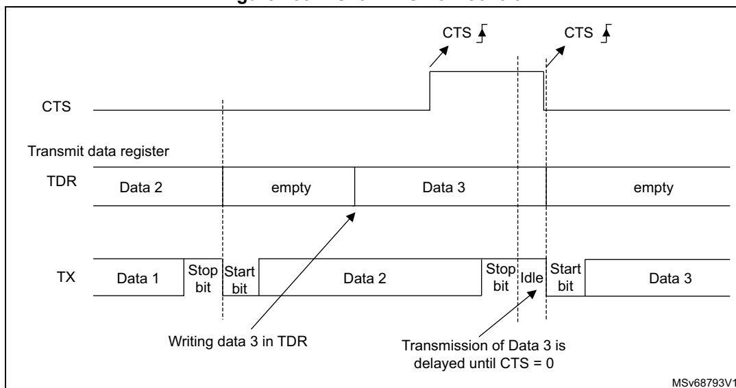
Figure 455. RS232 CTS flow control
