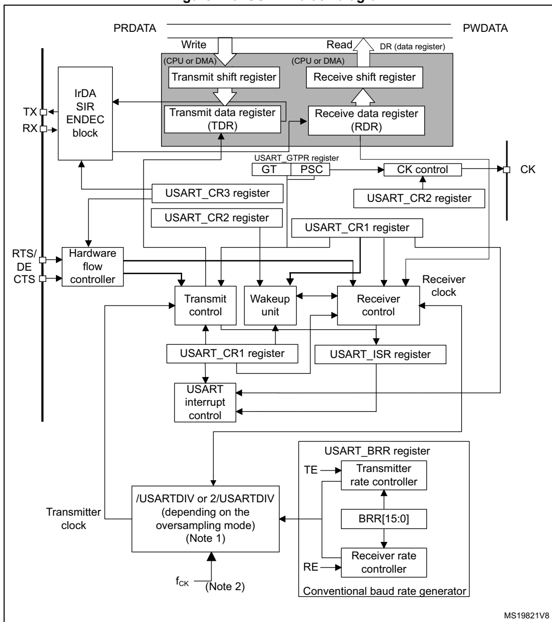
Figure 420. USART block diagram
