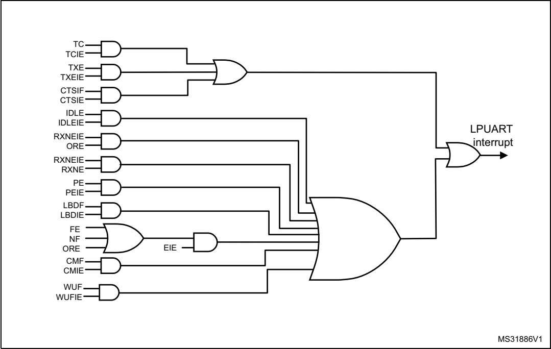
Figure 456. LPUART interrupt mapping diagram
