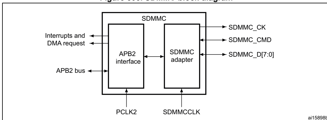
Figure 506. SDMMC block diagram
