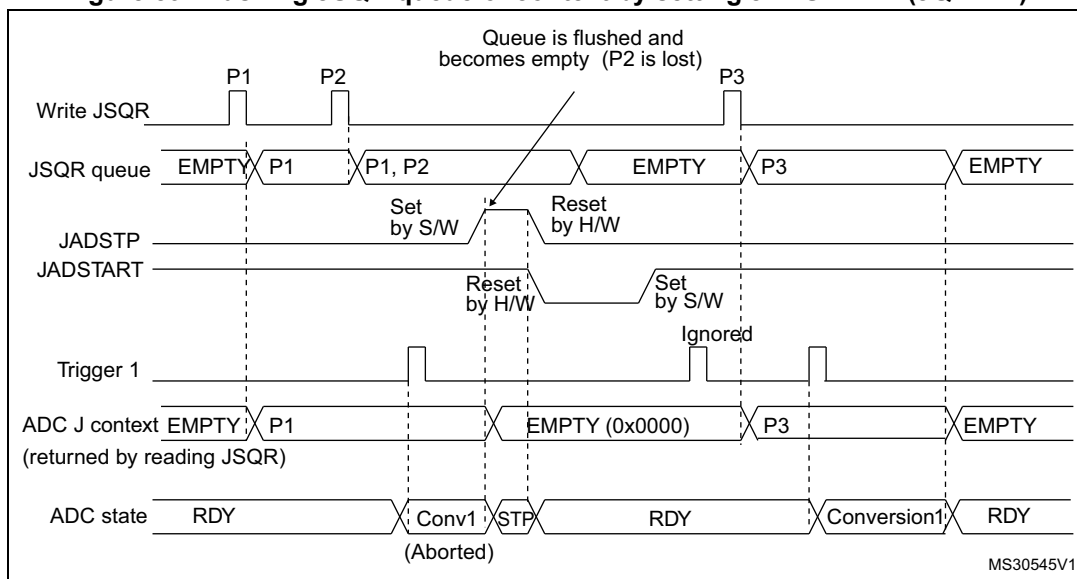
Figure 89. Flushing JSQR queue of context by setting JADSTP = 1 (JQM = 1)
