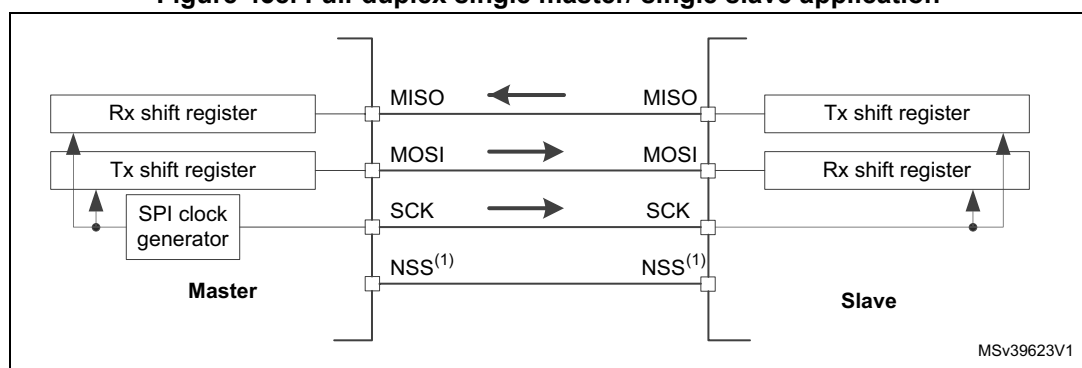
Figure 458. Full-duplex single master/ single slave application
