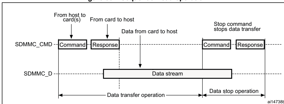
Figure 504. Sequential read operation
