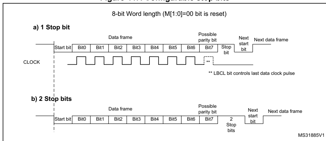
Figure 447. Configurable stop bits
