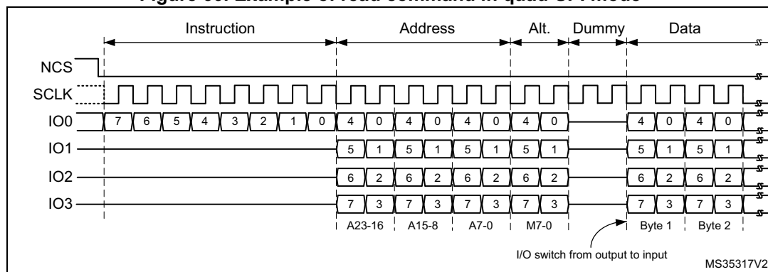
Figure 60. Example of read command in quad-SPI mode
