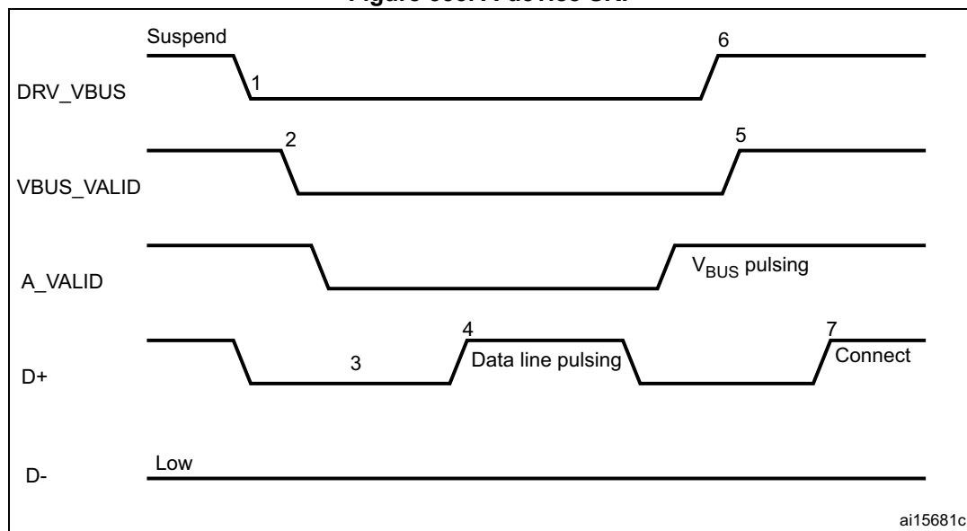
Figure 553. A-device SRP
