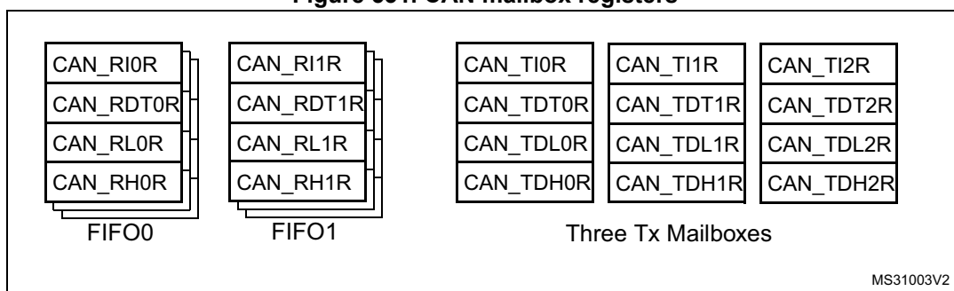
Figure 531. CAN mailbox registers
