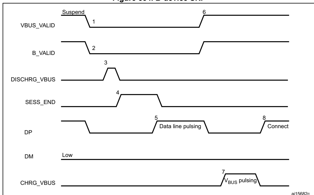
Figure 554. B-device SRP
