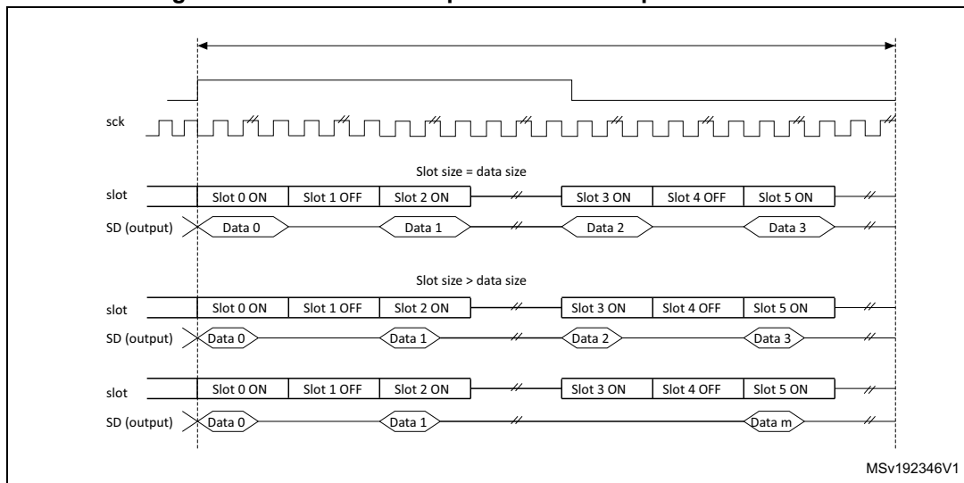
Figure 486. Tristate on output data line in a protocol like I2S
