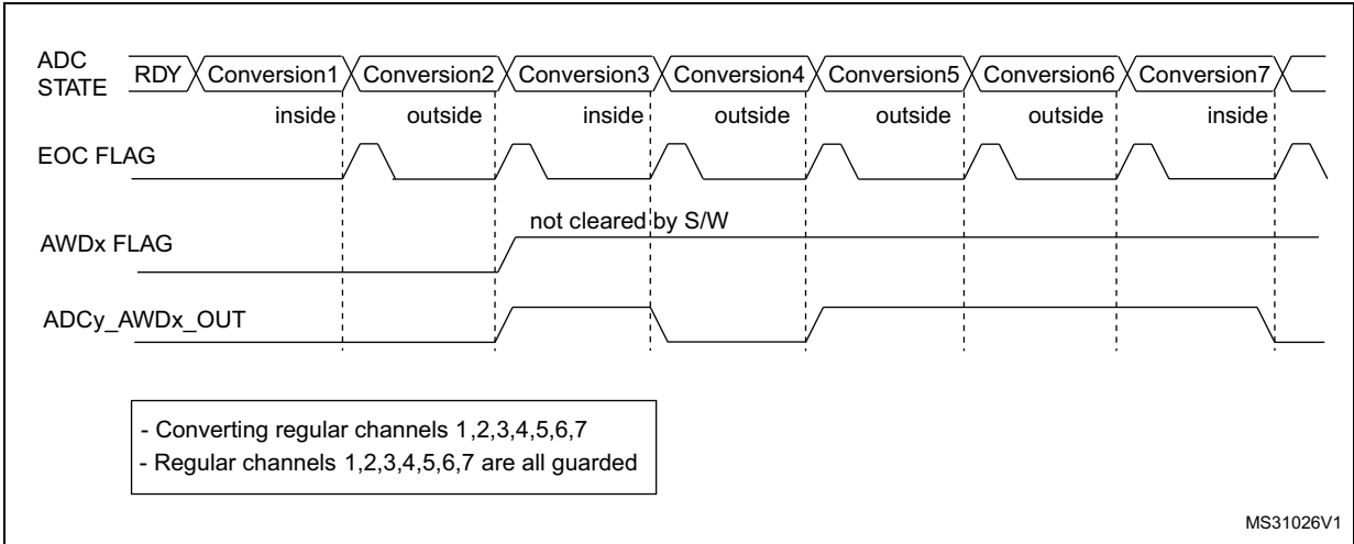
Figure 108. ADCy_AWDx_OUT signal generation (AWDx flag not cleared by software)
