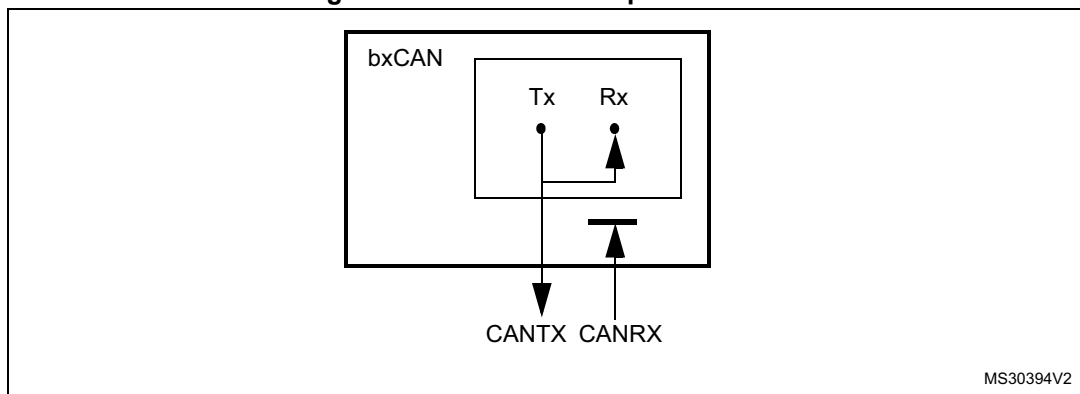
Figure 520. bxCAN in Loop back mode
