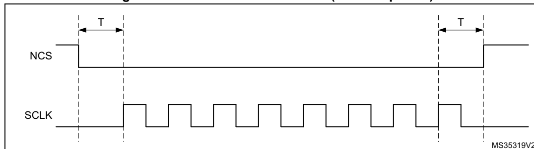
Figure 62. NCS when CKMODE = 0 (T = CLK period)
