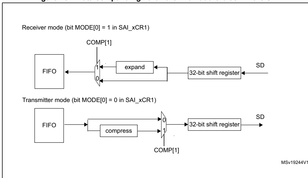
Figure 484. Data companding hardware in an audio block in the SAI
