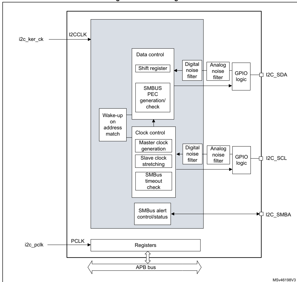
Figure 390. Block diagram
