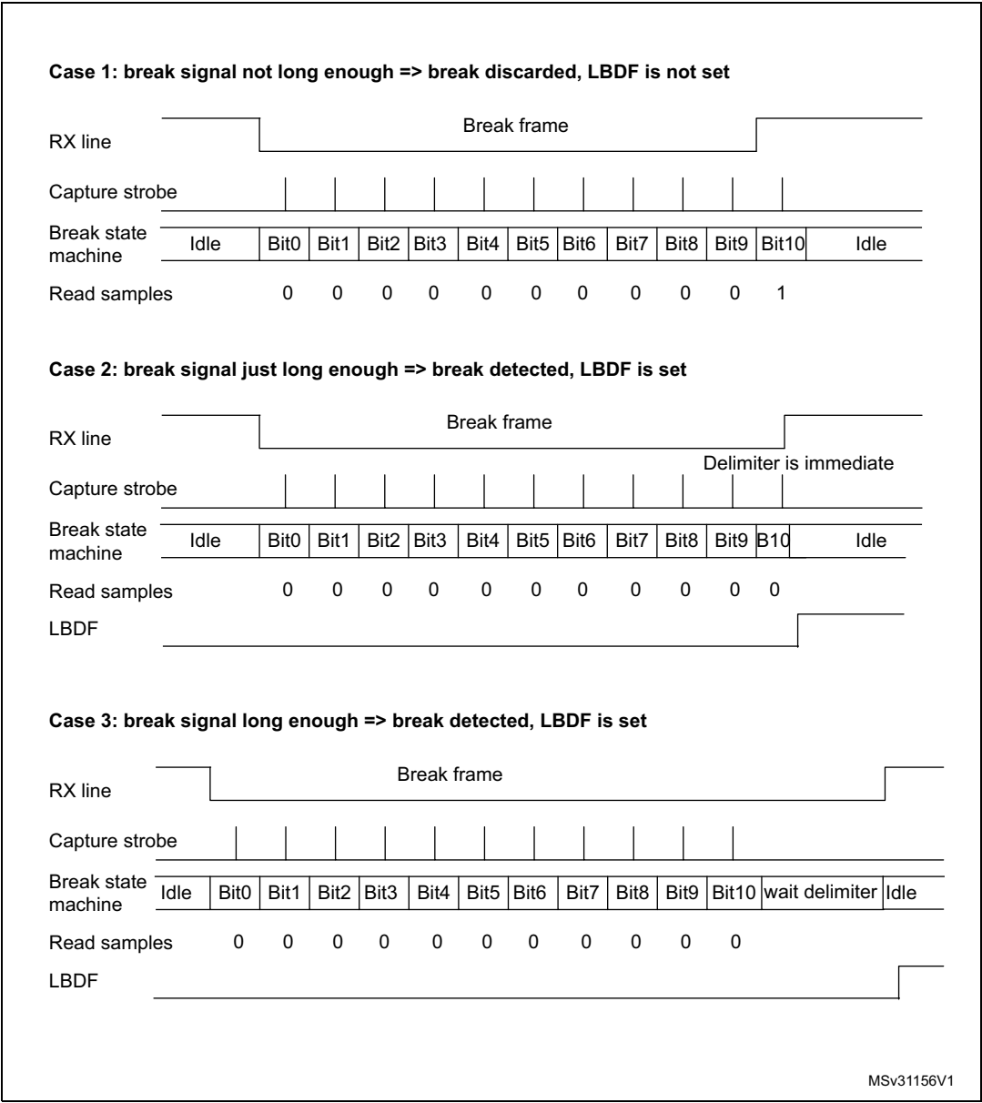
Figure 429. Break detection in LIN mode (11-bit break length - LBDL bit is set)
