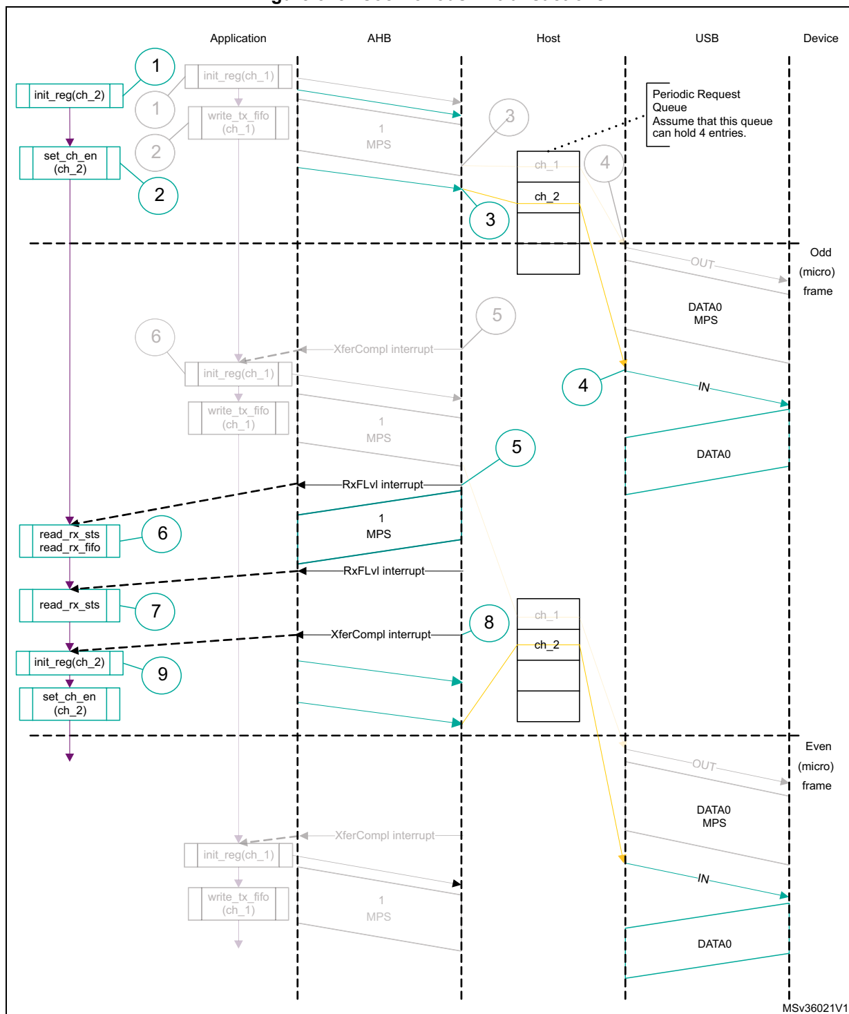
Figure 548. Isochronous IN transactions
