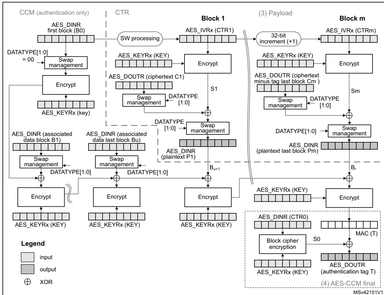
Figure 215. CCM mode authenticated decryption
