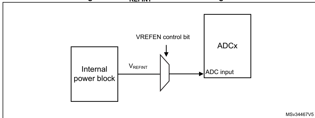
Figure 136. V_{REFINT} channel block diagram
