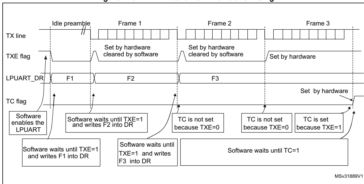
Figure 448. TC/TXE behavior when transmitting
