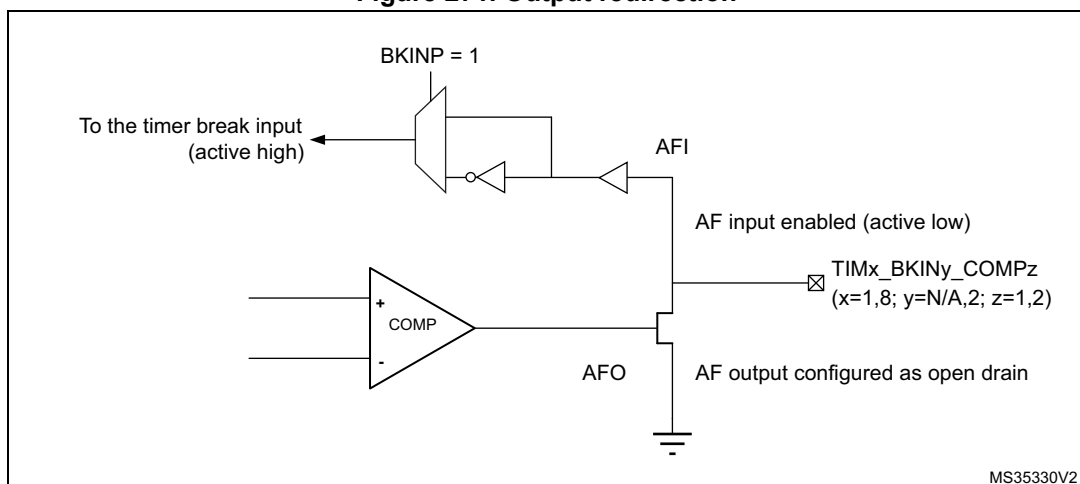
Figure 271. Output redirection
