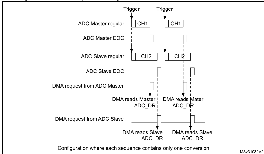
Figure 131. DMA Requests in regular simultaneous mode when MDMA = 00
