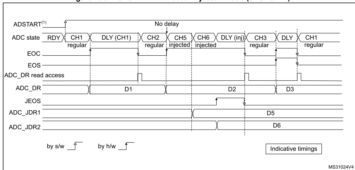
Figure 105. AUTODLY = 1 in auto-injected mode (JAUTO = 1)
