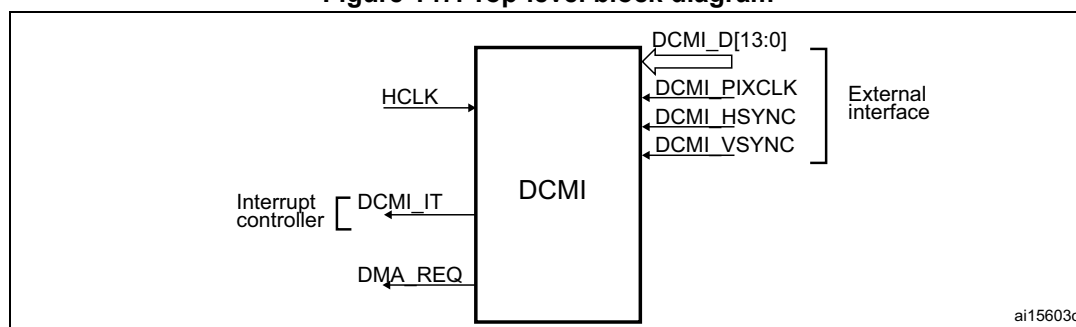
Figure 147. Top-level block diagram
