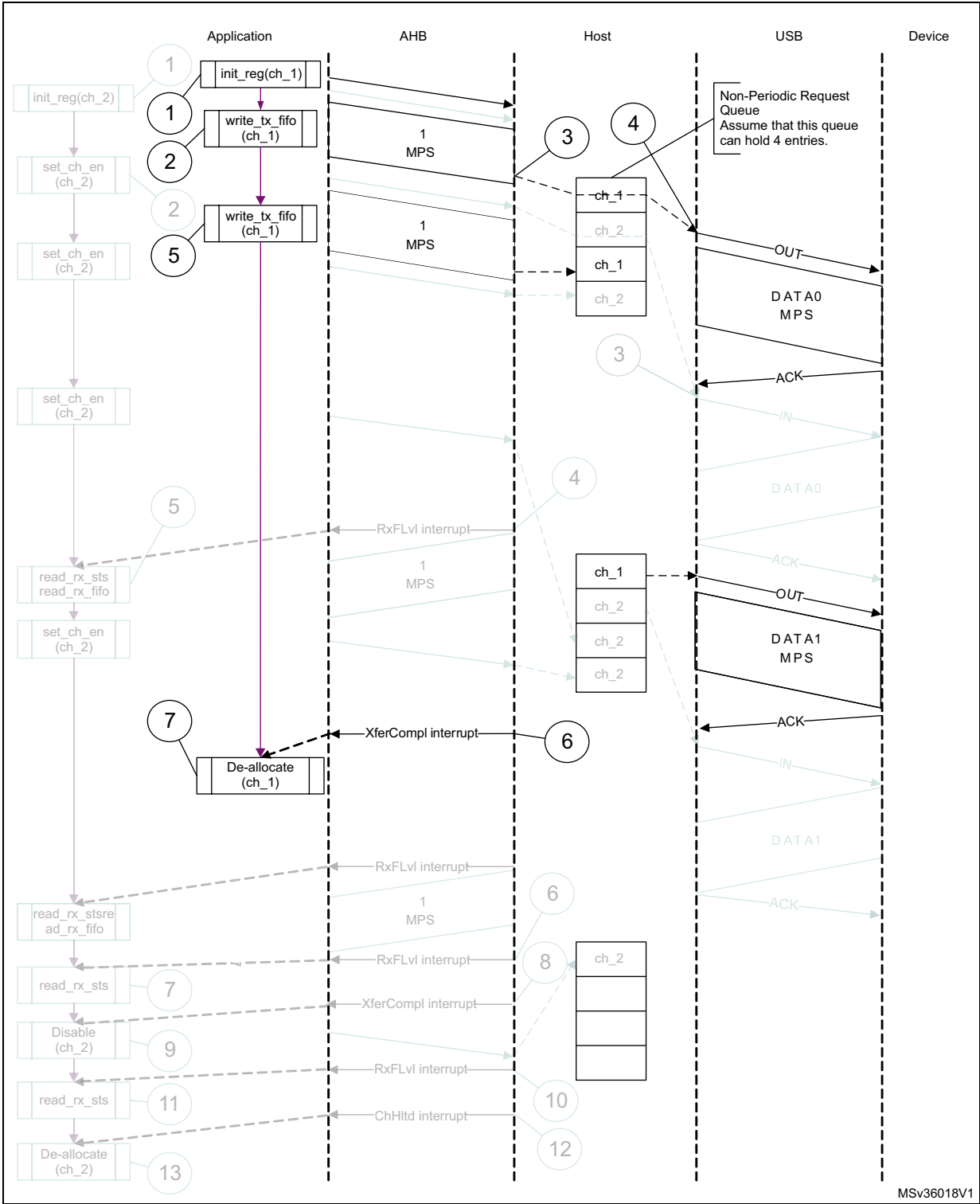
Figure 543. Normal bulk/control OUT/SETUP
