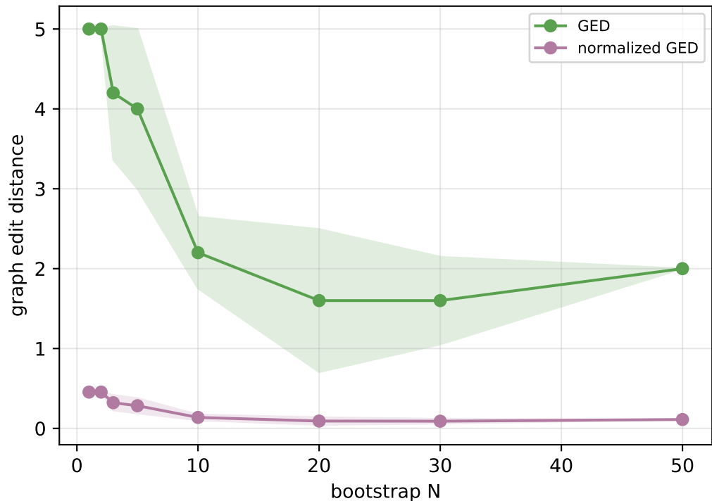
GED vs bootstrap N (lower = better)
