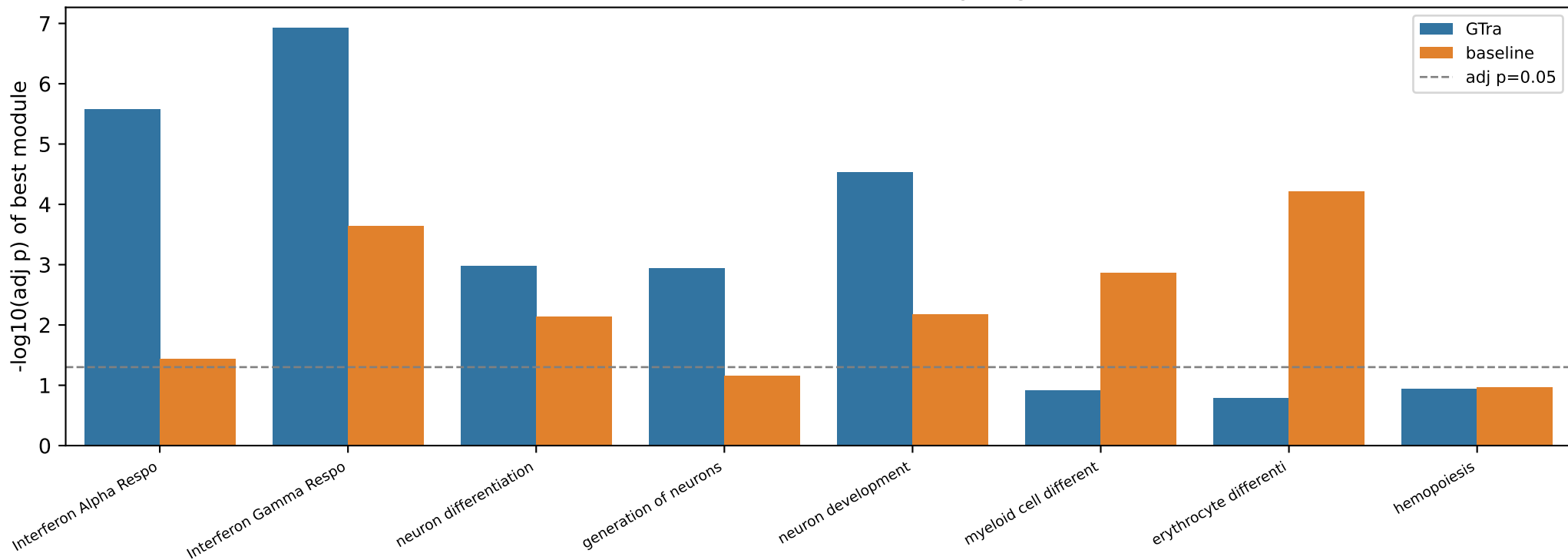
Known biological-program recovery (best module, size-capped 60 genes) GTra wins COVID+MND; HSPC confounded by large GTra modules
