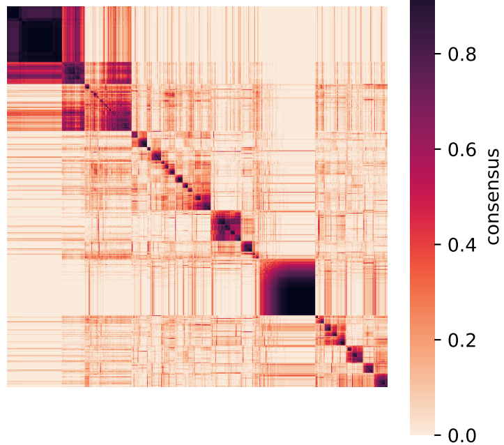
annotation | tp13 | cluster 0 PAC=0.275
