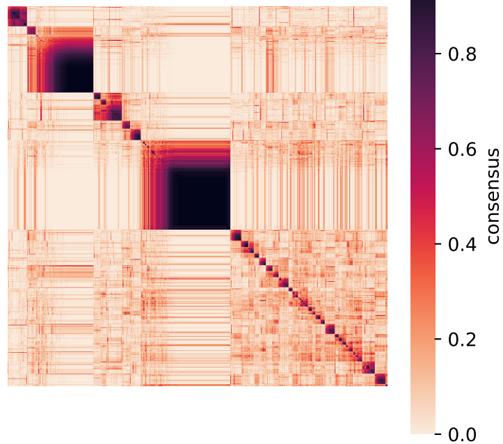
annotation | tp17 | cluster 0 PAC=0.275
