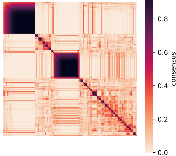
annotation | tp15 | cluster 0 PAC=0.277
