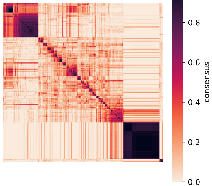
annotation | tp11 | cluster 0 PAC=0.343
