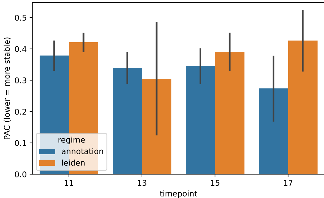
Gene-module ambiguity across bootstraps
