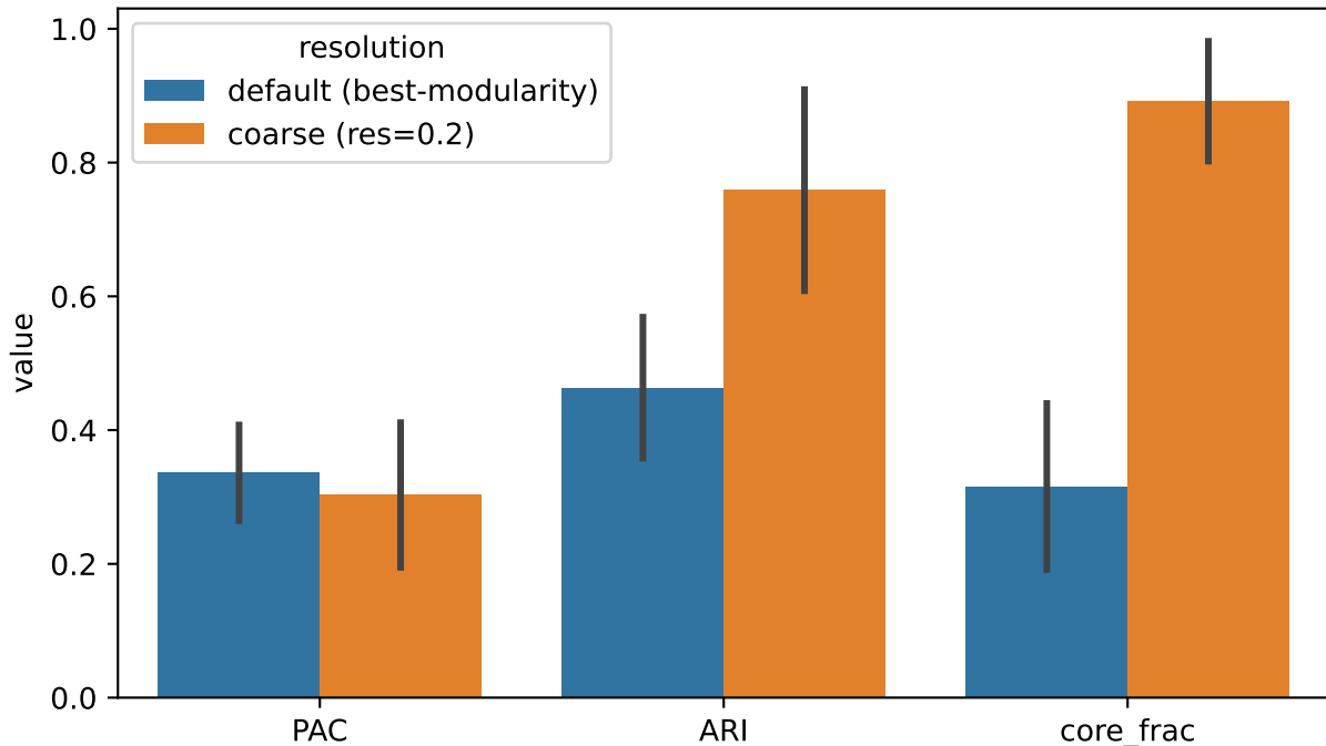
Gene-clustering resolution sensitivity (annotation regime)
