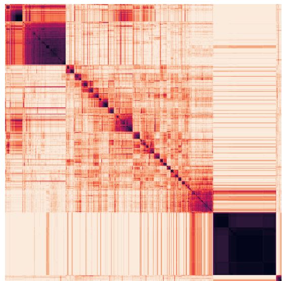
tp11 (PAC=0.34, 2000 genes)
