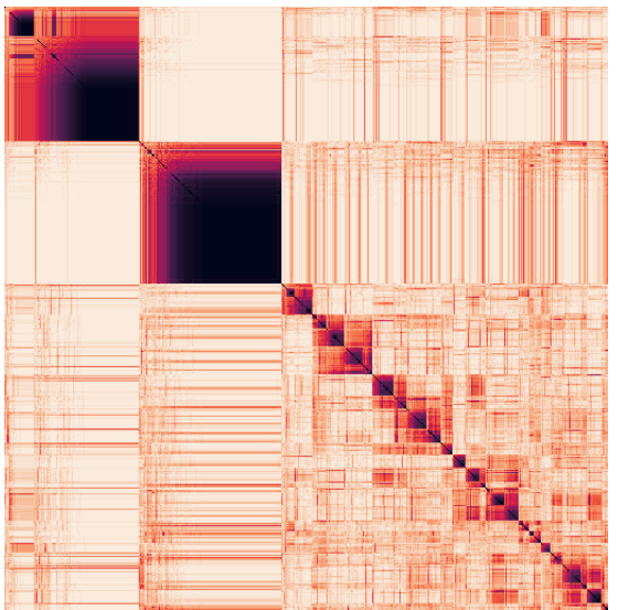
tp15 (PAC=0.30, 2000 genes)
