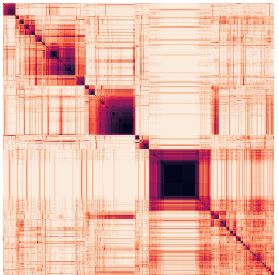
tp13 (PAC=0.35, 2000 genes)
