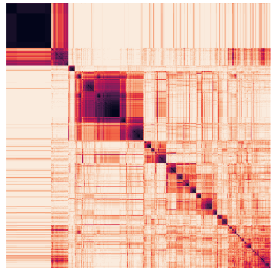
tp11 (PAC=0.33, 2000 genes)
