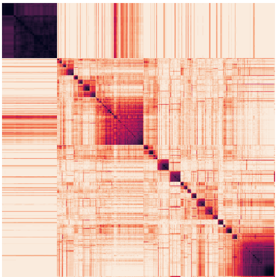
tp17 (PAC=0.31, 2000 genes)
