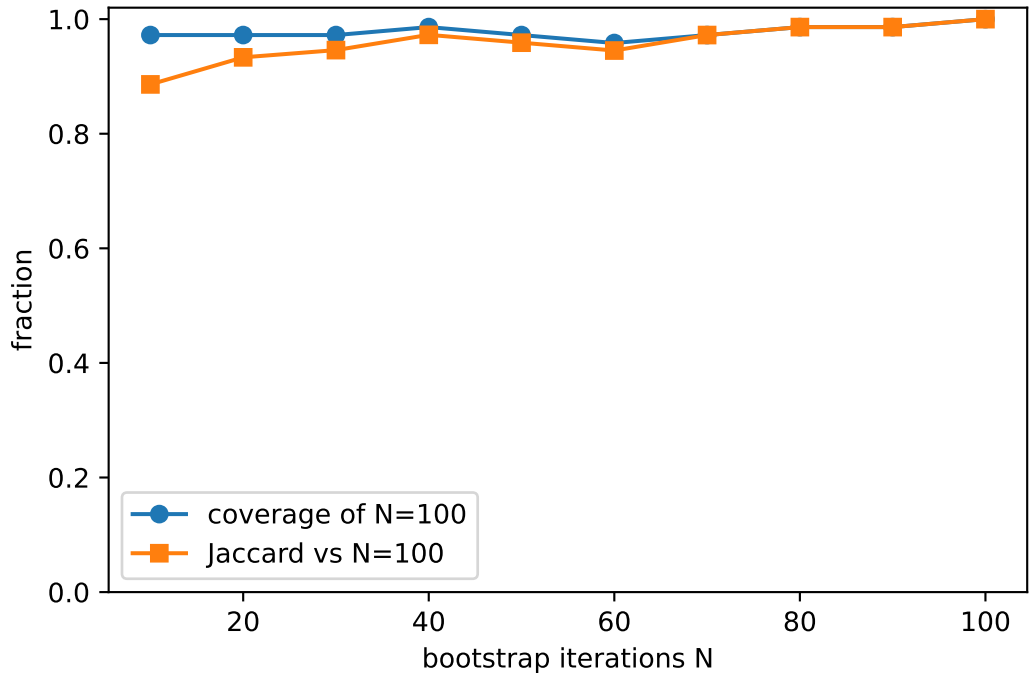
Convergence to N=100 network
