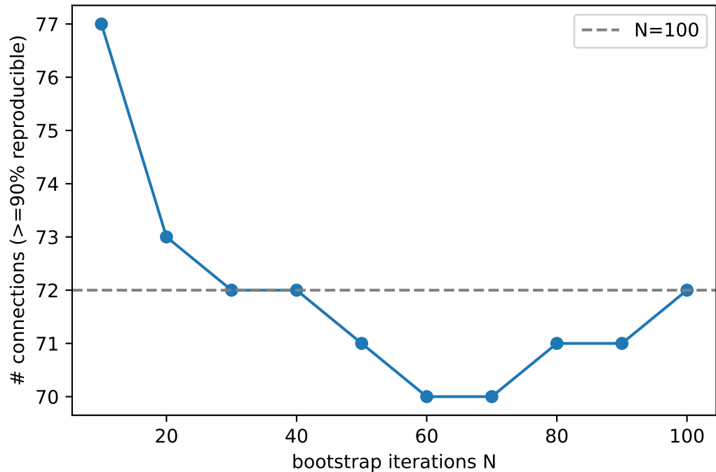
Network size vs bootstrap N
