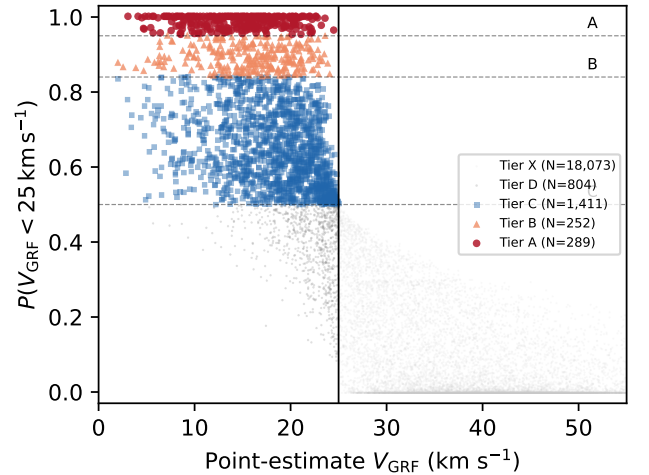
Figure 7. Velocity-threshold membership probability versus corrected point-estimate V_{grf} for the propagated Gaia DR3 candidate pool. The horizontal dashed lines mark the Tier A, Tier A+B, and Tier A+B+C probability boundaries; the vertical line marks the 25 \text{km s}^{-1} point-estimate selection boundary. The catalogue is defined by threshold probability, not by a hard point estimate alone.
