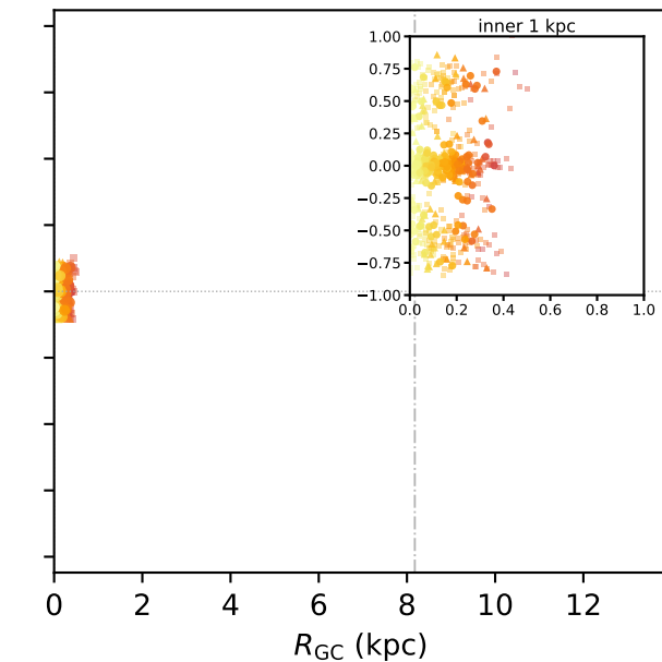
Modelled pericentres
