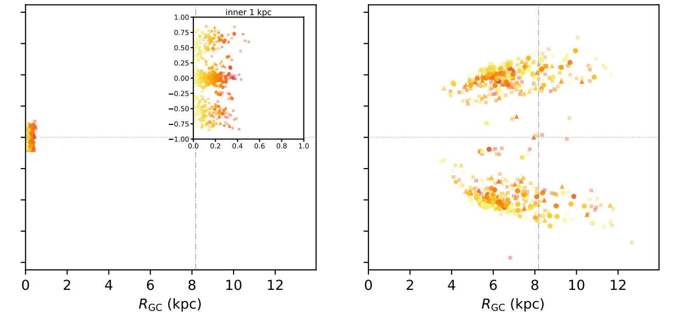
Modelled pericentres
