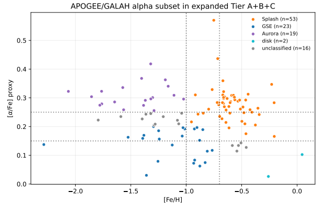
Figure 5. [\text{Mg}/\text{Fe}] (APOGEE) and [\alpha/\text{Fe}] (GALAH) vs. [\text{Fe}/\text{H}] for the \alpha -classified spectroscopic subset within Tier A+B+C ( N = 113 ). Literature-region labels are shown only as contextual comparisons and are not treated as whole-catalogue population assignments.
