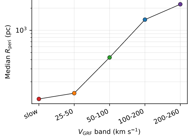
Figure 11. Median pericentre as a function of Galactic rest-frame velocity for the slow Tier A+B+C catalogue ( N = 1,835 ) and the four observability-matched control bands. The slow band sits at the small- R_{\text{peri}} end of a smooth kinematic sequence; per-band pericentre medians are reported in Table 12.
