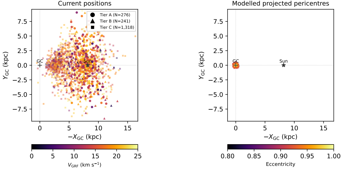
Figure 2. Face-on view of the Tier A+B+C slow catalogue ( N = 1,835 ) in the displayed -X_{GC} vs. Y_{GC} plane, so that the Galactic centre is at left and the Sun lies to the right. As in Fig. 1, the broader Tier A+B+C orbit-summary sample is shown, with marker shape separating the Tier A+B headline catalogue from the Tier C extension. Left: current Galactocentric positions, colour-coded by V_{grf} ; the catalogue is observed in a Sun-centred local volume. Right: modelled, projected pericentre passage positions in the static Hunter+2024 potential, colour-coded by orbital eccentricity and shown on the same spatial scale as the left panel. Marker shape encodes tier (circle/triangle/square = A/B/C). The shared scale makes the inner-Galaxy reach of the catalogue directly visible: all point-estimate pericentres fall inside R_{GC} < 1 kpc in this fine trajectory sampling, with a median Tier A+B+C pericentre of 112 pc.
