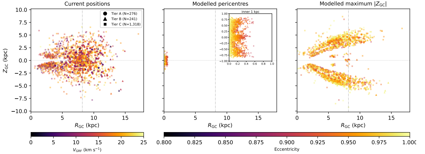
Figure 1. Edge-on orbital context for the Tier A+B+C slow catalogue ( N = 1,835 ) in R_{GC} vs. Z_{GC} . Current positions are observed coordinates, while the modelled pericentre and modelled maximum- |Z_{GC}| panels are model-derived locations in the adopted static Hunter+2024 potential. This broader Tier A+B+C sample is used for orbit-context visualisation; the Tier A+B headline catalogue is distinguished from the Tier C extension by marker shape. The panels show current positions, modelled pericentre positions, and modelled maximum- |Z_{GC}| points. Current positions are colour-coded by V_{grf} ; modelled pericentre and maximum- |Z_{GC}| positions are colour-coded by eccentricity, with the pericentre panel inset expanding the inner kiloparsec. The right panel shows the vertical envelope of the adopted model trajectories; apocentre radii are reported separately in Table 11 and Fig. 7. Marker shape encodes tier: circles (Tier A), triangles (Tier B), squares (Tier C). The vertical dot-dashed line marks R_{\odot} = 8.178 kpc and the Galactic centre is at R_{GC} = 0 . Because R_{GC} is cylindrical radius, the pericentre panel and inset show central reach, not the signed side of the Galactic centre on which each passage occurs; that azimuthal side-of-centre information is retained in the face-on view of Fig. 2.
