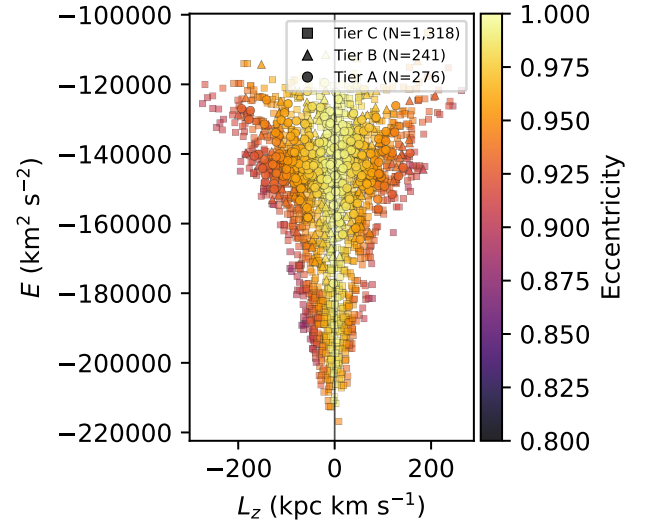
Figure 12. Tier A+B+C slow catalogue ( N = 1,835 ) in E – L_z space, colour-coded by orbital eccentricity in the static Hunter+2024 potential. Marker shape encodes tier (circle/triangle/square = A/B/C); the vertical line marks L_z = 0 and the header annotation reports the 57%/43% retrograde/prograde split. The catalogue shows a mild retrograde majority but no strong tier-by-tier retrograde climb.
