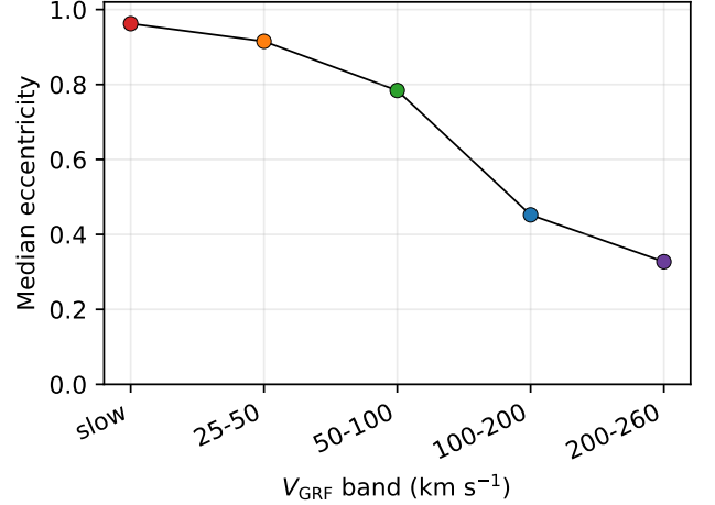
Figure 9. Median eccentricity as a function of Galactic rest-frame velocity for the Tier A+B+C slow catalogue ( N = 1,835 ) and the four observability-matched control bands. Points show the band medians and 16th–84th percentile ranges after the control bands are kernel-weighted against the slow catalogue. The monotonic decline from e \sim 1.0 at low V_{\text{grf}} to moderate eccentricity at 200–260 \text{km s}^{-1} matches the band-by-band medians in Table 12.
