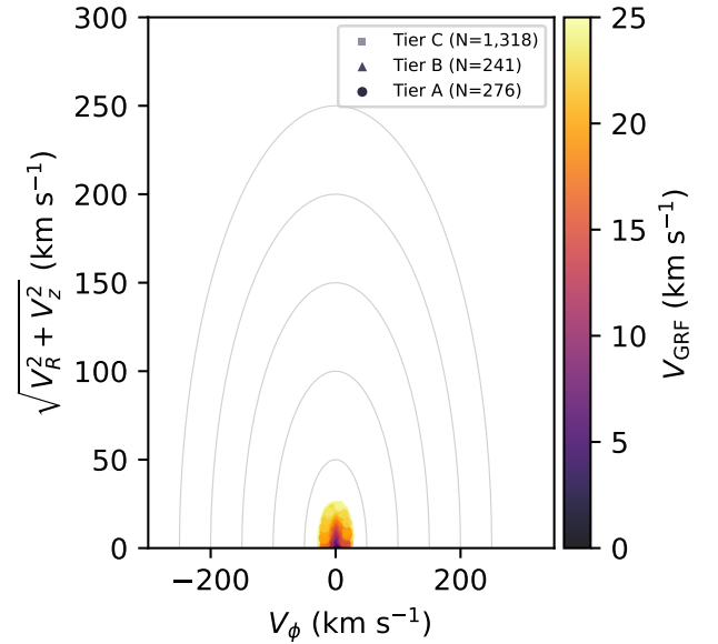
Figure 8. Toomre diagram ( V_\phi vs. \sqrt{V_R^2 + V_z^2} ) for the Tier A+B+C slow catalogue ( N = 1,835 ), colour-coded by V_{\text{grf}} . The sample is concentrated at low azimuthal velocity, far from the disc locus.
