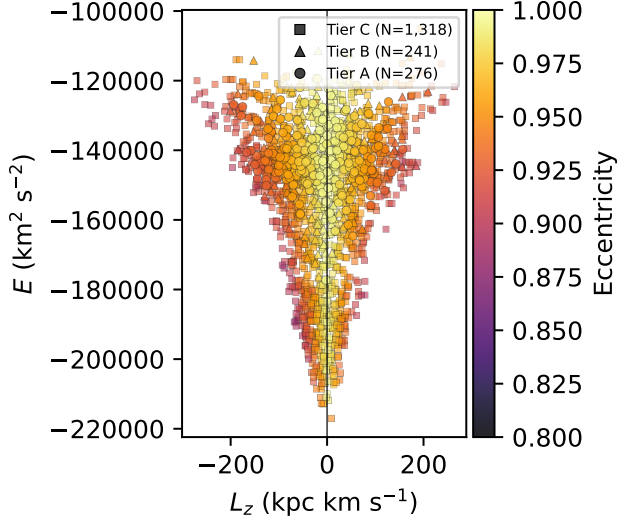
Figure 12. Tier A+B+C slow catalogue ( N = 1,835 ) in E - L_z space, colour-coded by orbital eccentricity in the static Hunter+2024 potential. Marker shape encodes tier (circle/triangle/square = A/B/C); the vertical line marks L_z = 0 .
