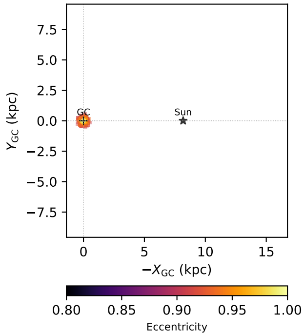
Modelled projected pericentres
