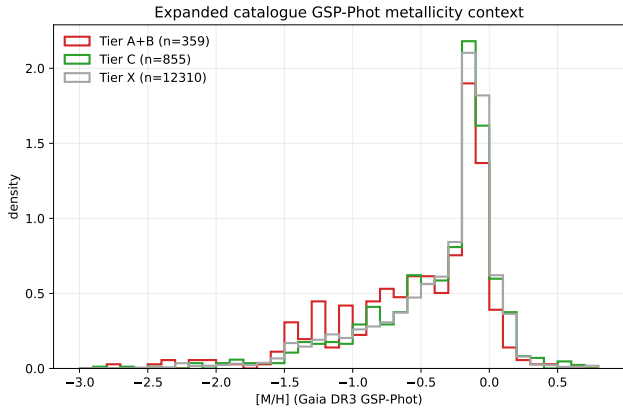
Figure 4. Gaia GSP-Phot metallicity distribution for the expanded catalogue, shown as a low-resolution contextual diagnostic. These values are not used for population-region assignment.
