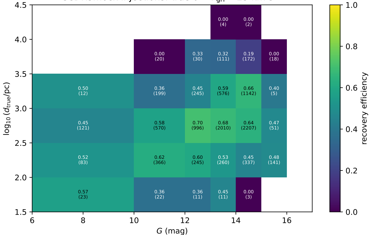
GeDR3mock injections: true 0 < V_{\text{grf}} < 25 \text{ km s}^{-1}
