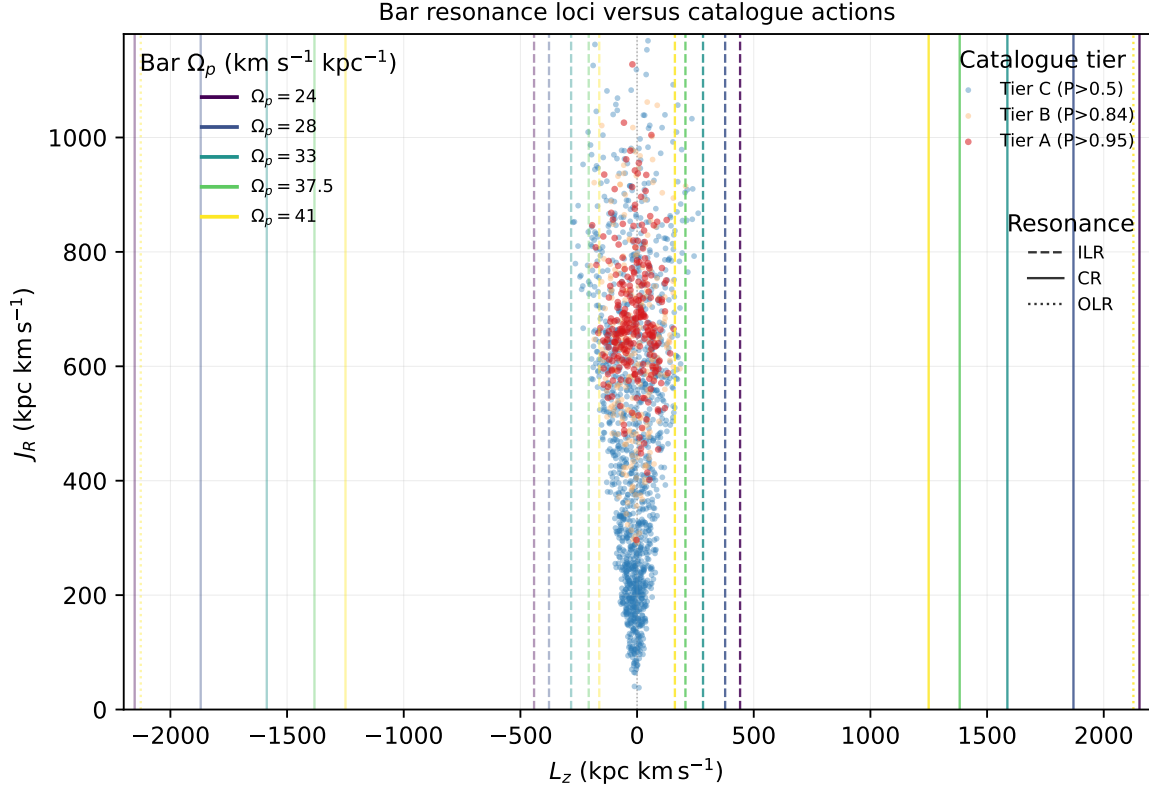
Figure 22. Bar resonance loci versus catalogue actions. Vertical lines mark the values of L_z for circular orbits at the inner Lindblad (dashed), corotation (solid), and outer Lindblad (dotted) radii in the axisymmetrised Hunter+2024 potential at each of the five bar pattern speeds in the extended grid (colour-coded). Loci at negative L_z mirror the retrograde-orbit case. Catalogue points are colour-coded by tier and use the Stäckel-fudge (L_z, J_R) values reported per star; Tier A points cluster near L_z \approx 0 at large J_R .
