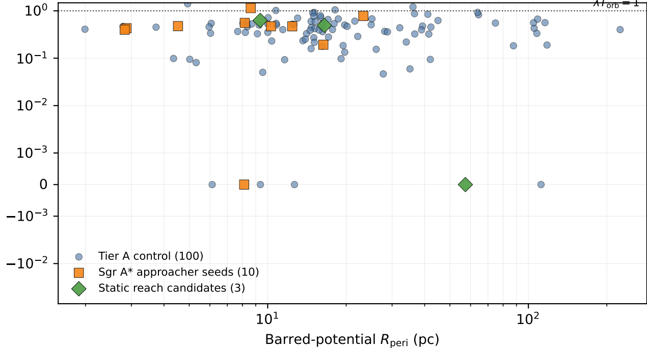
Chaos diagnostic in the default barred potential
