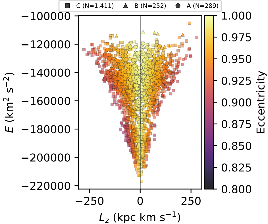
Figure 18. Tier A+B+C slow catalogue ( N = 1,952 ) in E – L_z space, colour-coded by orbital eccentricity in the static Hunter+2024 potential. Marker shape encodes tier (circle/triangle/square = A/B/C); the vertical line marks L_z = 0 .
