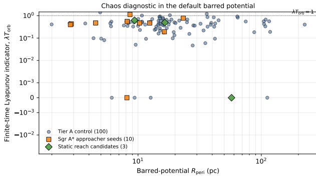
Figure 20. Finite-time Lyapunov indicator in the default barred Hunter/Sormani potential at \Omega_p = 37.5 \text{ km s}^{-1} \text{ kpc}^{-1} , plotted against the barred-potential cylindrical pericentre. The horizontal dotted line marks \lambda T_{\text{orb}} = 1 , the order-unity level used by Agama as a practical strongly chaotic threshold.
