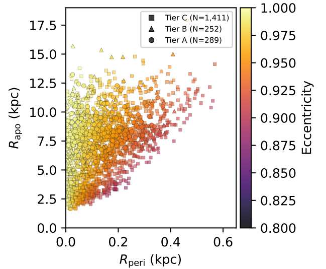
Figure 13. Pericentre vs. apocentre for the Tier A+B+C slow catalogue ( N = 1,952 ), colour-coded by eccentricity, in the static Hunter+2024 potential. Axis ranges are set to where the adopted-model point-estimate integrations place the data: all 1,952 stars have R_{\text{peri}} < 1 kpc and nearly all have R_{\text{apo}} < 18 kpc. The long-apocentre inner-reach sensitivity test (§4.4) is reported in the text and in Table 20, not on this panel.
