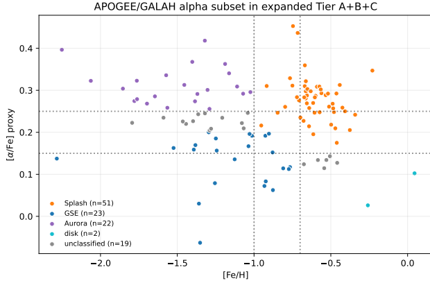
Figure 10. [\text{Mg}/\text{Fe}] (APOGEE) and [\alpha/\text{Fe}] (GALAH) vs. [\text{Fe}/\text{H}] for the \alpha -classified spectroscopic subset within Tier A+B+C ( N = 117 ). Literature-region labels are shown only as contextual comparisons and are not treated as whole-catalogue population assignments.
