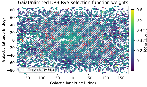
Figure 11. GaiaUnlimited DR3-RVS (Castro-Ginard et al. 2023) selection-function weight map for the expanded candidate pool, queried in the same (G_{RVS}, BP-RP, l, b) convention as the pipeline. Cell colour is the per-pixel mean \log_{10}(1/S_{RVS}) ; red points mark the Tier A+B primary catalogue ( N = 541 ). White hatching flags pixels in which \geq 50\% of catalogue stars sit in GaiaUnlimited cells with parent count n < 10 , the regime where the \text{Beta}(k+1, n-k+1) posterior is prior-dominated. The Tier A+B locus overlaps the hatched region substantially, consistent with the f_{n<10} = 83.2\% of stars and 88.7\% of \sum 1/S_{RVS} reported in Table 15.
