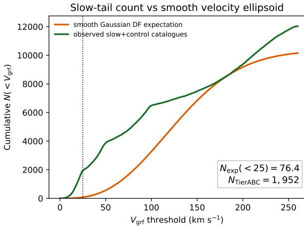
Figure 8. Observed cumulative slow-tail count compared with an illustrative smooth trivariate-Gaussian velocity ellipsoid fit to the matched-control catalogues and normalised over 25\text{--}260 \text{ km s}^{-1} . The observed/predicted ratio below the adopted 25 \text{ km s}^{-1} selection threshold motivates treating the low- V_{\text{grf}} catalogue as a low-velocity tail in the observed Gaia DR3 6D distribution, not as evidence for a physical discontinuity at exactly 25 \text{ km s}^{-1} or as a complete Milky Way forward model. This single-ellipsoid baseline gives the largest of the tested smooth-continuation observed/predicted ratios; a BIC Gaussian mixture and a cross-validated kernel density give 7.4\times and 11\times respectively (Table 12). Absolute pipeline normalisation is provided separately by the controlled injection-recovery test of Section 4.7.
