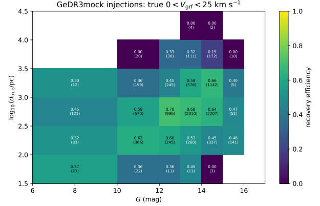
Figure 19. End-to-end recovery efficiency for the true 0 < V_{\text{grf}} < 25 \text{ km s}^{-1} GeDR3mock injections as a function of apparent G magnitude and true distance. Each cell reports the recovered fraction, with the number of injected stars in parentheses. The denominator is the post-observability injected sample; the numerator requires the RVS-availability draw, \varpi_{\text{corr}}/\sigma_{\varpi} > 5 , and Tier A+B+C recovery in the fixed 500-realisation diagnostic pass.
