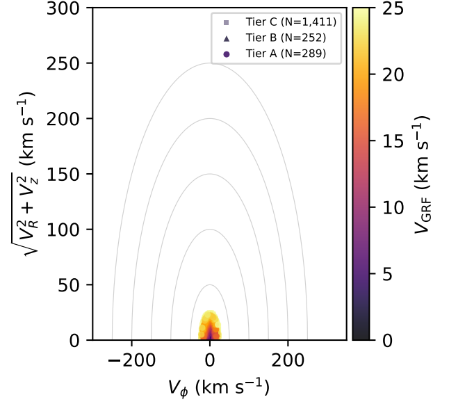
Figure 14. Toomre diagram ( V_\phi vs. \sqrt{V_R^2 + V_z^2} ) for the Tier A+B+C slow catalogue ( N = 1,952 ), colour-coded by V_{\text{grf}} . The sample is concentrated at low azimuthal velocity, far from the disc locus.
