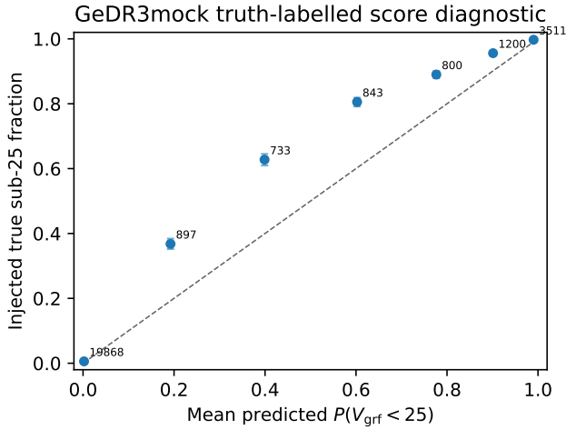
Figure 3. Truth-labelled GeDR3mock probability-score diagnostic for pipeline-input mock stars. Points bin injected stars by their predicted P(V_{\text{grf}} < 25 \text{ km s}^{-1}) and compare with the fraction whose injected true V_{\text{grf}} is below 25 \text{ km s}^{-1} . Numbers annotate the stars per bin. The mock prior is balanced across injected velocity bins, so the figure checks score monotonicity and high-probability behaviour rather than the population-prior calibration of the observed catalogue.
