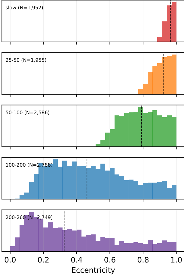
Figure 16. Eccentricity histograms for each of the five GRF velocity bands, stacked vertically. The slow Tier A+B+C band ( N = 1,952 ) shows the extreme near-unity peak; the eccentricity distribution broadens monotonically through the four control bands toward 200–260 \text{km s}^{-1} .
