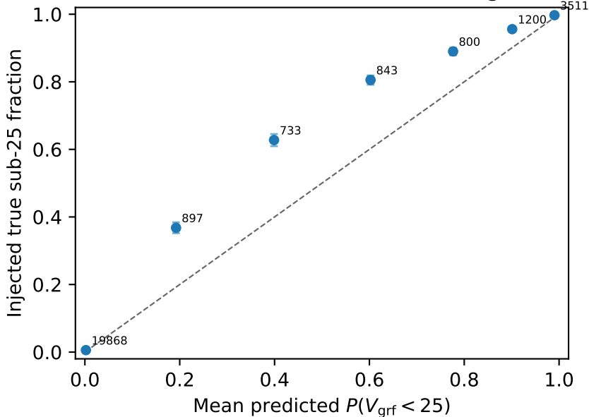
GeDR3mock truth-labelled score diagnostic
