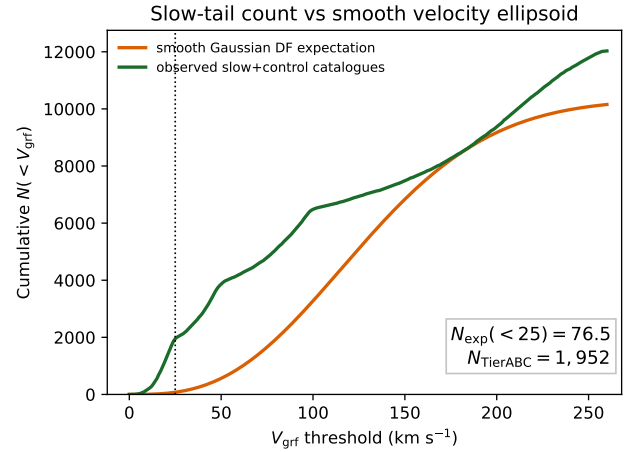
Figure 7. Observed cumulative slow-tail count compared with a smooth trivariate-Gaussian velocity ellipsoid fit to the matched-control catalogues and normalised over 25\text{--}260 \text{ km s}^{-1} . The excess below the adopted 25 \text{ km s}^{-1} selection threshold motivates treating the low- V_{\text{grf}} catalogue as a genuine low-velocity excess in the observed Gaia DR3 6D distribution, not as evidence for a physical discontinuity at exactly 25 \text{ km s}^{-1} . This single-ellipsoid baseline gives the largest of the smooth-null excess factors; a BIC Gaussian mixture and a cross-validated kernel density give 7.4\times and 11\times respectively (Table 10). Absolute pipeline normalisation is provided separately by the controlled injection-recovery test of Section 4.7.
