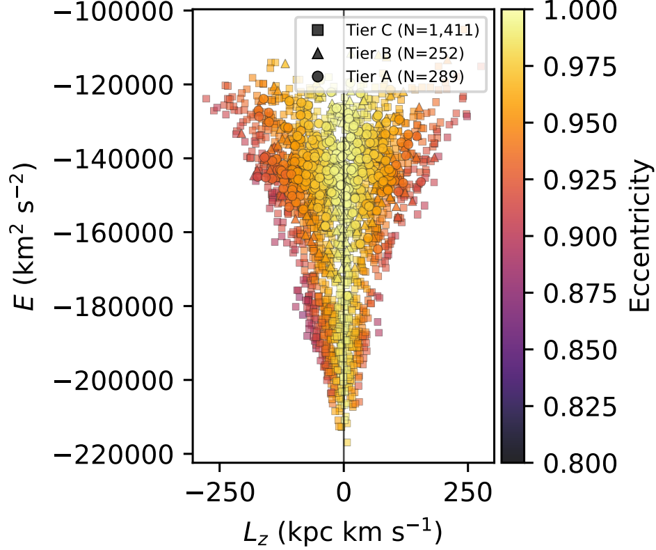
Figure 17. Tier A+B+C slow catalogue ( N = 1,952 ) in E - L_z space, colour-coded by orbital eccentricity in the static Hunter+2024 potential. Marker shape encodes tier (circle/triangle/square = A/B/C); the vertical line marks L_z = 0 .
