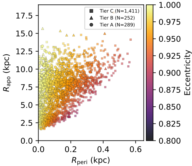
Figure 12. Pericentre vs. apocentre for the Tier A+B+C slow catalogue ( N = 1,952 ), colour-coded by eccentricity, in the static Hunter+2024 potential. Axis ranges are set to where the adopted-model point-estimate integrations place the data: all 1,952 stars have R_{\text{peri}} < 1 kpc and nearly all have R_{\text{apo}} < 18 kpc. The long-apocentre inner-reach sensitivity test (§4.4) is reported in the text and in Table 19, not on this panel.
