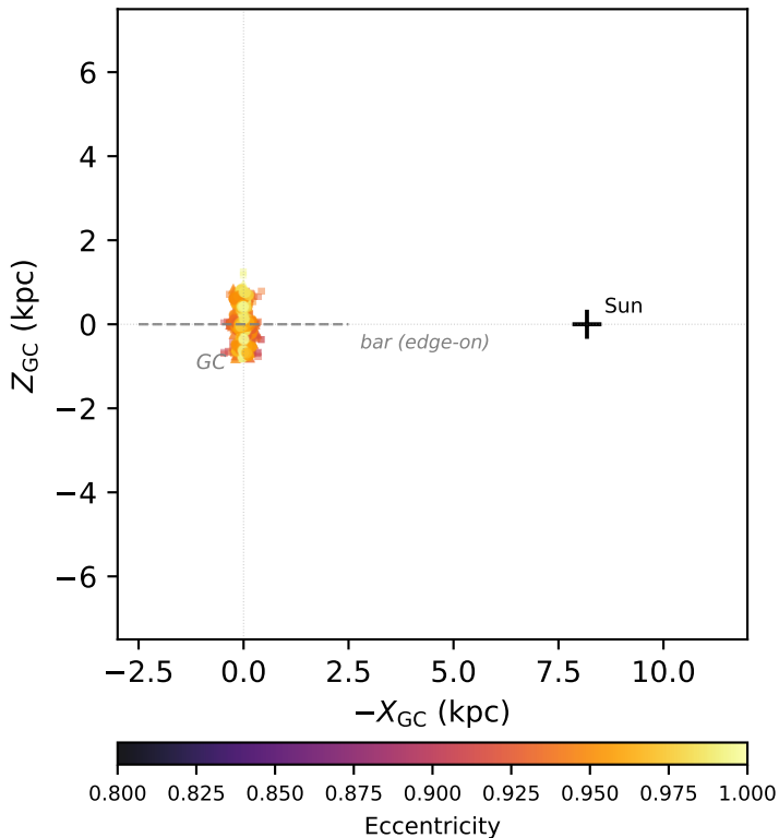
Fig 1va working version -- fixed 15 x 15 kpc axes (not final)
