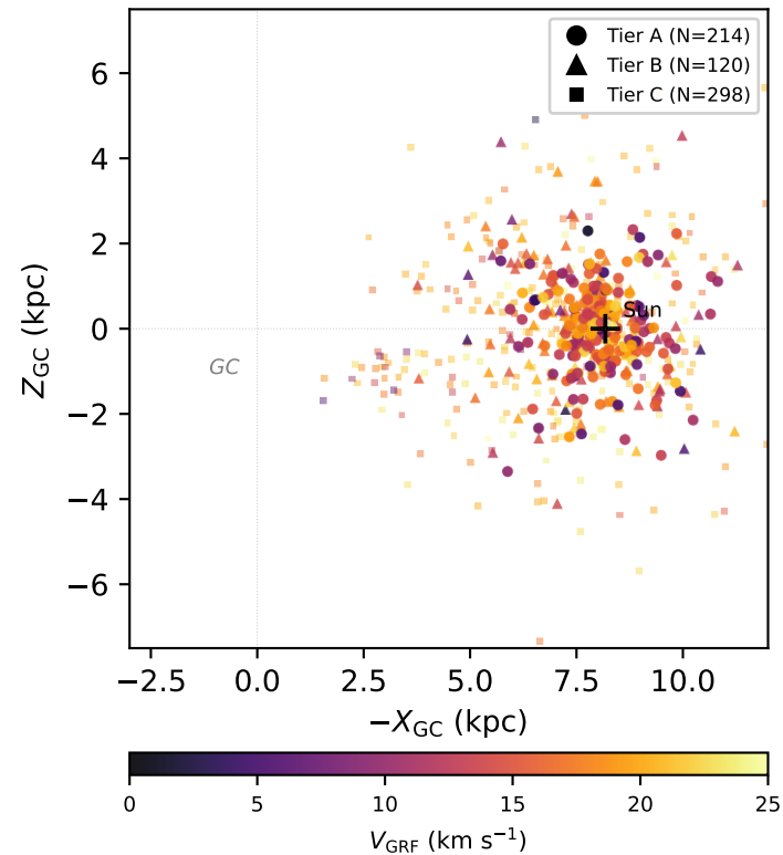
Fig 1va working version -- fixed 15 x 15 kpc axes (not final)
