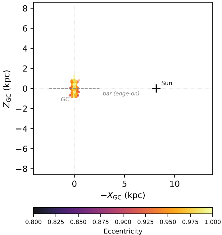
Pericentre positions
