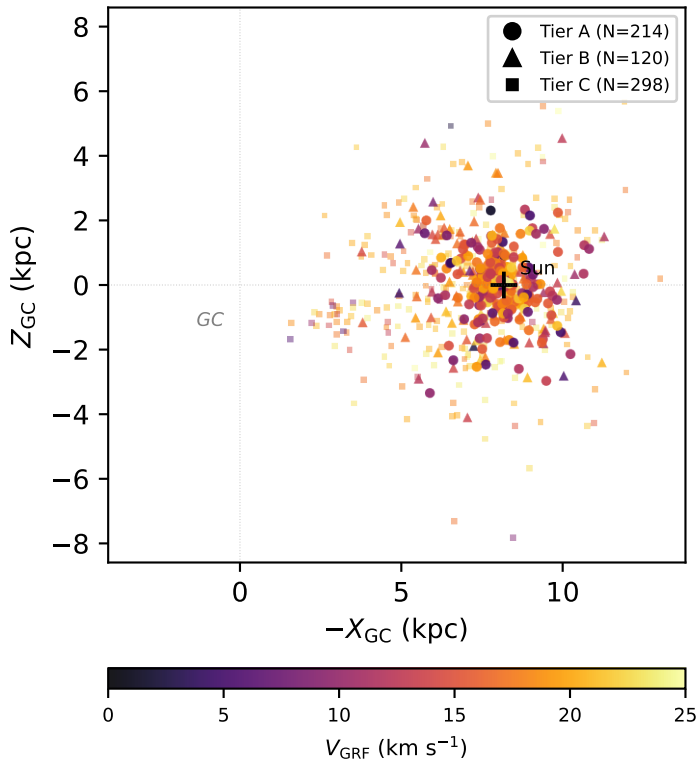
Current positions
