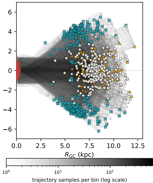
Side view: meridional orbit density
