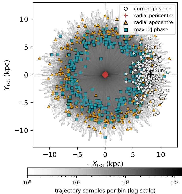
Top-down view: same orbit samples
