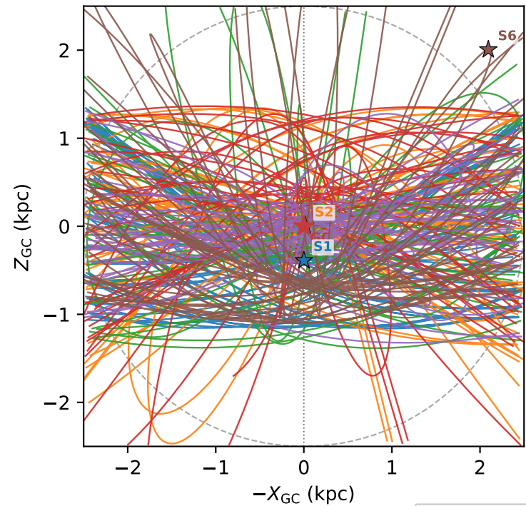
Inner 2.5 kpc: side view
