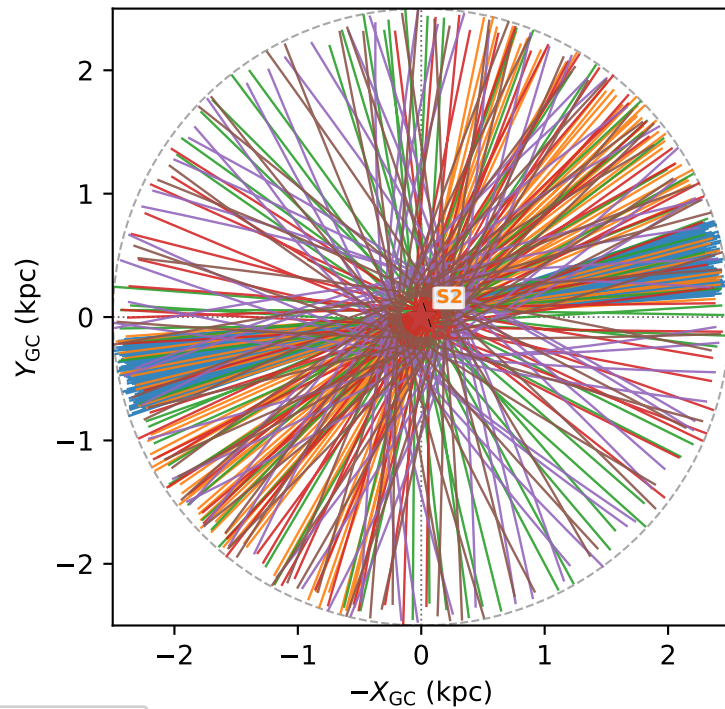
Inner 2.5 kpc: top-down view
