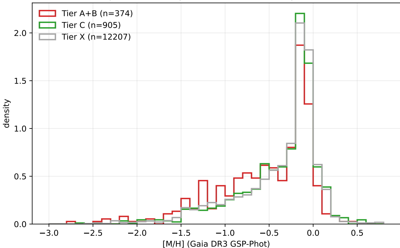
Expanded catalogue GSP-Phot metallicity context
