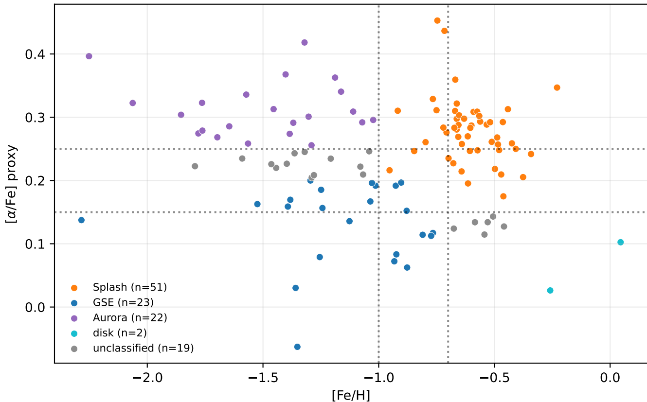
APOGEE/GALAH alpha subset in expanded Tier A+B+C
