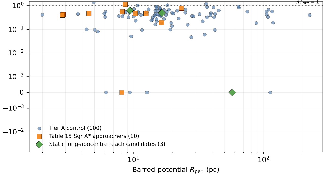
WP-5 chaos diagnostic in the default barred potential
