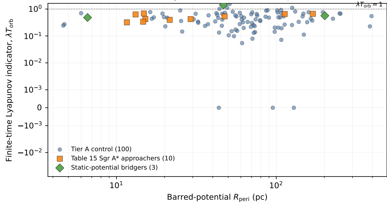
WP-5 chaos diagnostic in the default barred potential
