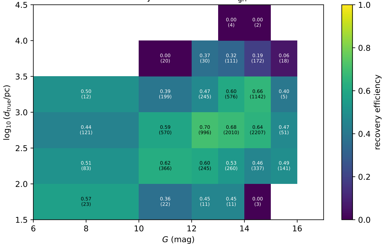
WP-7 GeDR3mock injections: true 0 < V_{\text{grf}} < 25 \text{ km s}^{-1}
