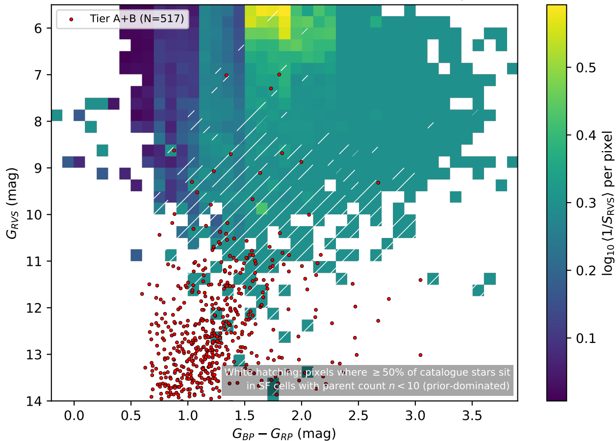
GaiaUnlimited DR3-RVS selection-function map
