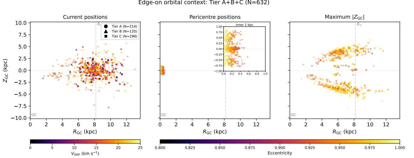
Figure 1. Edge-on orbital context for the Tier A+B+C slow catalogue ( N = 632 ) in R_{GC} vs. Z_{GC} . This broader Tier A+B+C sample is used for orbit-context visualisation; the Tier A+B headline catalogue is distinguished from the Tier C extension by marker shape. The panels show current positions, pericentre positions, and the maximum- |Z_{GC}| points in the adopted static Hunter+2024 potential. Current positions are colour-coded by V_{grf} ; pericentre and maximum- |Z_{GC}| positions are colour-coded by eccentricity, with the pericentre panel inset expanding the inner kiloparsec. The right panel shows the vertical envelope of the adopted model trajectories; apocentre radii are reported separately in Table 11 and Fig. 8. Marker shape encodes tier: circles (Tier A), triangles (Tier B), squares (Tier C). The vertical dot-dashed line marks R_{\odot} = 8.178 kpc and the Galactic centre is at R_{GC} = 0 . Because R_{GC} is cylindrical radius, the pericentre panel and inset show central reach, not the signed side of the Galactic centre on which each passage occurs; that azimuthal side-of-centre information is retained in the face-on view of Fig. 2.
