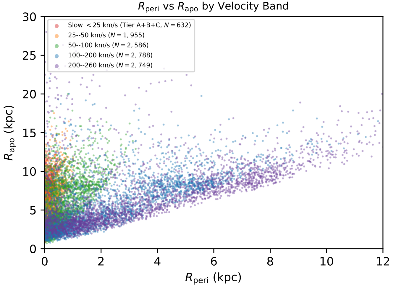
Figure 12. Pericentre vs. apocentre for all five velocity bands (slow Tier A+B+C, N = 632 , plus four observability-matched control bands), colour-coded by band. The slow band sits at the small- R_{\text{peri}} end of a smooth kinematic sequence; per-band pericentre medians are reported in Table 12.
