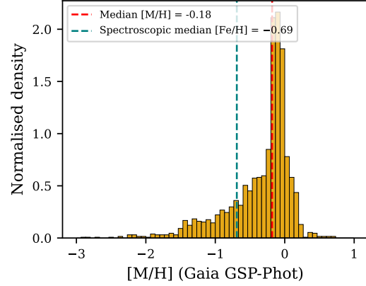
Figure 4. Gaia GSP-Phot metallicity distribution for the 1,963 stars with [\text{M}/\text{H}] , with the spectroscopic median [\text{Fe}/\text{H}] reference line. See Figure 5 for the same sample re-derived from the Zhang et al. (2023) XP catalogue.
