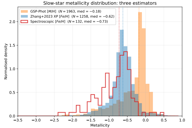
Figure 5. Three independent metallicity estimators for the slow-star sample: Gaia GSP-Phot [\text{M}/\text{H}] (orange), Zhang et al. (2023) XP-spectra [\text{Fe}/\text{H}] restricted to the highest-quality flag (blue), and the unified spectroscopic [\text{Fe}/\text{H}] reference sample (red outline). The XP estimator agrees with the spectroscopic median at [\text{Fe}/\text{H}] \approx -0.7 ; GSP-Phot is biased toward solar by \sim 0.34 dex, consistent with the documented GSP-Phot systematic for metal-poor giants (Andrae et al. 2023). We therefore do not use GSP-Phot metallicities for population assignment.
