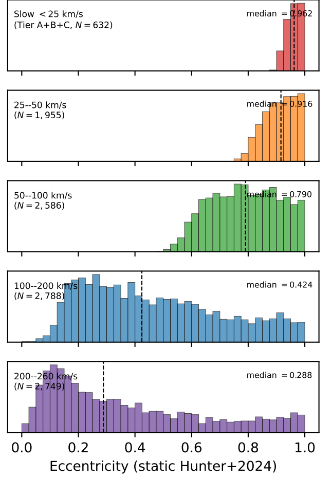
Figure 11. Eccentricity histograms for each of the five GRF velocity bands, stacked vertically. The slow Tier A+B+C band ( N = 632 ) shows the extreme near-unity peak; the eccentricity distribution broadens monotonically through the four control bands toward 200\text{--}260\text{ km s}^{-1} .
