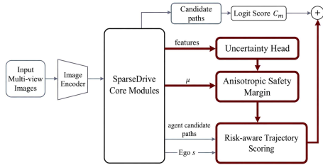
Fig. 1 Pipeline of the proposed uncertainty-aware planning decoder
