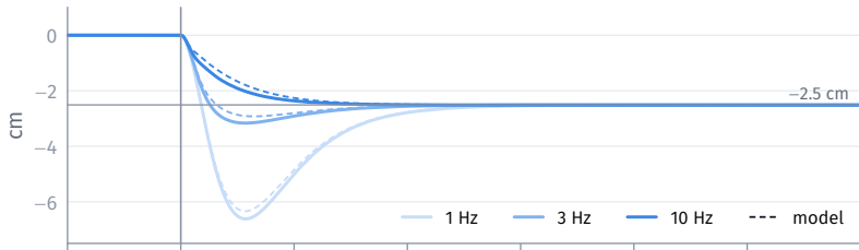
Payload in calm air, no sensor noise: altitude error by filter C(s)
