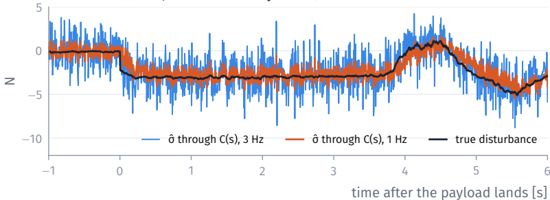
The lesson (wind, 0.1 m/s velocity noise): what the estimator sees
