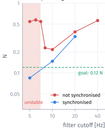
Motor jitter against the filter
