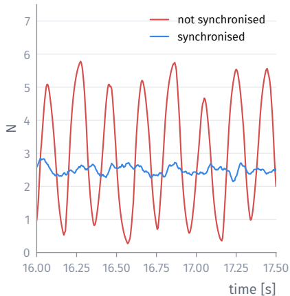
Motor 1, both filters at 5 Hz
