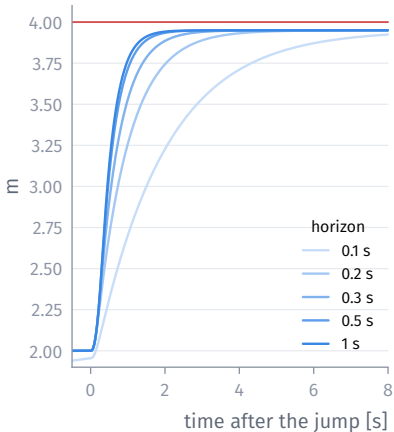
Altitude, by horizon
