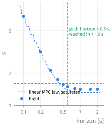
Time to reach the set-point
