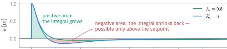
Error after a 1 m setpoint step at t = 10 s
