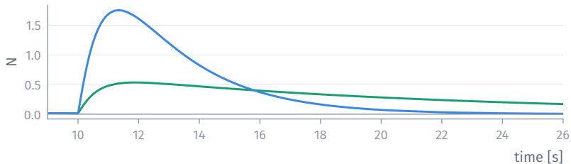
The integral term must end where it started: the load has not changed
