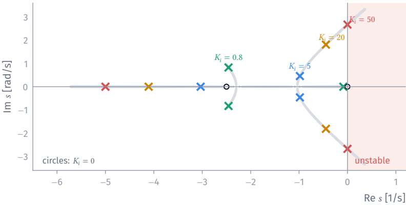
Where the three poles go as the integral gain grows ( m = 1.4 \text{ kg} )
