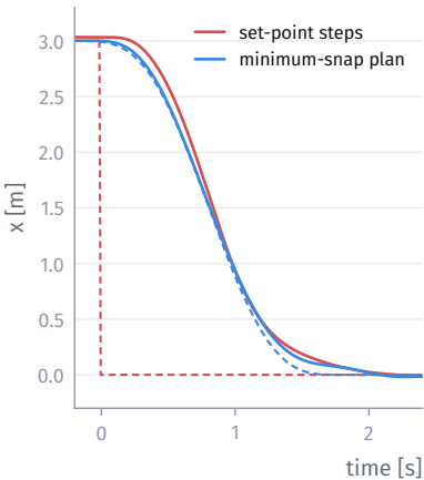
One side: set-point (dashed) and drone
