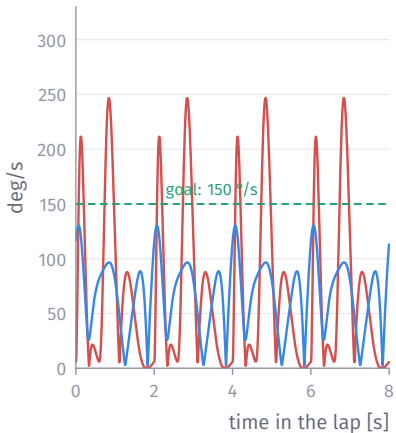
Body rate over the lap
