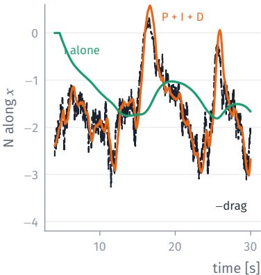
L2: the force against the wind
