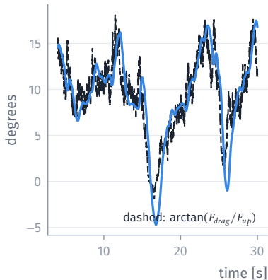
L3: the pitch angle
