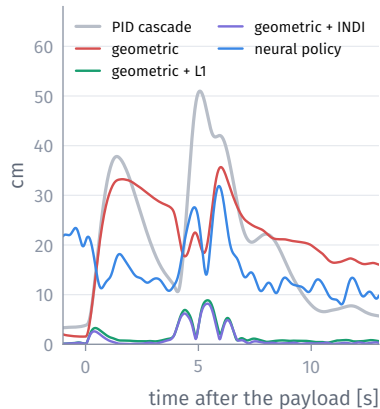
Payload: +300 g at 12 s
