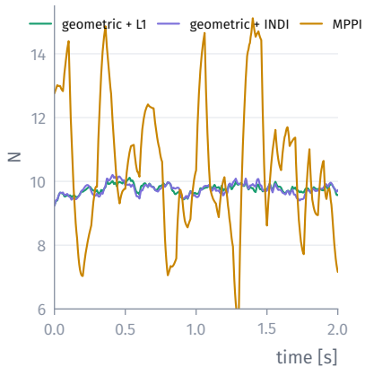
Noisy sensors: total thrust, 2 s
