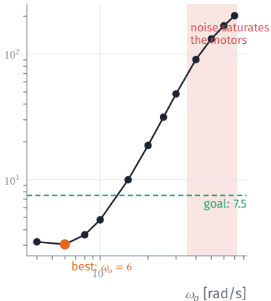
Score = error [cm] + 10 × jitter [N]
