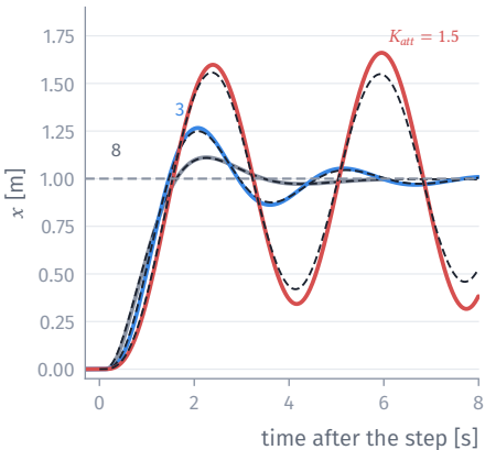
A 1 m step with softer attitude loops
