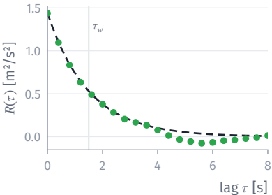
Autocorrelation
