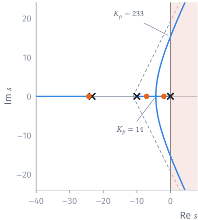
K_p grows, K_d = 7
