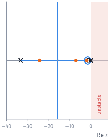
K_p and K_d grow, ratio 10 : 7
